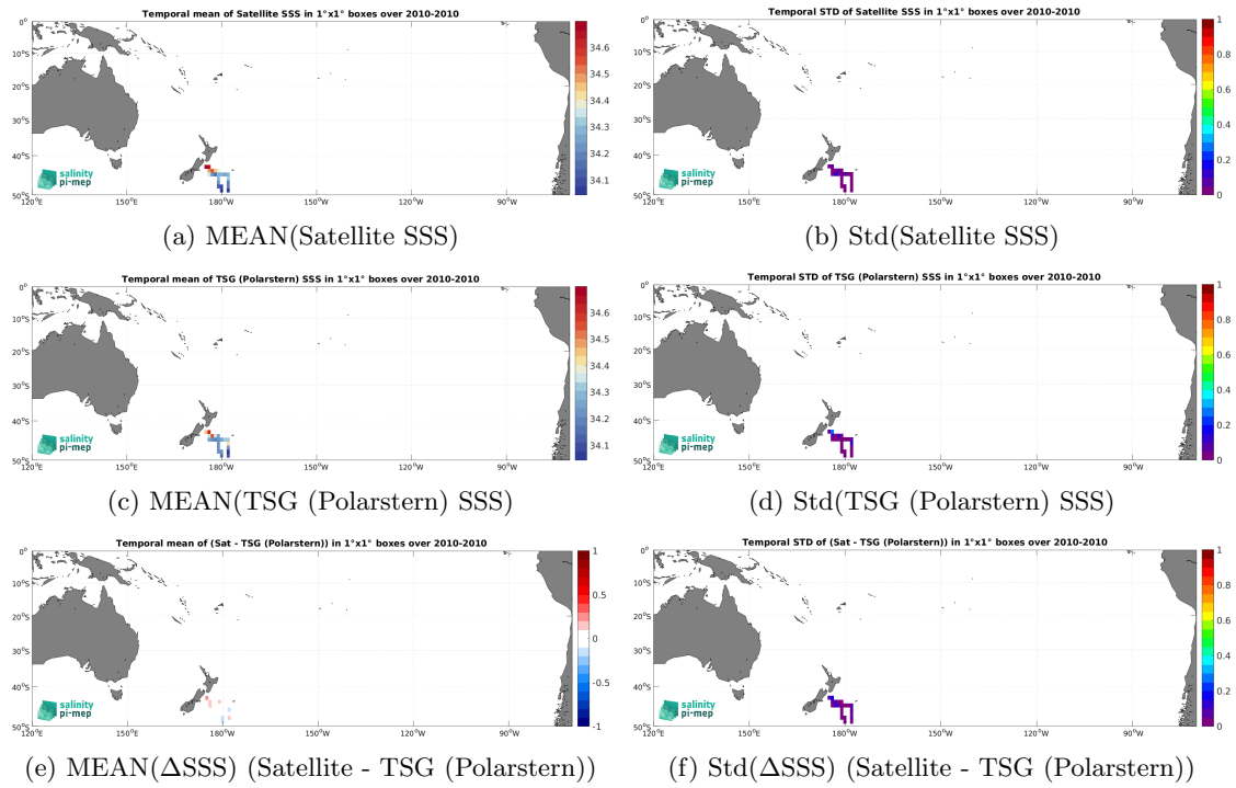
Figure 7: Temporal mean (left) and Std (right) of SSS from CCI SSS L4 Merged-OI v4.41 - 7-day running (ESA) (top), TSG (Polarstern) (middle), and of \Delta SSS (Satellite - TSG (Polarstern)). Only match-up pairs are used to generate these maps.
