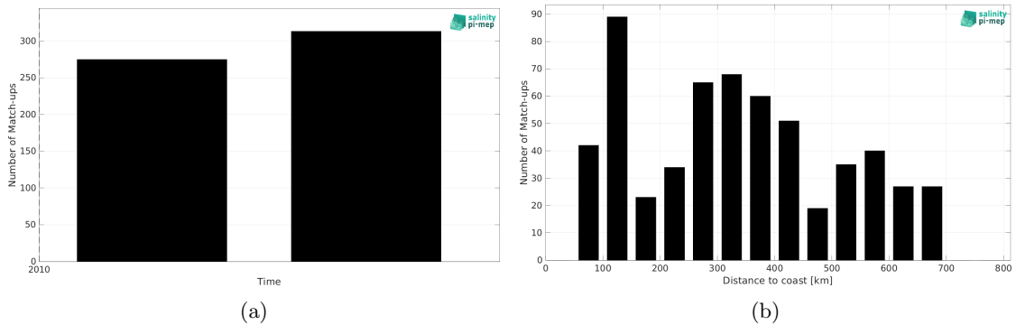
Figure 2: Number of match-ups between TSG (Polarstern) and CCI SSS L4 Merged-OI v4.41 - 7-day running (ESA) SSS as a function of time (a) and as function of the distance to coast (b) over the South Pacific Ocean Pi-MEP region and for the full satellite product period.
