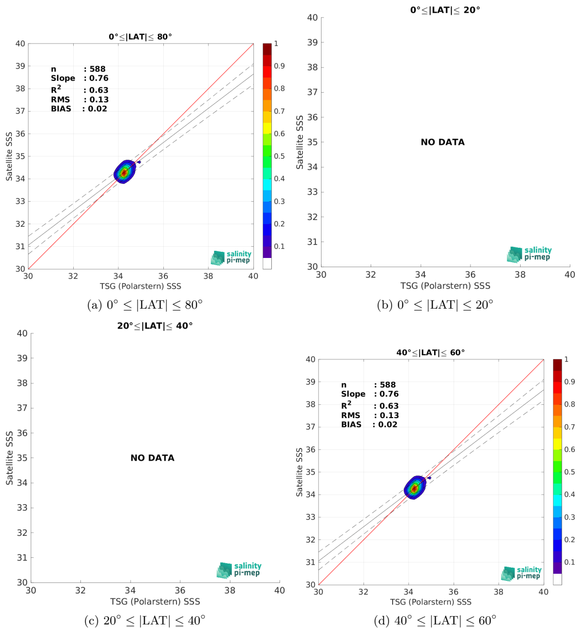
Figure 10: Contour maps of the concentration of CCI SSS L4 Merged-OI v4.41 - 7-day running (ESA) SSS (y-axis) versus TSG (Polarstern) SSS (x-axis) at match-up pairs for different latitude bands. For each plot, the red line shows x=y . The black thin and dashed lines indicate a linear fit through the data cloud and the \pm 95\% confidence levels, respectively. The number match-up pairs n , the slope and R^2 coefficient of the linear fit, the root mean square (RMS) and the mean bias between satellite and in situ data are indicated for each latitude band in each plots.
