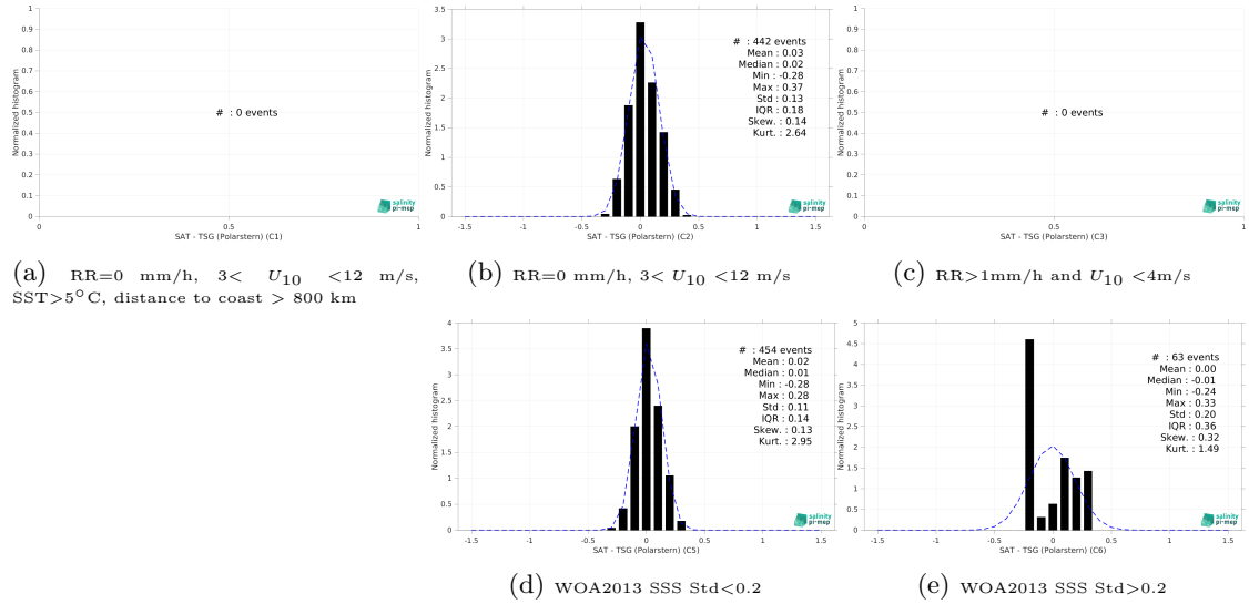
Figure 15: Normalized histogram of \Delta SSS (CCI SSS L4 Merged-OI v4.41 - 7-day running (ESA) - TSG (Polarstern)) for 5 different subdatasets corresponding to: RR=0 mm/h, 3 < U_{10} < 12 m/s, SST > 5°C, distance to coast > 800 km (a), RR=0 mm/h, 3 < U_{10} < 12 m/s (b), RR > 1mm/h and U_{10} < 4 m/s (c), WOA2013 SSS Std < 0.2 (d), WOA2013 SSS Std > 0.2 (e).
