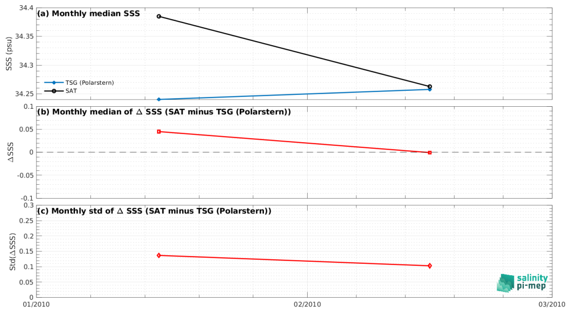
Figure 8: Time series of the monthly median SSS (top), median of \Delta SSS (Satellite - TSG (Polarstern)) and Std of \Delta SSS (Satellite - TSG (Polarstern)) over the South Pacific Ocean Pi-MEP region considering all match-ups collected by the Pi-MEP.
