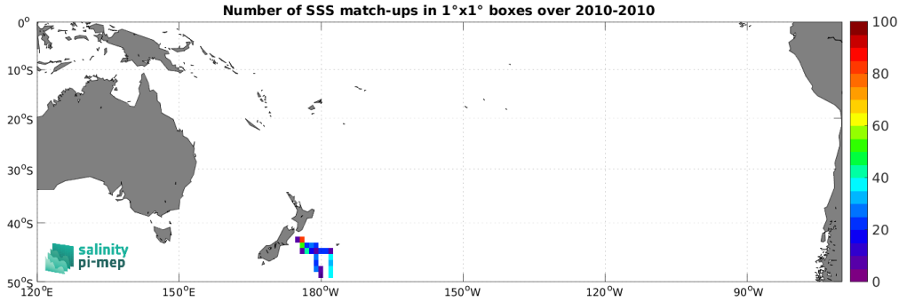
Figure 5: Number of SSS match-ups between TSG (Polarstern) SSS and the CCI SSS L4 Merged-OI v4.41 - 7-day running (ESA) SSS product for the South Pacific Ocean Pi-MEP region over 1^\circ \times 1^\circ boxes and for the full satellite product period.
