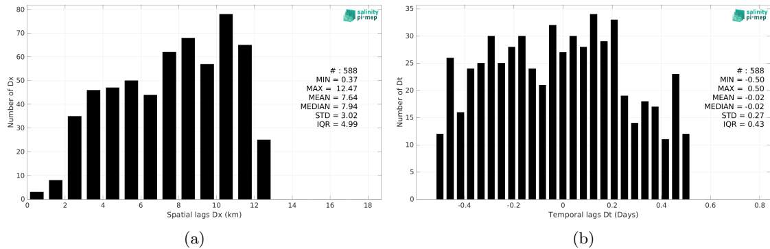
Figure 6: Histograms of the spatial (a) and temporal (b) lags between the location/time of the TSG (Polarstern) measurement and the date of the corresponding CCI SSS L4 Merged-OI v4.41 - 7-day running (ESA) SSS pixel.
