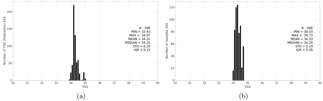
Figure 3: Histograms of SSS from TSG (Polarstern) (a) and CCI SSS L4 Merged-OI v4.41 - 7-day running (ESA) (b) considering all match-up pairs per bins of 0.1 over the South Pacific Ocean Pi-MEP region and for the full satellite product period.
