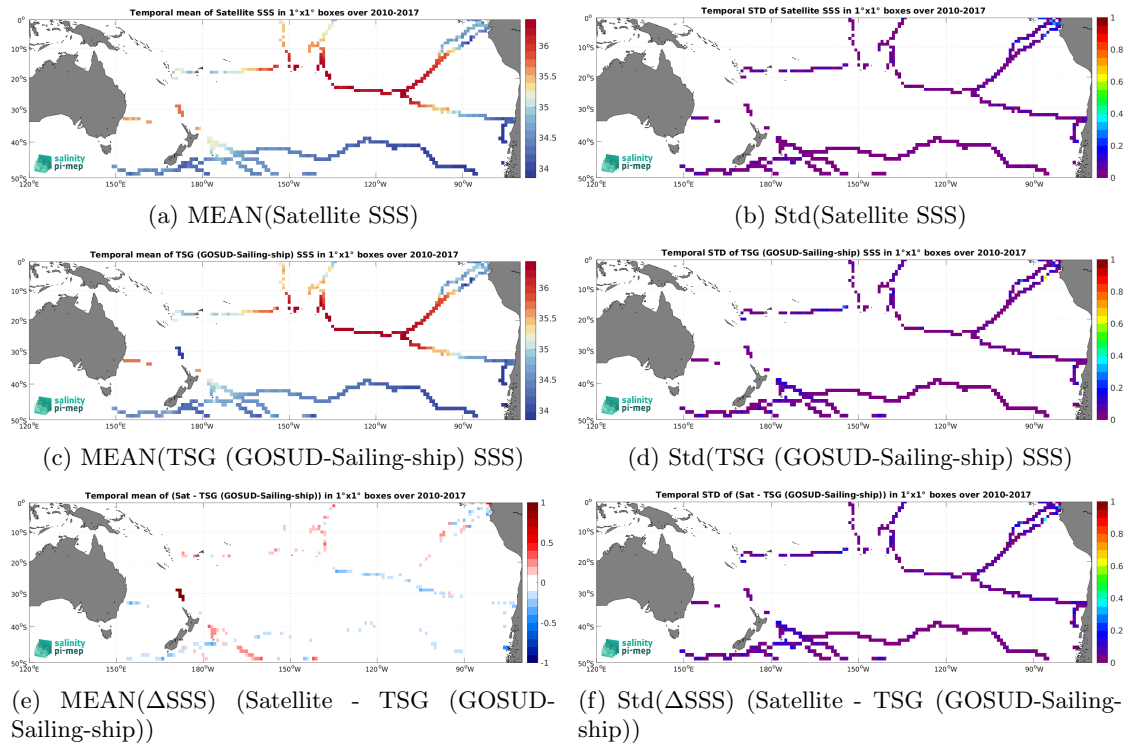
Figure 7: Temporal mean (left) and Std (right) of SSS from CCI SSS L4 Merged-OI v4.41 - 7-day running (ESA) (top), TSG (GOSUD-Sailing-ship) (middle), and of \Delta SSS (Satellite - TSG (GOSUD-Sailing-ship)). Only match-up pairs are used to generate these maps.
