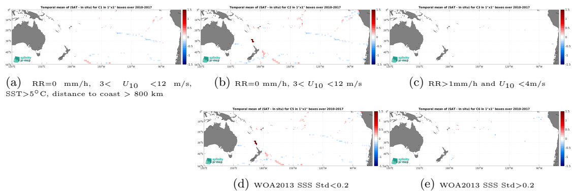
Figure 14: Temporal mean gridded over spatial boxes of size 1^\circ \times 1^\circ of \Delta SSS (CCI SSS L4 Merged-OI v4.41 - 7-day running (ESA) - TSG (GOSUD-Sailing-ship)) for 5 different subdatasets corresponding to:RR=0 mm/h, 3 < U_{10} < 12 m/s, SST >5^\circ C, distance to coast > 800 km (a), RR=0 mm/h, 3 < U_{10} < 12 m/s (b), RR >1 mm/h and U_{10} < 4 m/s (c), WOA2013 SSS Std <0.2 (d), WOA2013 SSS Std >0.2 (e).
