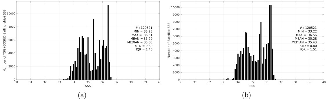
Figure 3: Histograms of SSS from TSG (GOSUD-Sailing-ship) (a) and CCI SSS L4 Merged-OI v4.41 - 7-day running (ESA) (b) considering all match-up pairs per bins of 0.1 over the South Pacific Ocean Pi-MEP region and for the full satellite product period.
