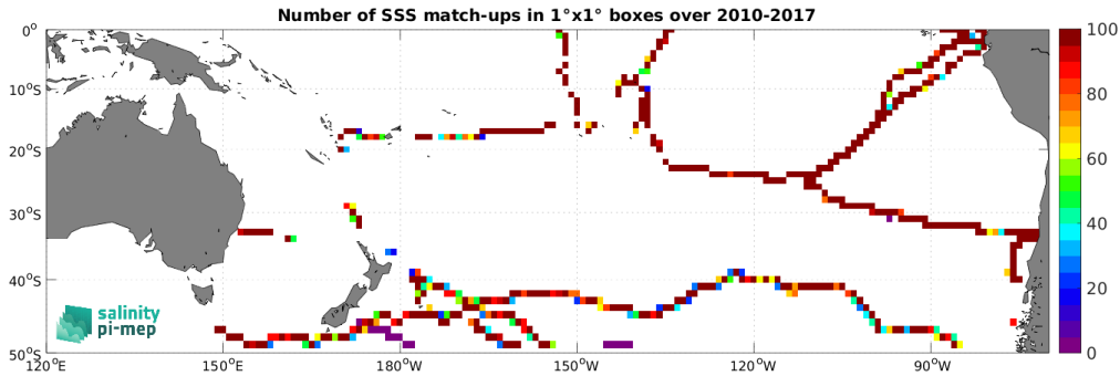
Figure 5: Number of SSS match-ups between TSG (GOSUD-Sailing-ship) SSS and the CCI SSS L4 Merged-OI v4.41 - 7-day running (ESA) SSS product for the South Pacific Ocean Pi-MEP region over 1^\circ \times 1^\circ boxes and for the full satellite product period.
