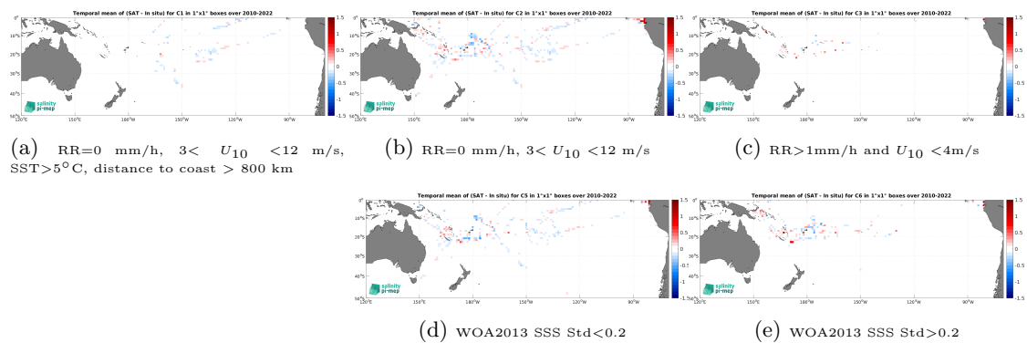
Figure 14: Temporal mean gridded over spatial boxes of size 1^\circ \times 1^\circ of \Delta SSS (CCI SSS L4 Merged-OI v4.41 - 7-day running (ESA) - TSG (GOSUD-Research-vessel)) for 5 different subdatasets corresponding to:RR=0 mm/h, 3 < U_{10} < 12 m/s, SST >5^\circ C, distance to coast > 800 km (a), RR=0 mm/h, 3 < U_{10} < 12 m/s (b), RR >1 mm/h and U_{10} < 4 m/s (c), WOA2013 SSS Std <0.2 (d), WOA2013 SSS Std >0.2 (e).
