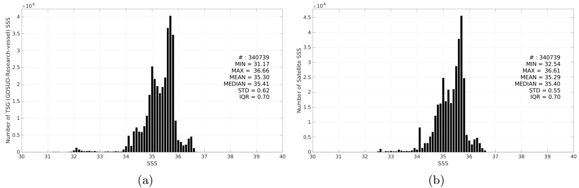
Figure 3: Histograms of SSS from TSG (GOSUD-Research-vessel) (a) and CCI SSS L4 Merged-OI v4.41 - 7-day running (ESA) (b) considering all match-up pairs per bins of 0.1 over the South Pacific Ocean Pi-MEP region and for the full satellite product period.
