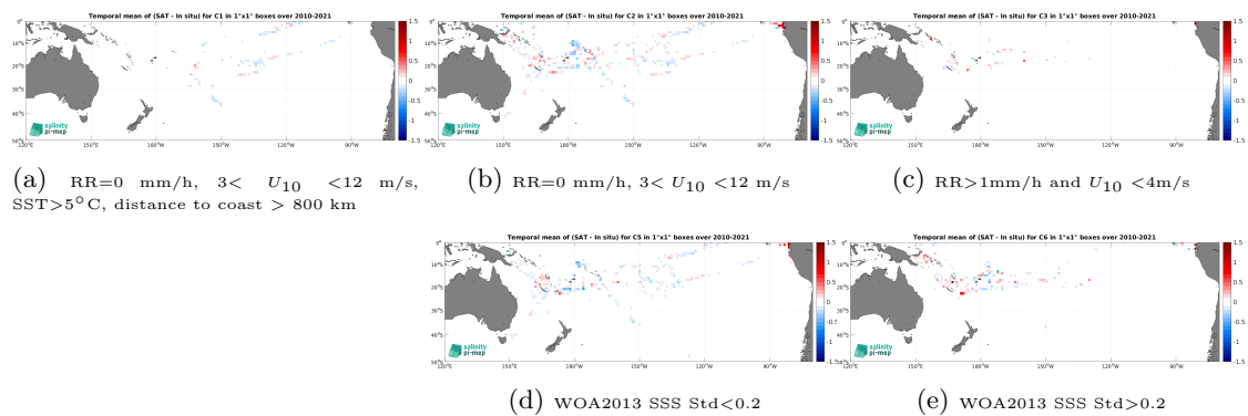
Figure 14: Temporal mean gridded over spatial boxes of size 1^\circ \times 1^\circ of \Delta\text{SSS} (CCI SSS L4 Merged-OI v4.41 - 7-day running (ESA) - TSG (GOSUD-Research-vessel)) for 5 different subdatasets corresponding to:RR=0 mm/h, 3 < U_{10} < 12 m/s, SST>5°C, distance to coast > 800 km (a), RR=0 mm/h, 3 < U_{10} < 12 m/s (b), RR>1mm/h and U_{10} < 4 m/s (c), WOA2013 SSS Std<0.2 (d), WOA2013 SSS Std>0.2 (e).
