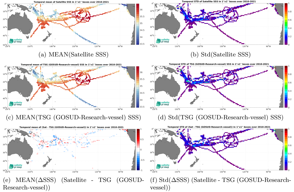
Figure 7: Temporal mean (left) and Std (right) of SSS from CCI SSS L4 Merged-OI v4.41 - 7-day running (ESA) (top), TSG (GOSUD-Research-vessel) (middle), and of \Delta SSS (Satellite - TSG (GOSUD-Research-vessel)). Only match-up pairs are used to generate these maps.
