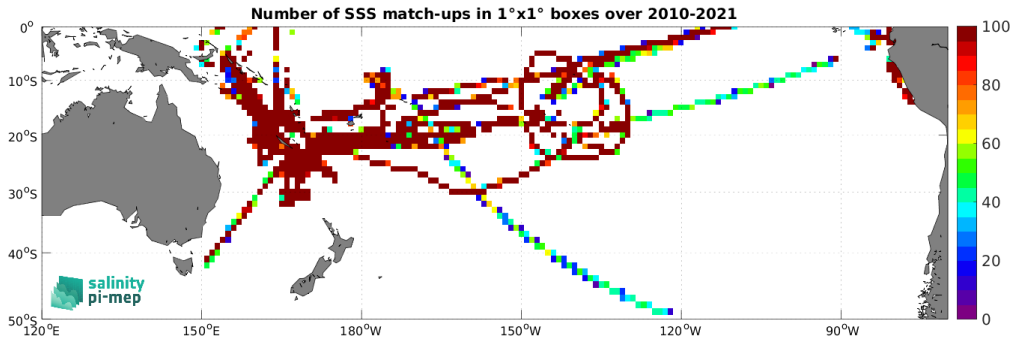
Figure 5: Number of SSS match-ups between TSG (GOSUD-Research-vessel) SSS and the CCI SSS L4 Merged-OI v4.41 - 7-day running (ESA) SSS product for the South Pacific Ocean Pi-MEP region over 1^\circ \times 1^\circ boxes and for the full satellite product period.
