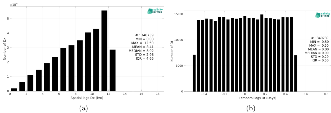
Figure 6: Histograms of the spatial (a) and temporal (b) lags between the location/time of the TSG (GOSUD-Research-vessel) measurement and the date of the corresponding CCI SSS L4 Merged-OI v4.41 - 7-day running (ESA) SSS pixel.
