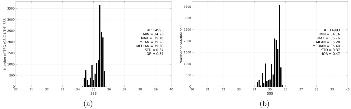
Figure 3: Histograms of SSS from TSG (CSIC-UTM) (a) and CCI SSS L4 Merged-OI v4.41 - 7-day running (ESA) (b) considering all match-up pairs per bins of 0.1 over the South Pacific Ocean Pi-MEP region and for the full satellite product period.
