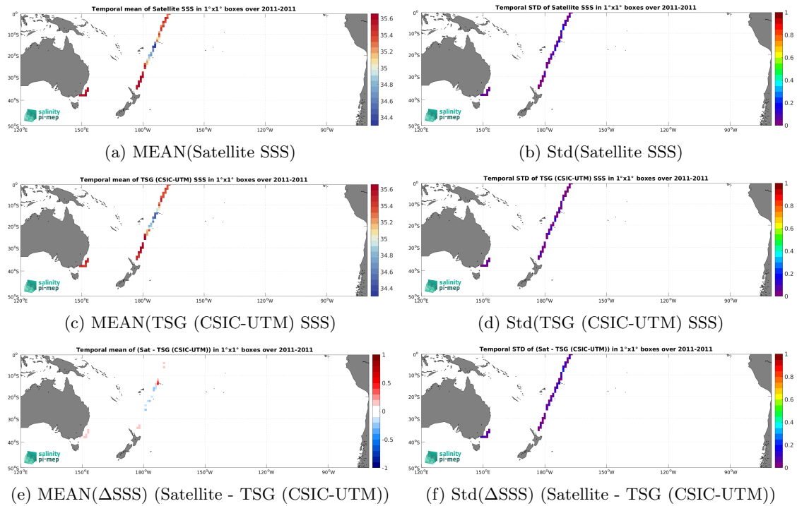
Figure 7: Temporal mean (left) and Std (right) of SSS from CCI SSS L4 Merged-OI v4.41 - 7-day running (ESA) (top), TSG (CSIC-UTM) ( in situ ) dataset (middle), and of \Delta SSS (Satellite - TSG (CSIC-UTM)). Only match-up pairs are used to generate these maps.
