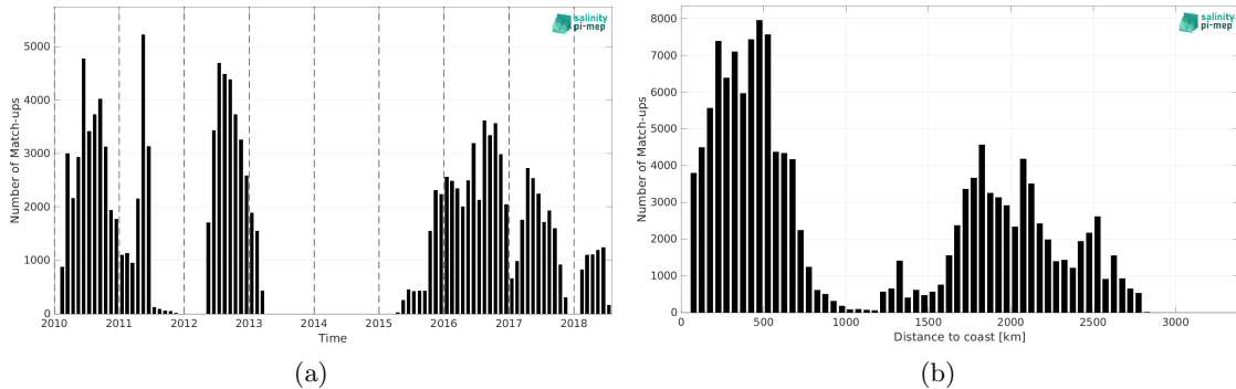
Figure 2: Number of match-ups between Surface drifters and CCI SSS L4 Merged-OI v4.41 - 7-day running (ESA) SSS as a function of time (a) and as function of the distance to coast (b) over the South Pacific Ocean Pi-MEP region and for the full satellite product period.
