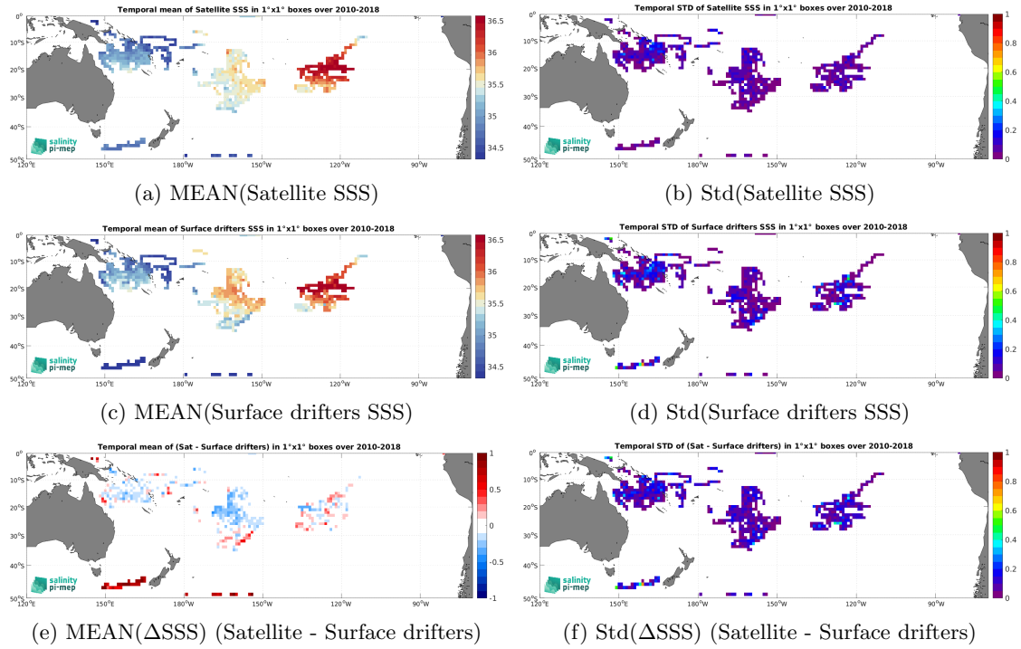
Figure 6: Temporal mean (left) and Std (right) of SSS from CCI SSS L4 Merged-OI v4.41 - 7-day running (ESA) (top), Surface drifters (middle), and of \Delta SSS (Satellite - Surface drifters). Only match-up pairs are used to generate these maps.
