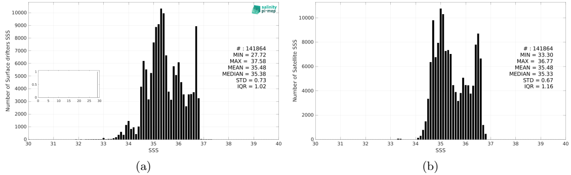
Figure 3: Histograms of SSS from Surface drifters (a) and CCI SSS L4 Merged-OI v4.41 - 7-day running (ESA) (b) considering all match-up pairs per bins of 0.1 over the South Pacific Ocean Pi-MEP region and for the full satellite product period.
