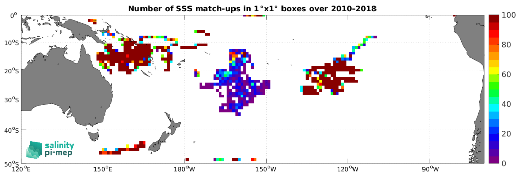
Figure 4: Number of SSS match-ups between Surface drifters SSS and the CCI SSS L4 Merged-OI v4.41 - 7-day running (ESA) SSS product for the South Pacific Ocean Pi-MEP region over 1^\circ \times 1^\circ boxes and for the full satellite product period.
