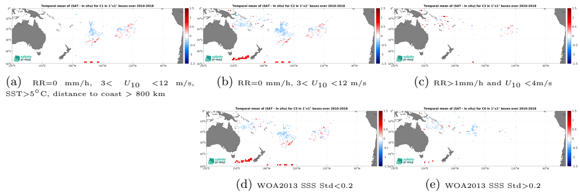
Figure 13: Temporal mean gridded over spatial boxes of size 1^\circ \times 1^\circ of \Delta\text{SSS} (CCI SSS L4 Merged-OI v4.41 - 7-day running (ESA) - Surface drifters) for 5 different subdatasets corresponding to:RR=0 mm/h, 3 < U_{10} < 12 m/s, SST >5^\circ\text{C} , distance to coast > 800 km (a), RR=0 mm/h, 3 < U_{10} < 12 m/s (b), RR >1 mm/h and U_{10} < 4 m/s (c), WOA2013 SSS Std <0.2 (d), WOA2013 SSS Std >0.2 (e).
