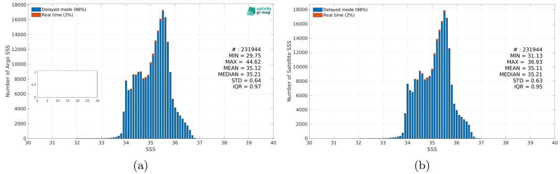
Figure 3: Histograms of SSS from Argo (a) and CCI SSS L4 Merged-OI v4.41 - 7-day running (ESA) (b) considering all match-up pairs per bins of 0.1 over the South Pacific Ocean Pi-MEP region and for the full satellite product period.
