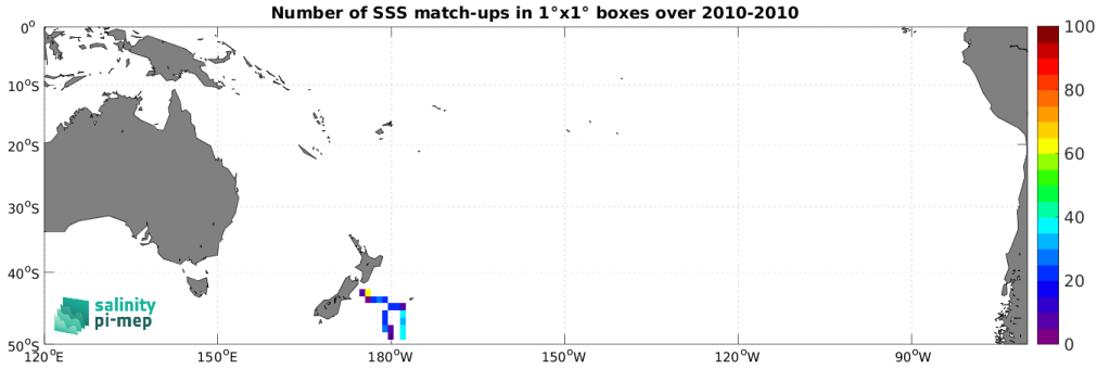
Figure 5: Number of SSS match-ups between TSG (Polarstern) SSS and the CCI SSS L4 Merged-OI v4.41 - 30-day running (ESA) SSS product for the South Pacific Ocean Pi-MEP region over 1^\circ \times 1^\circ boxes and for the full satellite product period.
