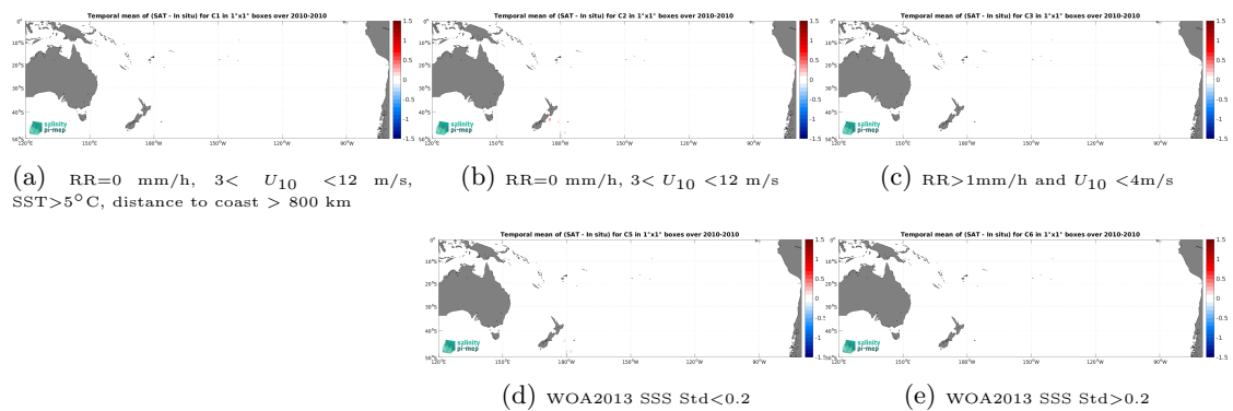
Figure 14: Temporal mean gridded over spatial boxes of size 1^\circ \times 1^\circ of \Delta\text{SSS} (CCI SSS L4 Merged-OI v4.41 - 30-day running (ESA) - TSG (Polarstern)) for 5 different subdatasets corresponding to:RR=0 mm/h, 3 < U_{10} < 12 m/s, SST>5°C, distance to coast > 800 km (a), RR=0 mm/h, 3 < U_{10} < 12 m/s (b), RR>1mm/h and U_{10} < 4 m/s (c), WOA2013 SSS Std<0.2 (d), WOA2013 SSS Std>0.2 (e).
