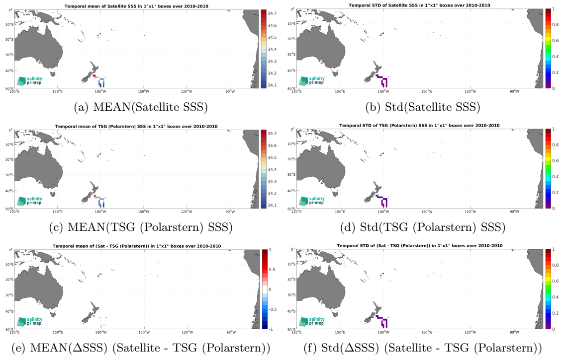
Figure 7: Temporal mean (left) and Std (right) of SSS from CCI SSS L4 Merged-OI v4.41 - 30-day running (ESA) (top), TSG (Polarstern) (middle), and of \Delta SSS (Satellite - TSG (Polarstern)). Only match-up pairs are used to generate these maps.
