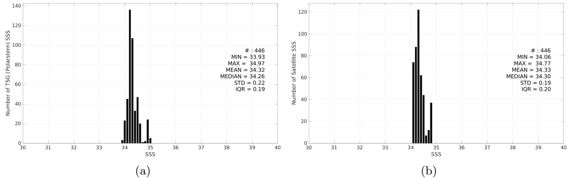
Figure 3: Histograms of SSS from TSG (Polarstern) (a) and CCI SSS L4 Merged-OI v4.41 - 30-day running (ESA) (b) considering all match-up pairs per bins of 0.1 over the South Pacific Ocean Pi-MEP region and for the full satellite product period.
