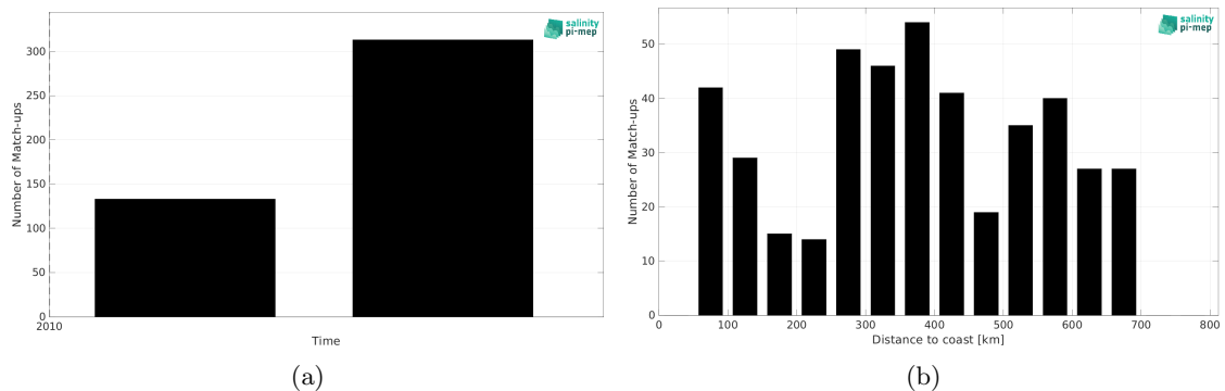
Figure 2: Number of match-ups between TSG (Polarstern) and CCI SSS L4 Merged-OI v4.41 - 30-day running (ESA) SSS as a function of time (a) and as function of the distance to coast (b) over the South Pacific Ocean Pi-MEP region and for the full satellite product period.
