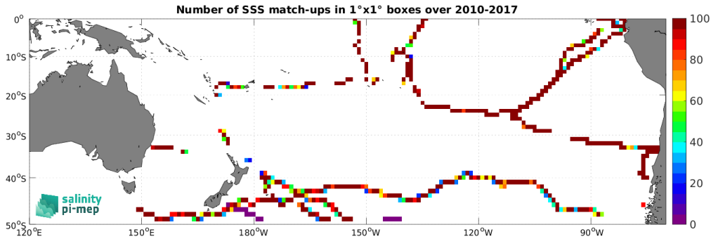
Figure 5: Number of SSS match-ups between TSG (GOSUD-Sailing-ship) SSS and the CCI SSS L4 Merged-OI v4.41 - 30-day running (ESA) SSS product for the South Pacific Ocean Pi-MEP region over 1^\circ \times 1^\circ boxes and for the full satellite product period.
