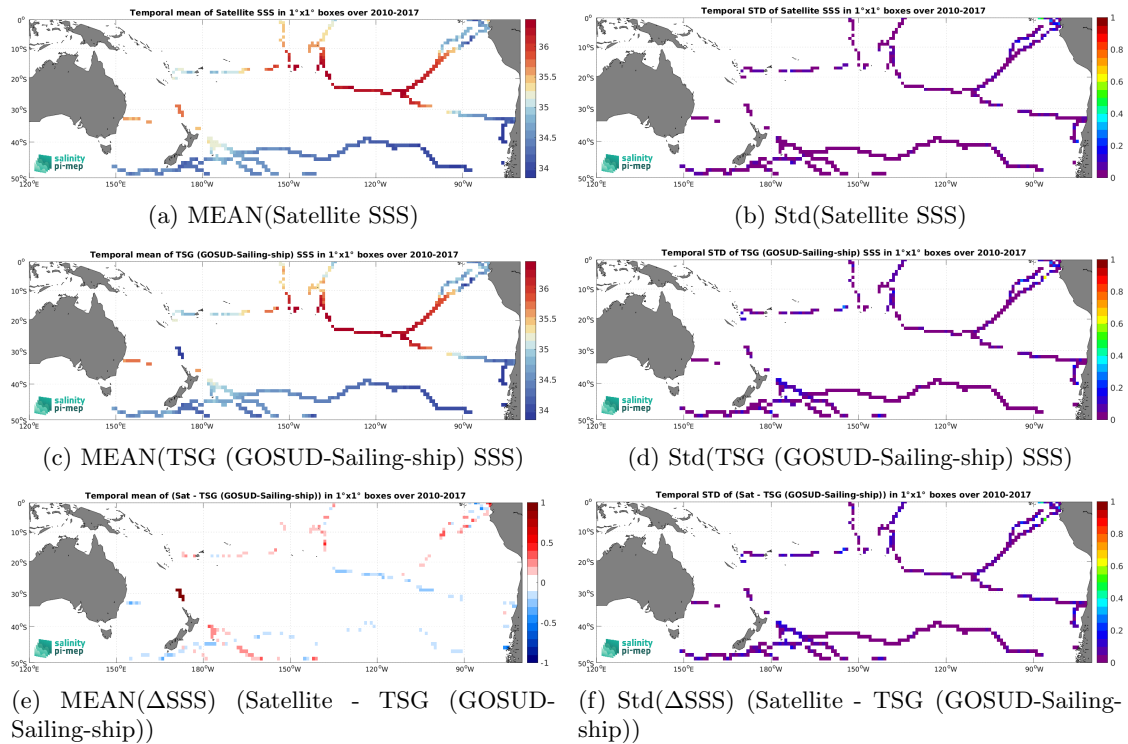
Figure 7: Temporal mean (left) and Std (right) of SSS from CCI SSS L4 Merged-OI v4.41 - 30-day running (ESA) (top), TSG (GOSUD-Sailing-ship) (middle), and of \Delta SSS (Satellite - TSG (GOSUD-Sailing-ship)). Only match-up pairs are used to generate these maps.
