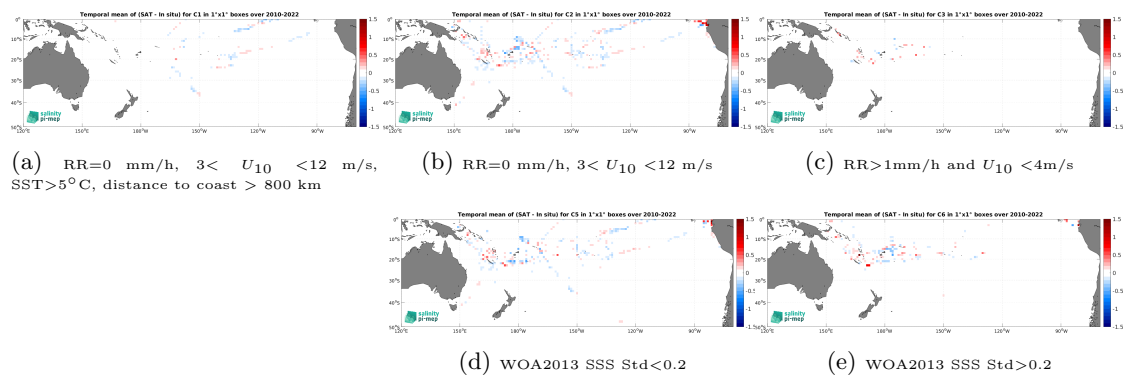
Figure 14: Temporal mean gridded over spatial boxes of size 1^\circ \times 1^\circ of \Delta\text{SSS} (CCI SSS L4 Merged-OI v4.41 - 30-day running (ESA) - TSG (GOSUD-Research-vessel)) for 5 different subdatasets corresponding to:RR=0 mm/h, 3 < U_{10} < 12 m/s, SST >5^\circ\text{C} , distance to coast > 800 km (a), RR=0 mm/h, 3 < U_{10} < 12 m/s (b), RR >1 mm/h and U_{10} < 4 m/s (c), WOA2013 SSS Std <0.2 (d), WOA2013 SSS Std >0.2 (e).
