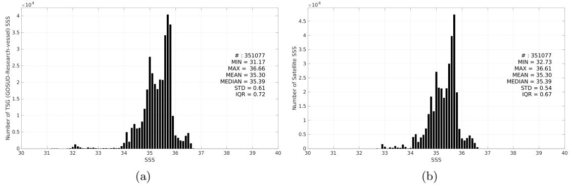
Figure 3: Histograms of SSS from TSG (GOSUD-Research-vessel) (a) and CCI SSS L4 Merged-OI v4.41 - 30-day running (ESA) (b) considering all match-up pairs per bins of 0.1 over the South Pacific Ocean Pi-MEP region and for the full satellite product period.
