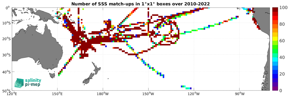
Figure 5: Number of SSS match-ups between TSG (GOSUD-Research-vessel) SSS and the CCI SSS L4 Merged-OI v4.41 - 30-day running (ESA) SSS product for the South Pacific Ocean Pi-MEP region over 1^\circ \times 1^\circ boxes and for the full satellite product period.
