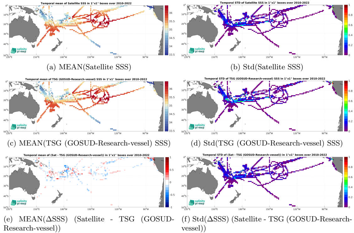
Figure 7: Temporal mean (left) and Std (right) of SSS from CCI SSS L4 Merged-OI v4.41 - 30-day running (ESA) (top), TSG (GOSUD-Research-vessel) (middle), and of \Delta SSS (Satellite - TSG (GOSUD-Research-vessel)). Only match-up pairs are used to generate these maps.
