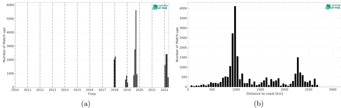
Figure 2: Number of match-ups between Saildrone and CCI SSS L4 Merged-OI v4.41 - 30-day running (ESA) SSS as a function of time (a) and as function of the distance to coast (b) over the South Pacific Ocean Pi-MEP region and for the full satellite product period.
