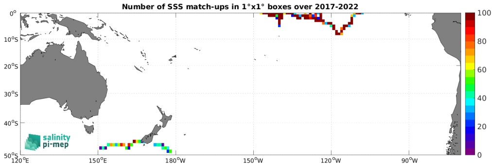
Figure 5: Number of SSS match-ups between Saildrone SSS and the CCI SSS L4 Merged-OI v4.41 - 30-day running (ESA) SSS product for the South Pacific Ocean Pi-MEP region over 1^\circ \times 1^\circ boxes and for the full satellite product period.
