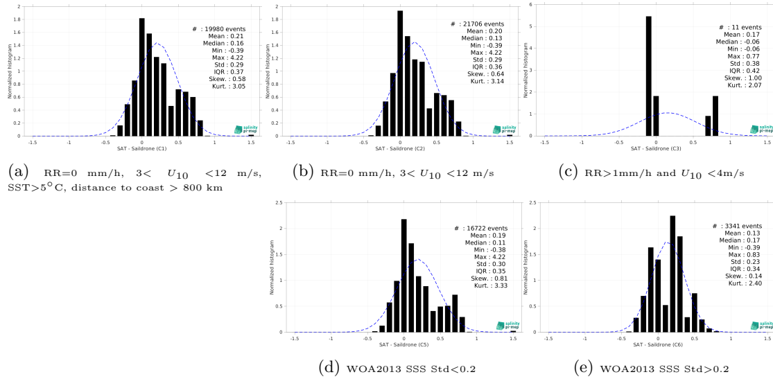
Figure 15: Normalized histogram of \Delta SSS (CCI SSS L4 Merged-OI v4.41 - 30-day running (ESA) - Saldrone) for 5 different subdatasets corresponding to: RR=0 mm/h, 3 < U_{10} < 12 m/s, SST > 5°C, distance to coast > 800 km (a), RR=0 mm/h, 3 < U_{10} < 12 m/s (b), RR > 1mm/h and U_{10} < 4 m/s (c), WOA2013 SSS Std < 0.2 (d), WOA2013 SSS Std > 0.2 (e).
