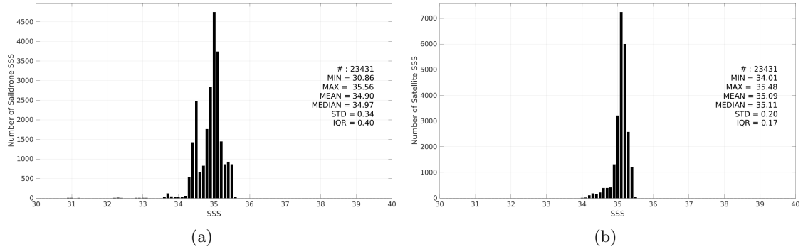
Figure 3: Histograms of SSS from Saildrone (a) and CCI SSS L4 Merged-OI v4.41 - 30-day running (ESA) (b) considering all match-up pairs per bins of 0.1 over the South Pacific Ocean Pi-MEP region and for the full satellite product period.
