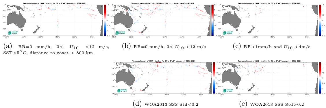
Figure 12: Temporal mean gridded over spatial boxes of size 1^\circ \times 1^\circ of \Delta\text{SSS} (CCI SSS L4 Merged-OI v4.4 - 7-day running (ESA) - TSG (SAMOS)) for 5 different subdatasets corresponding to:RR=0 mm/h, 3 < U_{10} < 12 m/s, SST >5^\circ\text{C} , distance to coast > 800 km (a), RR=0 mm/h, 3 < U_{10} < 12 m/s (b), RR >1 mm/h and U_{10} < 4 m/s (c), WOA2013 SSS Std <0.2 (d), WOA2013 SSS Std >0.2 (e).
