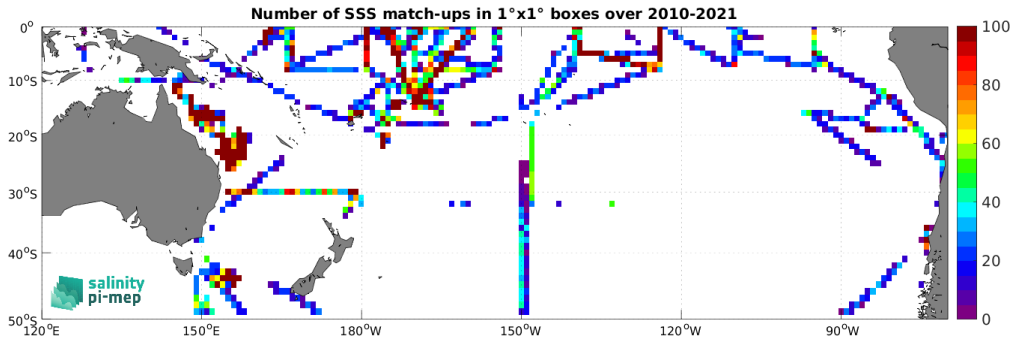
Figure 4: Number of SSS match-ups between TSG (SAMOS) SSS and the CCI SSS L4 Merged-OI v4.4 - 7-day running (ESA) SSS product for the South Pacific Ocean Pi-MEP region over 1^\circ \times 1^\circ boxes and for the full satellite product period.
