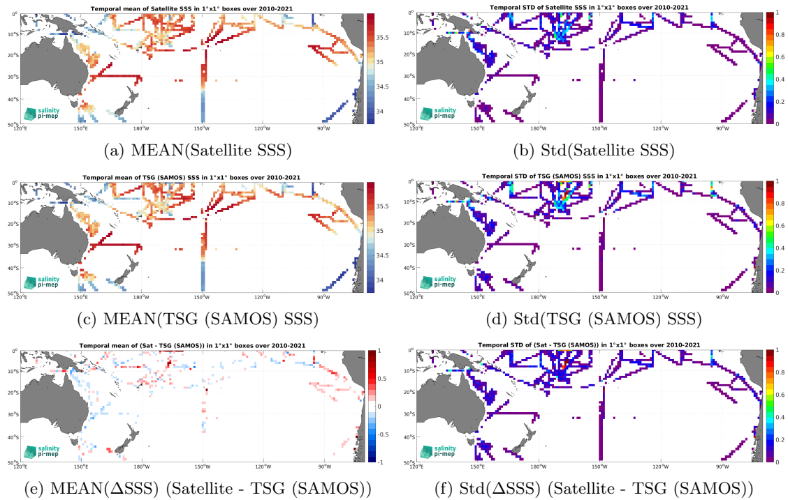
Figure 6: Temporal mean (left) and Std (right) of SSS from CCI SSS L4 Merged-OI v4.4 - 7-day running (ESA) (top), TSG (SAMOS) (middle), and of \Delta SSS (Satellite - TSG (SAMOS)). Only match-up pairs are used to generate these maps.
