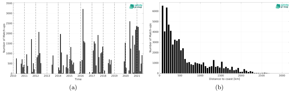
Figure 1: Number of match-ups between TSG (SAMOS) and CCI SSS L4 Merged-OI v4.4 - 7-day running (ESA) SSS as a function of time (a) and as function of the distance to coast (b) over the South Pacific Ocean Pi-MEP region and for the full satellite product period.
