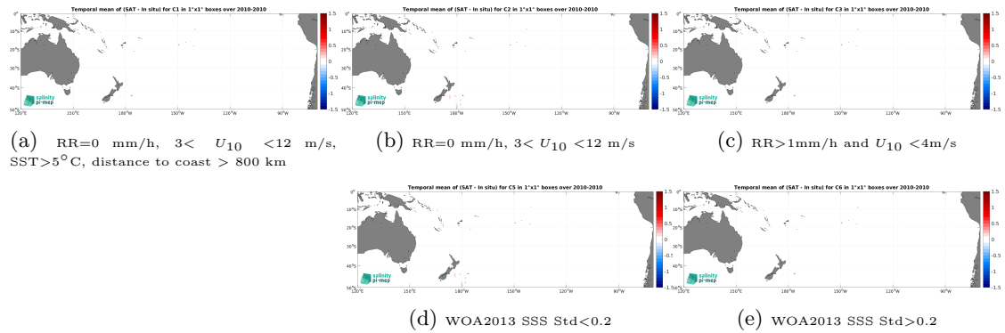
Figure 12: Temporal mean gridded over spatial boxes of size 1^{\circ}\times 1^{\circ} of \Delta\text{SSS} (CCI SSS L4 Merged-OI v4.4 - 7-day running (ESA) - TSG (Polarstern)) for 5 different subdatasets corresponding to:RR=0 mm/h, 3 < U_{10} < 12 m/s, SST >5^{\circ}\text{C} , distance to coast > 800 km (a), RR=0 mm/h, 3 < U_{10} < 12 m/s (b), RR >1 mm/h and U_{10} < 4 m/s (c), WOA2013 SSS Std <0.2 (d), WOA2013 SSS Std >0.2 (e).
