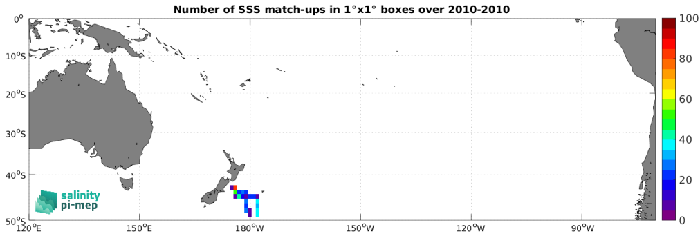
Figure 4: Number of SSS match-ups between TSG (Polarstern) SSS and the CCI SSS L4 Merged-OI v4.4 - 7-day running (ESA) SSS product for the South Pacific Ocean Pi-MEP region over 1^\circ \times 1^\circ boxes and for the full satellite product period.
