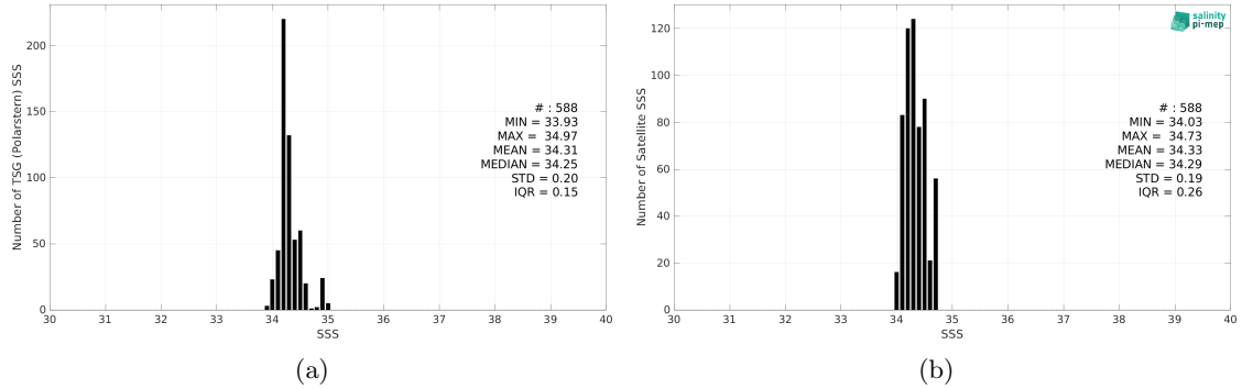
Figure 2: Histograms of SSS from TSG (Polarstern) (a) and CCI SSS L4 Merged-OI v4.4 - 7-day running (ESA) (b) considering all match-up pairs per bins of 0.1 over the South Pacific Ocean Pi-MEP region and for the full satellite product period.
