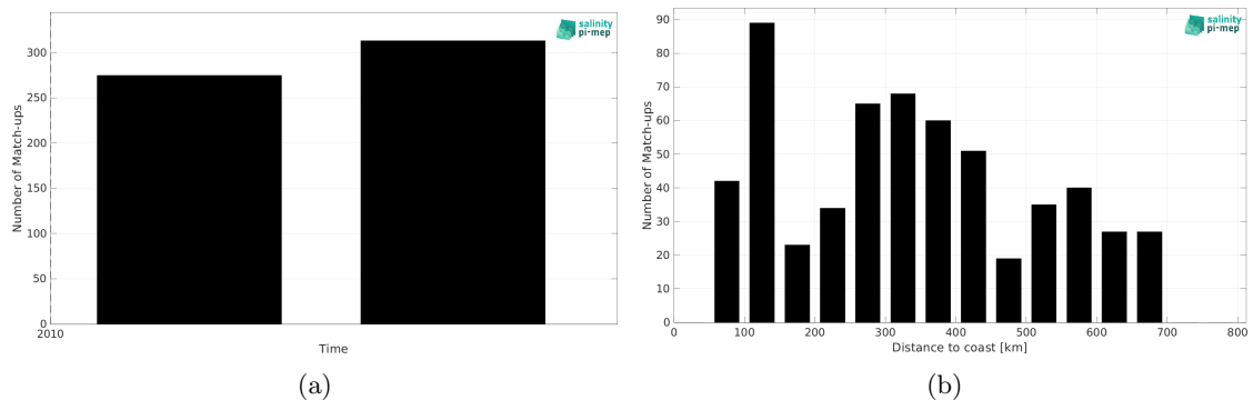
Figure 1: Number of match-ups between TSG (Polarstern) and CCI SSS L4 Merged-OI v4.4 - 7-day running (ESA) SSS as a function of time (a) and as function of the distance to coast (b) over the South Pacific Ocean Pi-MEP region and for the full satellite product period.
