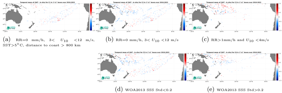
Figure 12: Temporal mean gridded over spatial boxes of size 1^\circ \times 1^\circ of \Delta\text{SSS} (CCI SSS L4 Merged-OI v4.4 - 7-day running (ESA) - TSG (LEGOS-DM)) for 5 different subdatasets corresponding to:RR=0 mm/h, 3 < U_{10} < 12 m/s, SST >5^\circ\text{C} , distance to coast > 800 km (a), RR=0 mm/h, 3 < U_{10} < 12 m/s (b), RR >1 mm/h and U_{10} < 4 m/s (c), WOA2013 SSS Std <0.2 (d), WOA2013 SSS Std >0.2 (e).
