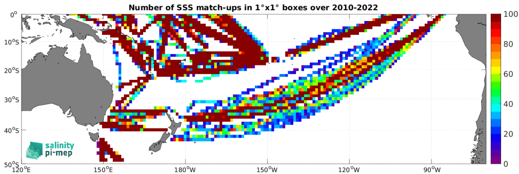
Figure 4: Number of SSS match-ups between TSG (LEGOS-DM) SSS and the CCI SSS L4 Merged-OI v4.4 - 7-day running (ESA) SSS product for the South Pacific Ocean Pi-MEP region over 1^\circ \times 1^\circ boxes and for the full satellite product period.
