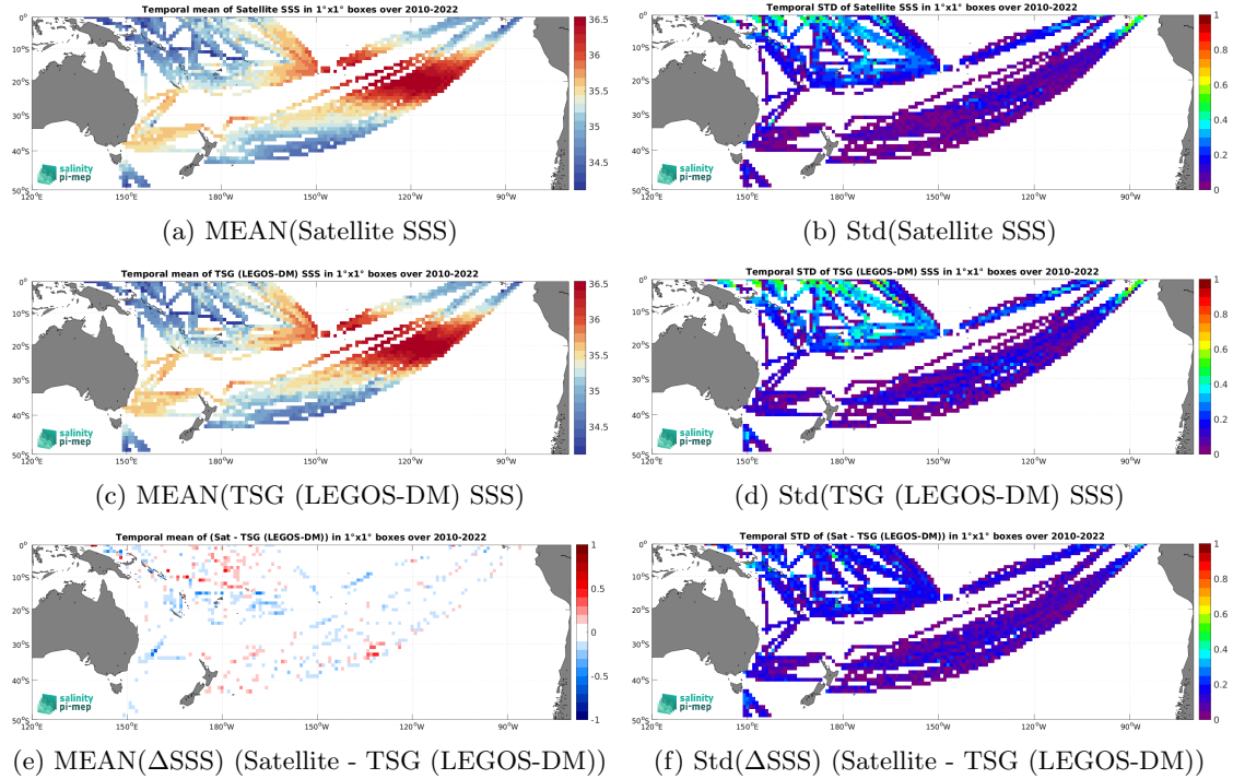
Figure 6: Temporal mean (left) and Std (right) of SSS from CCI SSS L4 Merged-OI v4.4 - 7-day running (ESA) (top), TSG (LEGOS-DM) ( in situ dataset) (middle), and of \Delta\text{SSS} (Satellite - TSG (LEGOS-DM)). Only match-up pairs are used to generate these maps.
