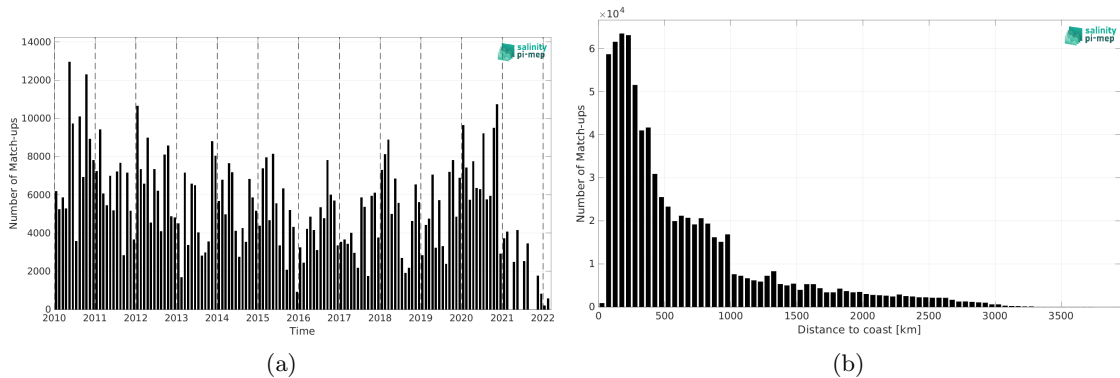
Figure 1: Number of match-ups between TSG (LEGOS-DM) and CCI SSS L4 Merged-OI v4.4 - 7-day running (ESA) SSS as a function of time (a) and as function of the distance to coast (b) over the South Pacific Ocean Pi-MEP region and for the full satellite product period.
