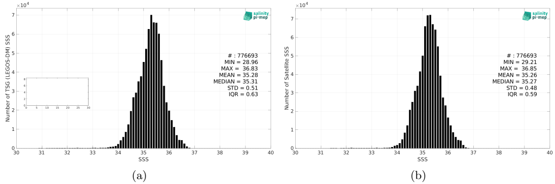
Figure 2: Histograms of SSS from TSG (LEGOS-DM) (a) and CCI SSS L4 Merged-OI v4.4 - 7-day running (ESA) (b) considering all match-up pairs per bins of 0.1 over the South Pacific Ocean Pi-MEP region and for the full satellite product period.
