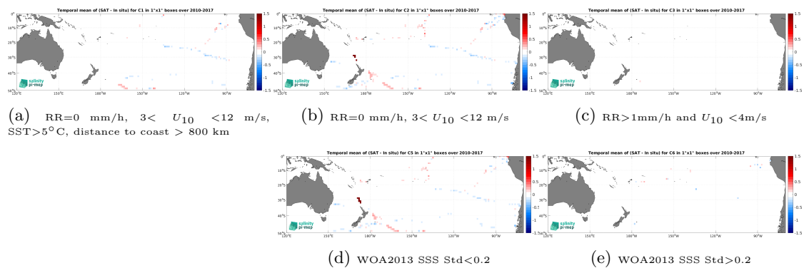
Figure 12: Temporal mean gridded over spatial boxes of size 1^\circ \times 1^\circ of \Delta\text{SSS} (CCI SSS L4 Merged-OI v4.4 - 7-day running (ESA) - TSG (GOSUD-Sailing-ship)) for 5 different subdatasets corresponding to:RR=0 mm/h, 3 < U_{10} < 12 m/s, SST >5^\circ\text{C} , distance to coast > 800 km (a), RR=0 mm/h, 3 < U_{10} < 12 m/s (b), RR >1 mm/h and U_{10} < 4 m/s (c), WOA2013 SSS Std <0.2 (d), WOA2013 SSS Std >0.2 (e).
