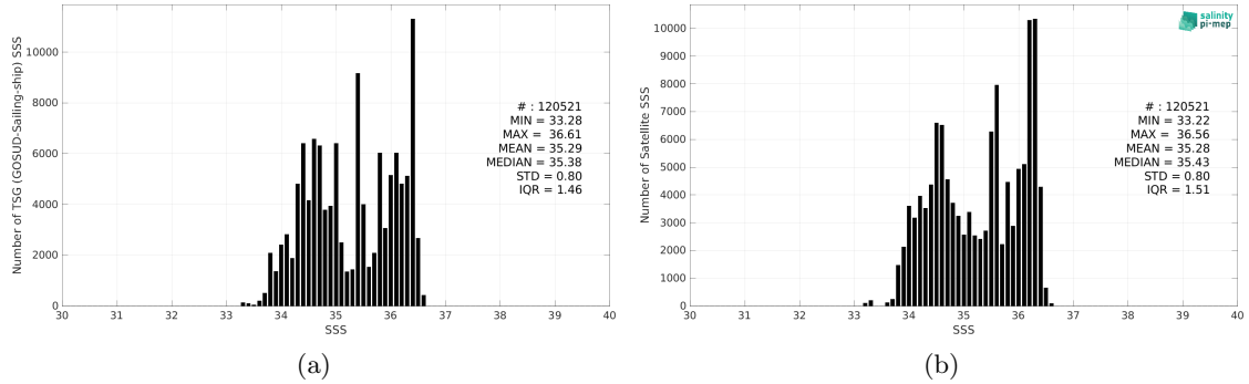
Figure 2: Histograms of SSS from TSG (GOSUD-Sailing-ship) (a) and CCI SSS L4 Merged-OI v4.4 - 7-day running (ESA) (b) considering all match-up pairs per bins of 0.1 over the South Pacific Ocean Pi-MEP region and for the full satellite product period.
