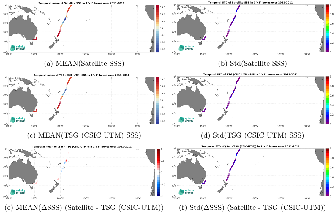
Figure 6: Temporal mean (left) and Std (right) of SSS from CCI SSS L4 Merged-OI v4.4 - 7-day running (ESA) (top), TSG (CSIC-UTM) (middle), and of \Delta SSS (Satellite - TSG (CSIC-UTM)). Only match-up pairs are used to generate these maps.
