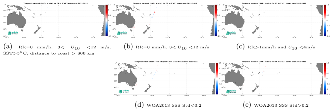
Figure 12: Temporal mean gridded over spatial boxes of size 1^\circ \times 1^\circ of \Delta SSS (CCI SSS L4 Merged-OI v4.4 - 7-day running (ESA) - TSG (CSIC-UTM)) for 5 different subdatasets corresponding to:RR=0 mm/h, 3 < U_{10} < 12 m/s, SST >5^\circ C, distance to coast > 800 km (a), RR=0 mm/h, 3 < U_{10} < 12 m/s (b), RR >1 mm/h and U_{10} < 4 m/s (c), WOA2013 SSS Std <0.2 (d), WOA2013 SSS Std >0.2 (e).
