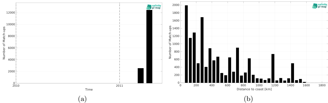
Figure 1: Number of match-ups between TSG (CSIC-UTM) and CCI SSS L4 Merged-OI v4.4 - 7-day running (ESA) SSS as a function of time (a) and as function of the distance to coast (b) over the South Pacific Ocean Pi-MEP region and for the full satellite product period.
