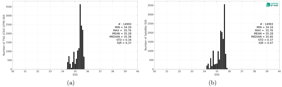
Figure 2: Histograms of SSS from TSG (CSIC-UTM) (a) and CCI SSS L4 Merged-OI v4.4 - 7-day running (ESA) (b) considering all match-up pairs per bins of 0.1 over the South Pacific Ocean Pi-MEP region and for the full satellite product period.
