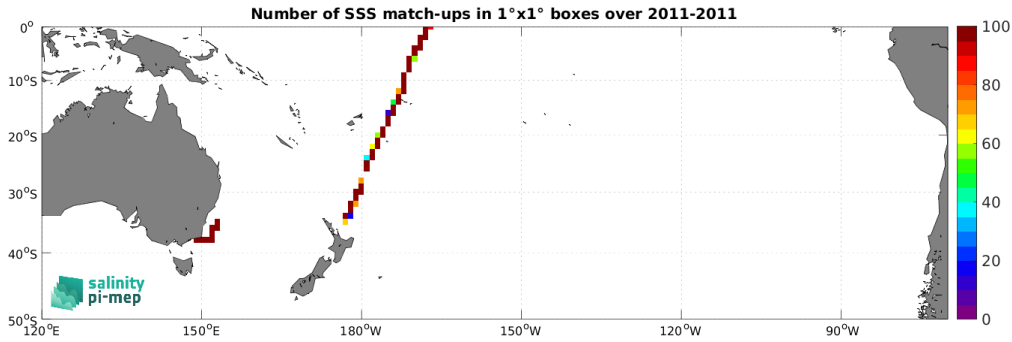
Figure 4: Number of SSS match-ups between TSG (CSIC-UTM) SSS and the CCI SSS L4 Merged-OI v4.4 - 7-day running (ESA) SSS product for the South Pacific Ocean Pi-MEP region over 1^\circ \times 1^\circ boxes and for the full satellite product period.
