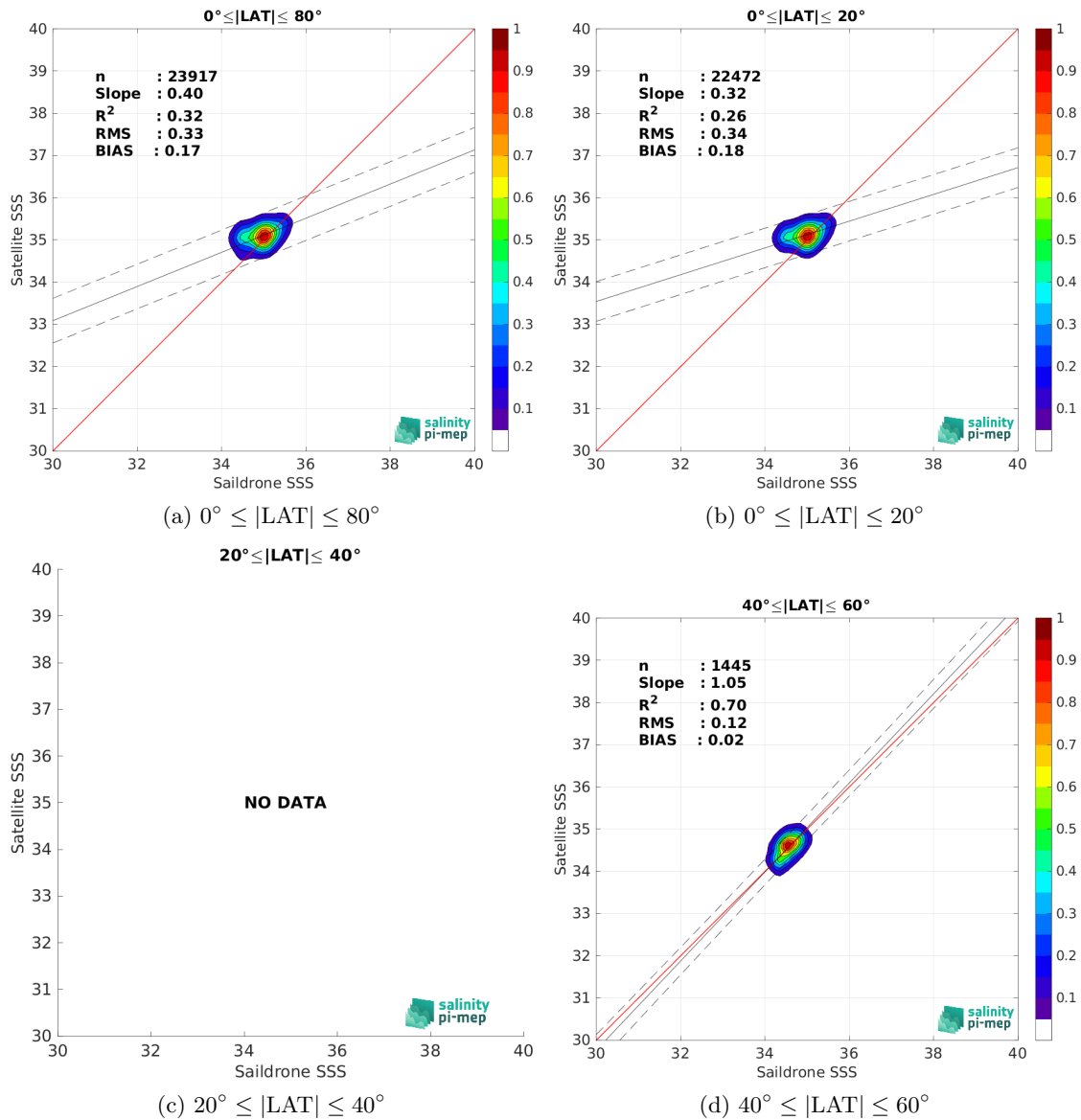
Figure 9: Contour maps of the concentration of CCI SSS L4 Merged-OI v4.4 - 7-day running (ESA) SSS (y-axis) versus Saldrone SSS (x-axis) at match-up pairs for different latitude bands. For each plot, the red line shows x=y . The black thin and dashed lines indicate a linear fit through the data cloud and the \pm 95\% confidence levels, respectively. The number match-up pairs n , the slope and R^2 coefficient of the linear fit, the root mean square (RMS) and the mean bias between satellite and in situ data are indicated for each latitude band in each plots.
