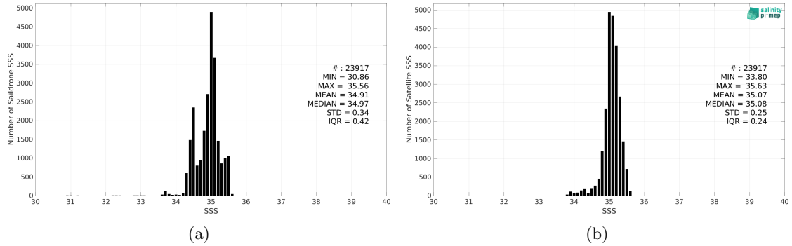
Figure 2: Histograms of SSS from Saildrone (a) and CCI SSS L4 Merged-OI v4.4 - 7-day running (ESA) (b) considering all match-up pairs per bins of 0.1 over the South Pacific Ocean Pi-MEP region and for the full satellite product period.
