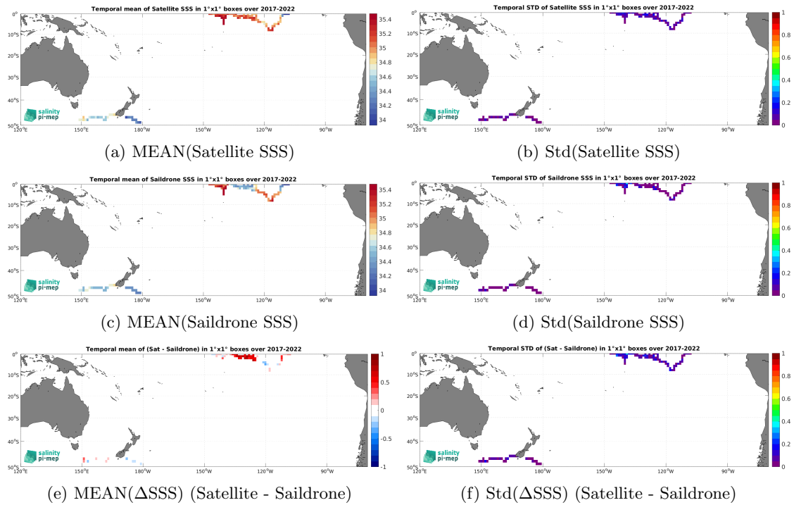
Figure 6: Temporal mean (left) and Std (right) of SSS from CCI SSS L4 Merged-OI v4.4 - 7-day running (ESA) (top), Saildrone (middle), and of \Delta SSS (Satellite - Saildrone). Only match-up pairs are used to generate these maps.
