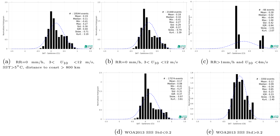
Figure 13: Normalized histogram of \Delta SSS (CCI SSS L4 Merged-OI v4.4 - 7-day running (ESA) - Saildrone) for 5 different subdatasets corresponding to: RR=0 mm/h, 3 < U_{10} < 12 m/s, SST>5°C, distance to coast > 800 km (a), RR=0 mm/h, 3 < U_{10} < 12 m/s (b), RR>1mm/h and U_{10} < 4 m/s (c), WOA2013 SSS Std<0.2 (d), WOA2013 SSS Std>0.2 (e).
