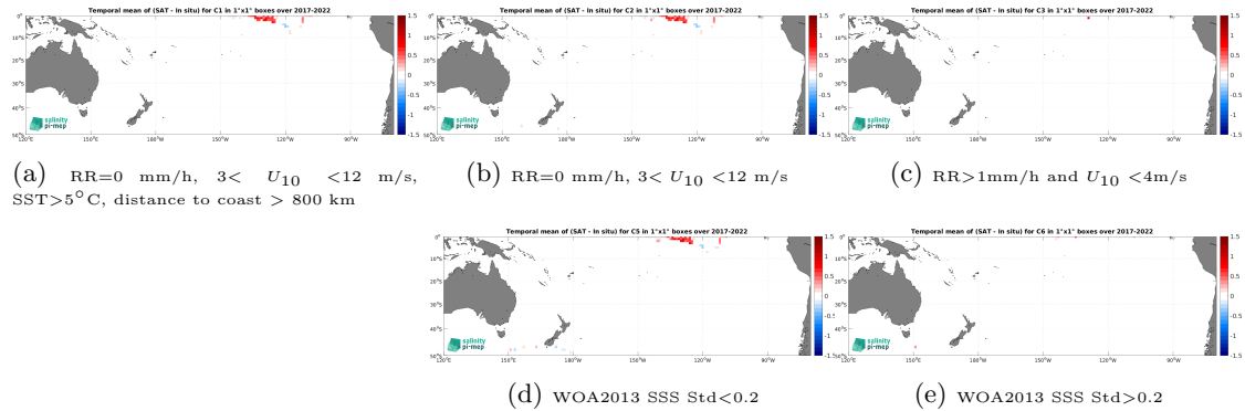
Figure 12: Temporal mean gridded over spatial boxes of size 1^\circ \times 1^\circ of \Delta SSS (CCI SSS L4 Merged-OI v4.4 - 7-day running (ESA) - Sairdrone) for 5 different subdatasets corresponding to:RR=0 mm/h, 3 < U_{10} < 12 m/s, SST >5^\circ\text{C} , distance to coast > 800 km (a), RR=0 mm/h, 3 < U_{10} < 12 m/s (b), RR >1 mm/h and U_{10} < 4 m/s (c), WOA2013 SSS Std <0.2 (d), WOA2013 SSS Std >0.2 (e).
