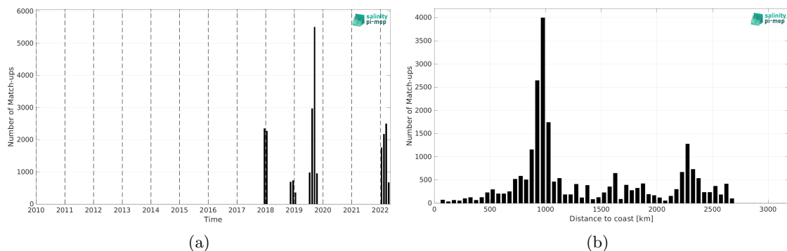
Figure 1: Number of match-ups between Saildrone and CCI SSS L4 Merged-OI v4.4 - 7-day running (ESA) SSS as a function of time (a) and as function of the distance to coast (b) over the South Pacific Ocean Pi-MEP region and for the full satellite product period.
