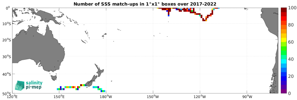
Figure 4: Number of SSS match-ups between Saildrone SSS and the CCI SSS L4 Merged-OI v4.4 - 7-day running (ESA) SSS product for the South Pacific Ocean Pi-MEP region over 1^\circ \times 1^\circ boxes and for the full satellite product period.
