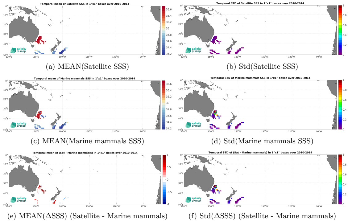
Figure 6: Temporal mean (left) and Std (right) of SSS from CCI SSS L4 Merged-OI v4.4 - 7-day running (ESA) (top), Marine mammals (middle), and of \Delta SSS (Satellite - Marine mammals). Only match-up pairs are used to generate these maps.
