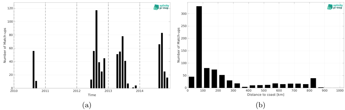
Figure 1: Number of match-ups between Marine mammals and CCI SSS L4 Merged-OI v4.4 - 7-day running (ESA) SSS as a function of time (a) and as function of the distance to coast (b) over the South Pacific Ocean Pi-MEP region and for the full satellite product period.
