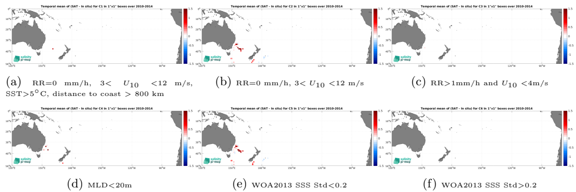
Figure 12: Temporal mean gridded over spatial boxes of size 1^\circ \times 1^\circ of \Delta SSS (CCI SSS L4 Merged-OI v4.4 - 7-day running (ESA) - Marine mammals) for 6 different subdatasets corresponding to:RR=0 mm/h, 3 < U_{10} < 12 m/s, SST >5^\circ C, distance to coast > 800 km (a), RR=0 mm/h, 3 < U_{10} < 12 m/s (b), RR >1 mm/h and U_{10} < 4 m/s (c),MLD <20 m (d),WOA2013 SSS Std <0.2 (e),WOA2013 SSS Std >0.2 (f).
