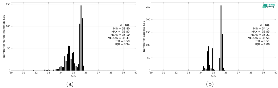
Figure 2: Histograms of SSS from Marine mammals (a) and CCI SSS L4 Merged-OI v4.4 - 7-day running (ESA) (b) considering all match-up pairs per bins of 0.1 over the South Pacific Ocean Pi-MEP region and for the full satellite product period.
