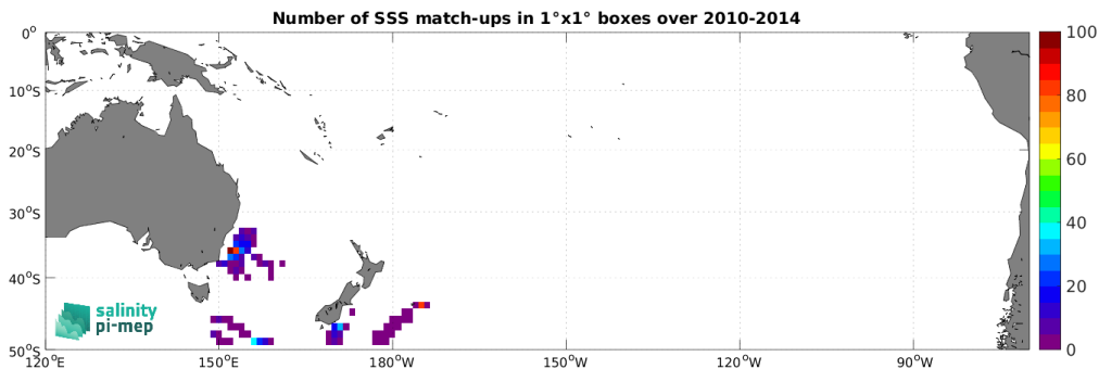
Figure 4: Number of SSS match-ups between Marine mammals SSS and the CCI SSS L4 Merged-OI v4.4 - 7-day running (ESA) SSS product for the South Pacific Ocean Pi-MEP region over 1^\circ \times 1^\circ boxes and for the full satellite product period.
