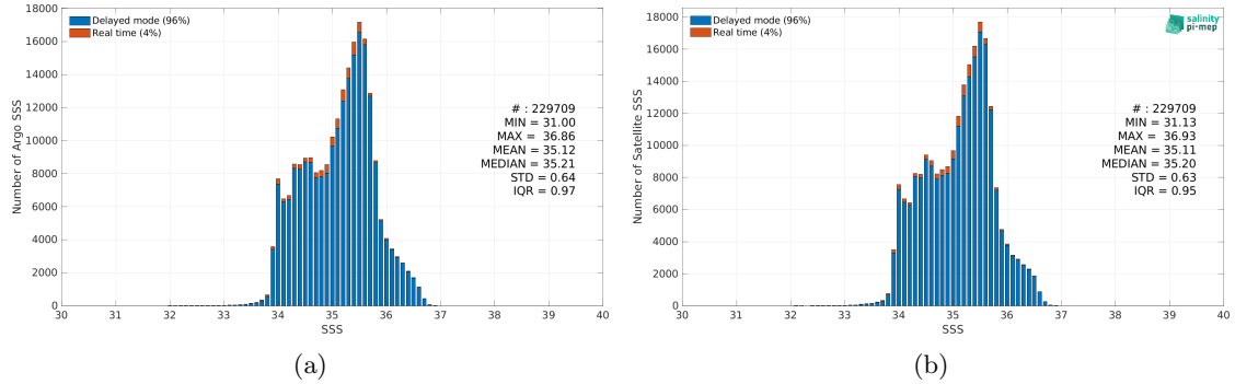
Figure 2: Histograms of SSS from Argo (a) and CCI SSS L4 Merged-OI v4.4 - 7-day running (ESA) (b) considering all match-up pairs per bins of 0.1 over the South Pacific Ocean Pi-MEP region and for the full satellite product period.
