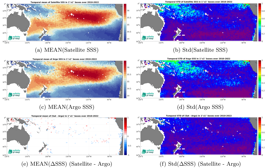
Figure 6: Temporal mean (left) and Std (right) of SSS from CCI SSS L4 Merged-OI v4.4 - 7-day running (ESA) (top), Argo (middle), and of \Delta SSS (Satellite - Argo). Only match-up pairs are used to generate these maps.
