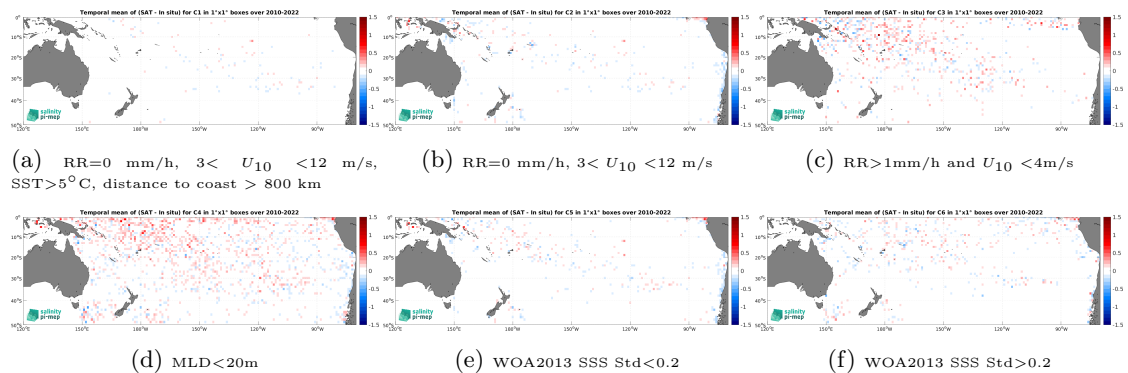
Figure 12: Temporal mean gridded over spatial boxes of size 1^\circ \times 1^\circ of \Delta SSS (CCI SSS L4 Merged-OI v4.4 - 7-day running (ESA) - Argo) for 6 different subdatasets corresponding to:RR=0 mm/h, 3 < U_{10} < 12 m/s, SST >5^\circ C, distance to coast > 800 km (a), RR=0 mm/h, 3 < U_{10} < 12 m/s (b), RR >1 mm/h and U_{10} < 4 m/s (c),MLD <20 m (d),WOA2013 SSS Std <0.2 (e),WOA2013 SSS Std >0.2 (f).
