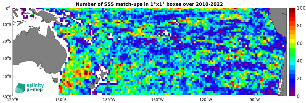
Figure 4: Number of SSS match-ups between Argo SSS and the CCI SSS L4 Merged-OI v4.4 - 7-day running (ESA) SSS product for the South Pacific Ocean Pi-MEP region over 1^\circ \times 1^\circ boxes and for the full satellite product period.
