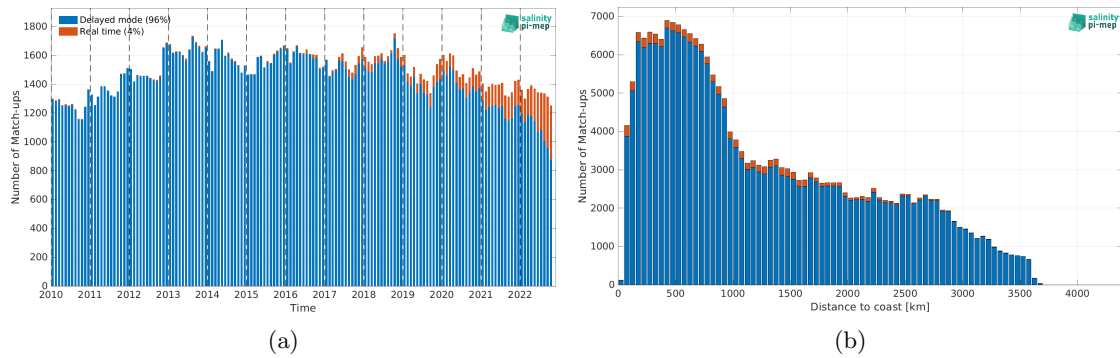
Figure 1: Number of match-ups between Argo and CCI SSS L4 Merged-OI v4.4 - 7-day running (ESA) SSS as a function of time (a) and as function of the distance to coast (b) over the South Pacific Ocean Pi-MEP region and for the full satellite product period.
