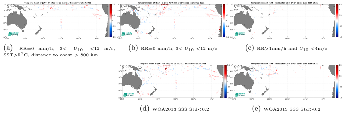
Figure 12: Temporal mean gridded over spatial boxes of size 1^\circ \times 1^\circ of \Delta SSS (CCI SSS L4 Merged-OI v4.4 - 30-day running (ESA) - TSG (SAMOS)) for 5 different subdatasets corresponding to:RR=0 mm/h, 3 < U_{10} < 12 m/s, SST >5^\circ C, distance to coast > 800 km (a), RR=0 mm/h, 3 < U_{10} < 12 m/s (b), RR >1 mm/h and U_{10} < 4 m/s (c), WOA2013 SSS Std <0.2 (d), WOA2013 SSS Std >0.2 (e).
