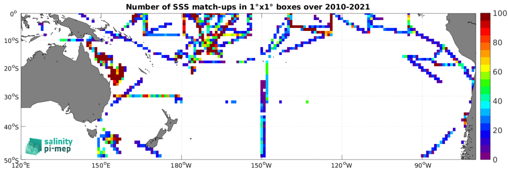
Figure 4: Number of SSS match-ups between TSG (SAMOS) SSS and the CCI SSS L4 Merged-OI v4.4 - 30-day running (ESA) SSS product for the South Pacific Ocean Pi-MEP region over 1^\circ \times 1^\circ boxes and for the full satellite product period.
