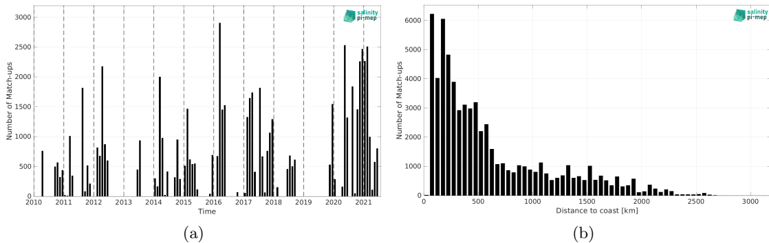
Figure 1: Number of match-ups between TSG (SAMOS) and CCI SSS L4 Merged-OI v4.4 - 30-day running (ESA) SSS as a function of time (a) and as function of the distance to coast (b) over the South Pacific Ocean Pi-MEP region and for the full satellite product period.
