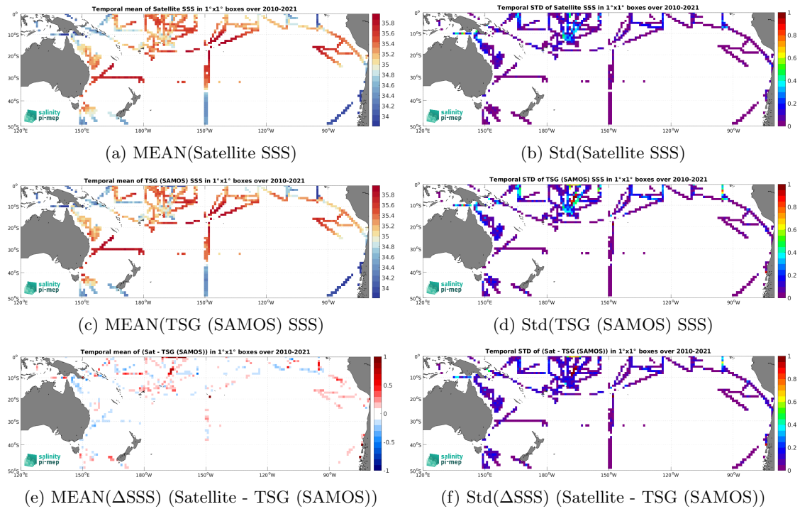
Figure 6: Temporal mean (left) and Std (right) of SSS from CCI SSS L4 Merged-OI v4.4 - 30-day running (ESA) (top), TSG (SAMOS) (middle), and of \Delta SSS (Satellite - TSG (SAMOS)). Only match-up pairs are used to generate these maps.
