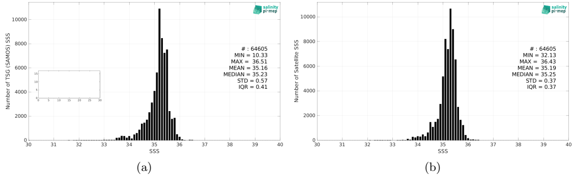
Figure 2: Histograms of SSS from TSG (SAMOS) (a) and CCI SSS L4 Merged-OI v4.4 - 30-day running (ESA) (b) considering all match-up pairs per bins of 0.1 over the South Pacific Ocean Pi-MEP region and for the full satellite product period.
