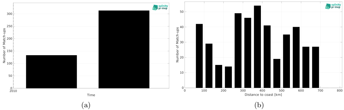
Figure 1: Number of match-ups between TSG (Polarstern) and CCI SSS L4 Merged-OI v4.4 - 30-day running (ESA) SSS as a function of time (a) and as function of the distance to coast (b) over the South Pacific Ocean Pi-MEP region and for the full satellite product period.
