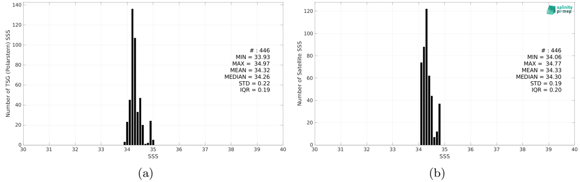
Figure 2: Histograms of SSS from TSG (Polarstern) (a) and CCI SSS L4 Merged-OI v4.4 - 30-day running (ESA) (b) considering all match-up pairs per bins of 0.1 over the South Pacific Ocean Pi-MEP region and for the full satellite product period.
