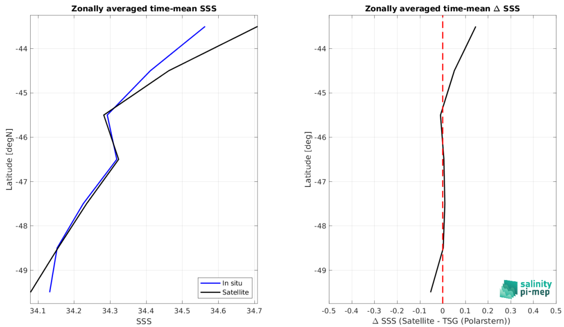
Figure 8: Left panel: Zonal mean SSS from CCI SSS L4 Merged-OI v4.4 - 30-day running (ESA) satellite product (black) and from TSG (Polarstern) (blue). Right panel: Zonal mean of \Delta SSS (Satellite - TSG (Polarstern)) for all the collected Pi-MEP match-up pairs estimated over the full satellite product period.
