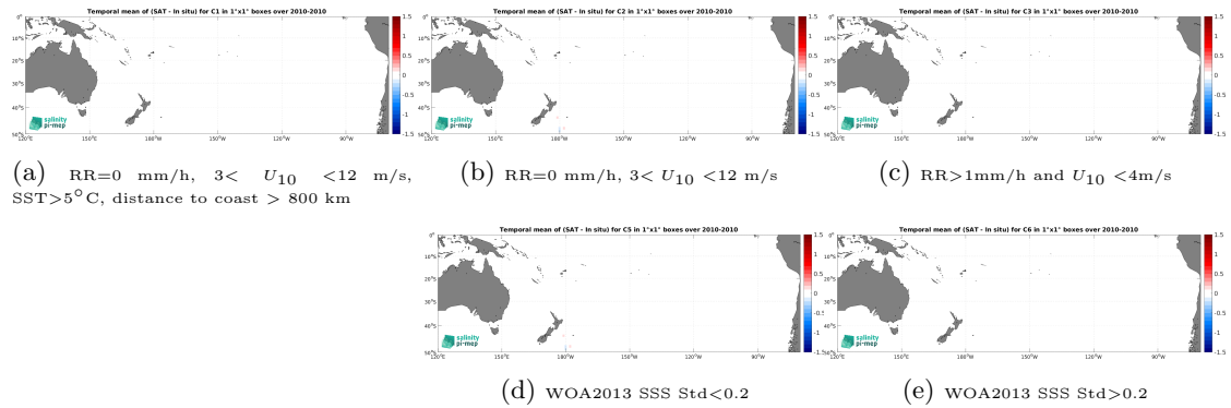
Figure 12: Temporal mean gridded over spatial boxes of size 1^{\circ}\times 1^{\circ} of \Delta\text{SSS} (CCI SSS L4 Merged-OI v4.4 - 30-day running (ESA) - TSG (Polarstern)) for 5 different subdatasets corresponding to:RR=0 mm/h, 3 < U_{10} < 12 m/s, SST >5^{\circ}\text{C} , distance to coast > 800 km (a), RR=0 mm/h, 3 < U_{10} < 12 m/s (b), RR >1 mm/h and U_{10} < 4 m/s (c), WOA2013 SSS Std <0.2 (d), WOA2013 SSS Std >0.2 (e).
