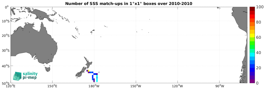
Figure 4: Number of SSS match-ups between TSG (Polarstern) SSS and the CCI SSS L4 Merged-OI v4.4 - 30-day running (ESA) SSS product for the South Pacific Ocean Pi-MEP region over 1^\circ \times 1^\circ boxes and for the full satellite product period.
