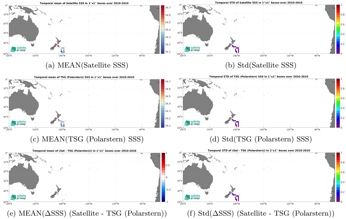
Figure 6: Temporal mean (left) and Std (right) of SSS from CCI SSS L4 Merged-OI v4.4 - 30-day running (ESA) (top), TSG (Polarstern) (middle), and of \Delta SSS (Satellite - TSG (Polarstern)). Only match-up pairs are used to generate these maps.
