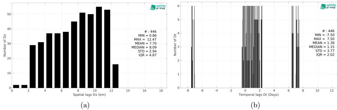
Figure 5: Histograms of the spatial (a) and temporal (b) lags between the location/time of the TSG (Polarstern) measurement and the date of the corresponding CCI SSS L4 Merged-OI v4.4 - 30-day running (ESA) SSS pixel.
