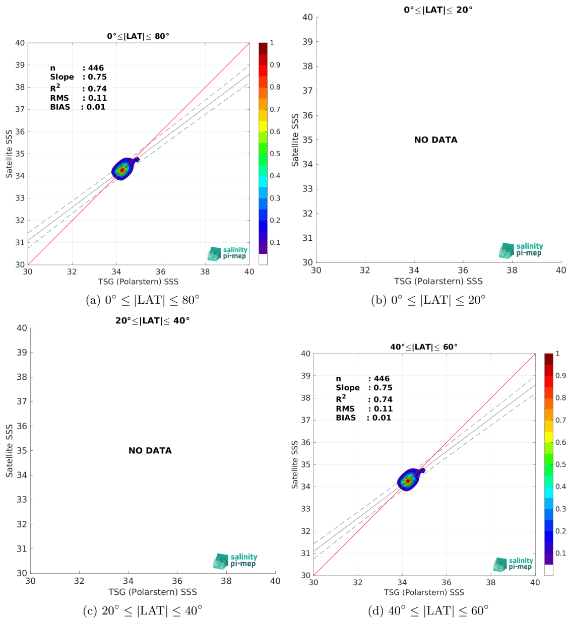
Figure 9: Contour maps of the concentration of CCI SSS L4 Merged-OI v4.4 - 30-day running (ESA) SSS (y-axis) versus TSG (Polarstern) SSS (x-axis) at match-up pairs for different latitude bands. For each plot, the red line shows x=y . The black thin and dashed lines indicate a linear fit through the data cloud and the \pm 95\% confidence levels, respectively. The number match-up pairs n , the slope and R^2 coefficient of the linear fit, the root mean square (RMS) and the mean bias between satellite and in situ data are indicated for each latitude band in each plots.
