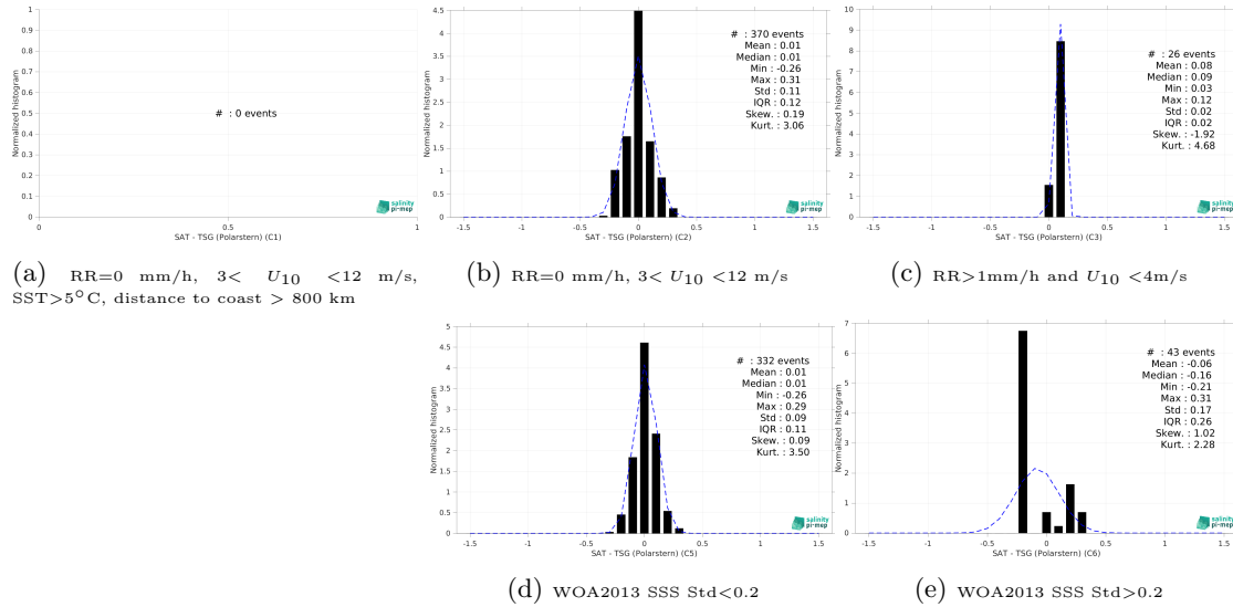
Figure 13: Normalized histogram of \Delta SSS (CCI SSS L4 Merged-OI v4.4 - 30-day running (ESA) - TSG (Polarstern)) for 5 different subdatasets corresponding to: RR=0 mm/h, 3 < U_{10} < 12 m/s, SST > 5°C, distance to coast > 800 km (a), RR=0 mm/h, 3 < U_{10} < 12 m/s (b), RR > 1mm/h and U_{10} < 4 m/s (c), WOA2013 SSS Std < 0.2 (d), WOA2013 SSS Std > 0.2 (e).
