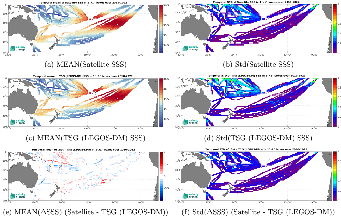
Figure 6: Temporal mean (left) and Std (right) of SSS from CCI SSS L4 Merged-OI v4.4 - 30-day running (ESA) (top), TSG (LEGOS-DM) (middle), and of \Delta\text{SSS} (Satellite - TSG (LEGOS-DM)). Only match-up pairs are used to generate these maps.
