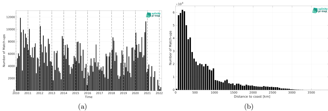
Figure 1: Number of match-ups between TSG (LEGOS-DM) and CCI SSS L4 Merged-OI v4.4 - 30-day running (ESA) SSS as a function of time (a) and as function of the distance to coast (b) over the South Pacific Ocean Pi-MEP region and for the full satellite product period.
