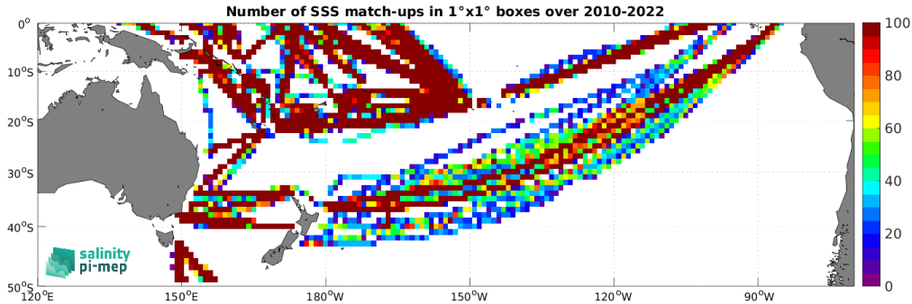
Figure 4: Number of SSS match-ups between TSG (LEGOS-DM) SSS and the CCI SSS L4 Merged-OI v4.4 - 30-day running (ESA) SSS product for the South Pacific Ocean Pi-MEP region over 1^\circ \times 1^\circ boxes and for the full satellite product period.
