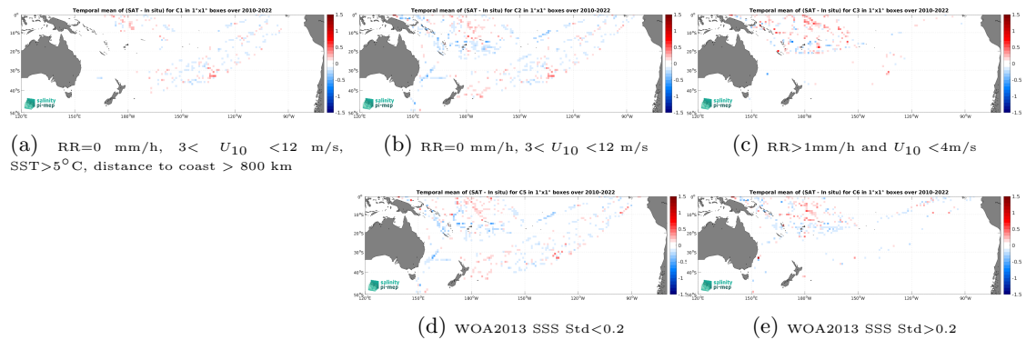
Figure 12: Temporal mean gridded over spatial boxes of size 1^\circ \times 1^\circ of \Delta\text{SSS} (CCI SSS L4 Merged-OI v4.4 - 30-day running (ESA) - TSG (LEGOS-DM)) for 5 different subdatasets corresponding to:RR=0 mm/h, 3 < U_{10} < 12 m/s, SST >5^\circ\text{C} , distance to coast > 800 km (a), RR=0 mm/h, 3 < U_{10} < 12 m/s (b), RR >1 mm/h and U_{10} < 4 m/s (c), WOA2013 SSS Std <0.2 (d), WOA2013 SSS Std >0.2 (e).
