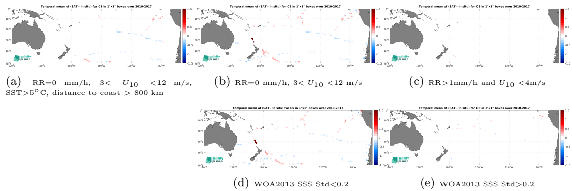
Figure 12: Temporal mean gridded over spatial boxes of size 1^\circ \times 1^\circ of \Delta SSS (CCI SSS L4 Merged-OI v4.4 - 30-day running (ESA) - TSG (GOSUD-Sailing-ship)) for 5 different subdatasets corresponding to:RR=0 mm/h, 3 < U_{10} < 12 m/s, SST>5°C, distance to coast > 800 km (a), RR=0 mm/h, 3 < U_{10} < 12 m/s (b), RR>1mm/h and U_{10} < 4 m/s (c), WOA2013 SSS Std<0.2 (d), WOA2013 SSS Std>0.2 (e).
