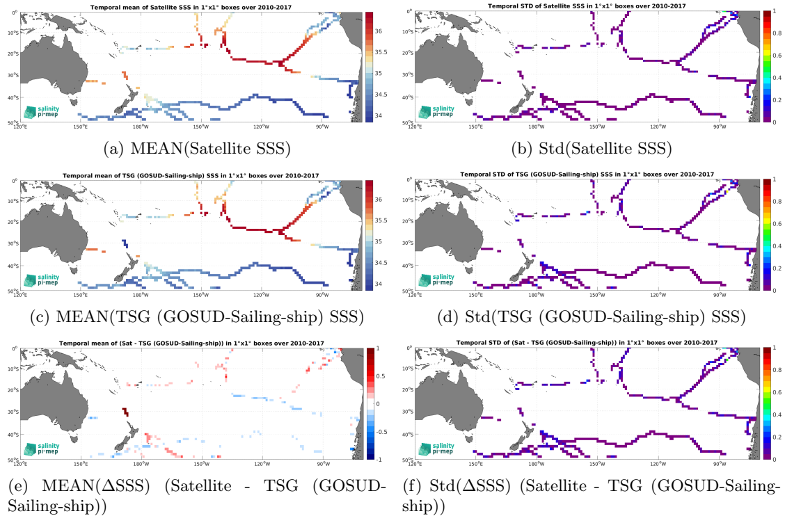
Figure 6: Temporal mean (left) and Std (right) of SSS from CCI SSS L4 Merged-OI v4.4 - 30-day running (ESA) (top), TSG (GOSUD-Sailing-ship) (middle), and of \Delta SSS (Satellite - TSG (GOSUD-Sailing-ship)). Only match-up pairs are used to generate these maps.
