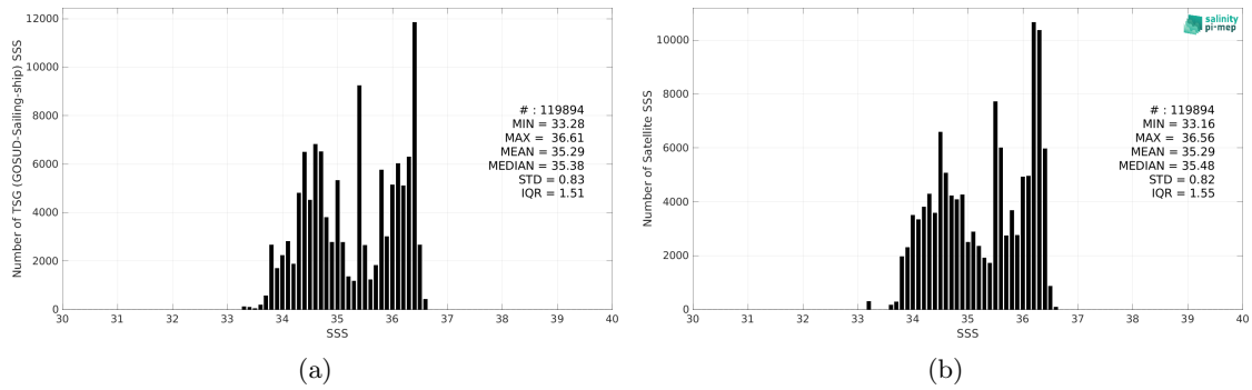
Figure 2: Histograms of SSS from TSG (GOSUD-Sailing-ship) (a) and CCI SSS L4 Merged-OI v4.4 - 30-day running (ESA) (b) considering all match-up pairs per bins of 0.1 over the South Pacific Ocean Pi-MEP region and for the full satellite product period.
