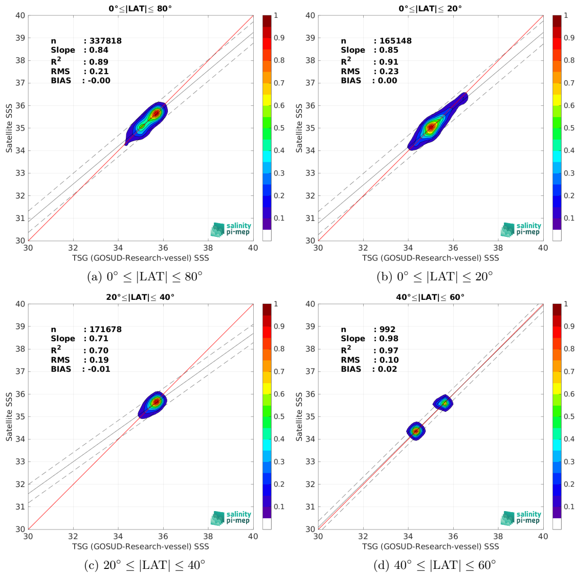
Figure 9: Contour maps of the concentration of CCI SSS L4 Merged-OI v4.4 - 30-day running (ESA) SSS (y-axis) versus TSG (GOSUD-Research-vessel) SSS (x-axis) at match-up pairs for different latitude bands. For each plot, the red line shows x=y . The black thin and dashed lines indicate a linear fit through the data cloud and the \pm 95\% confidence levels, respectively. The number match-up pairs n , the slope and R^2 coefficient of the linear fit, the root mean square (RMS) and the mean bias between satellite and in situ data are indicated for each latitude band in each plots.
