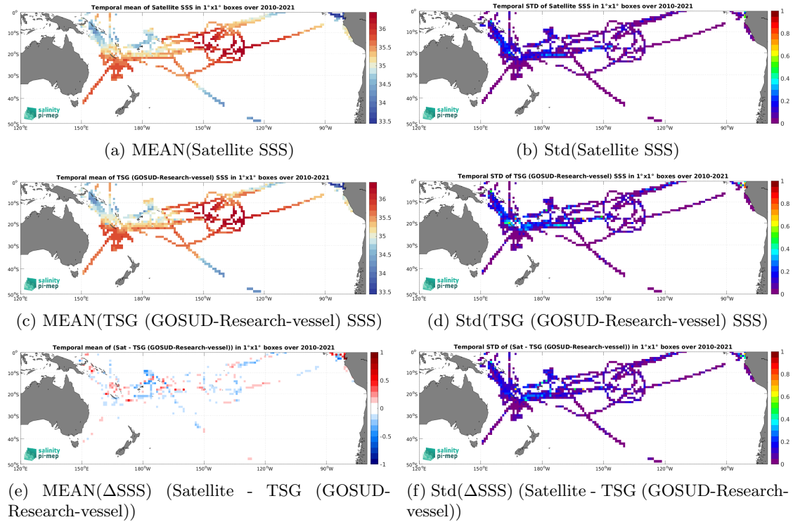
Figure 6: Temporal mean (left) and Std (right) of SSS from CCI SSS L4 Merged-OI v4.4 - 30-day running (ESA) (top), TSG (GOSUD-Research-vessel) (middle), and of \Delta SSS (Satellite - TSG (GOSUD-Research-vessel)). Only match-up pairs are used to generate these maps.
