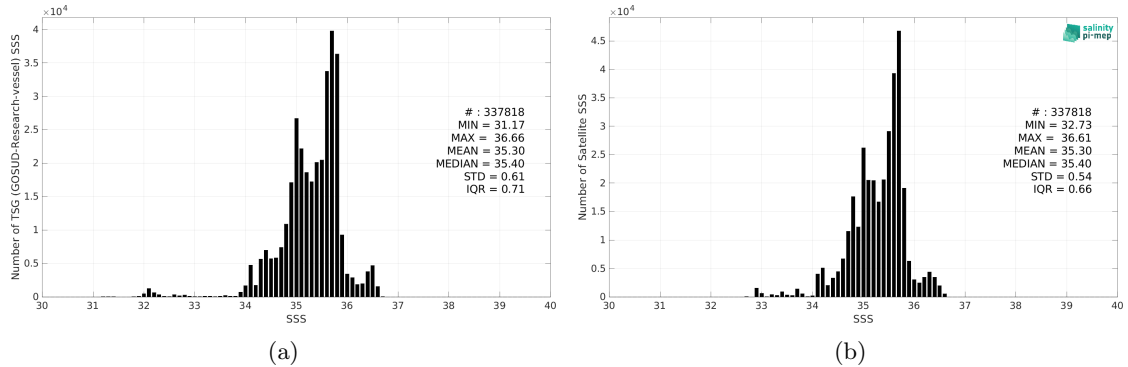
Figure 2: Histograms of SSS from TSG (GOSUD-Research-vessel) (a) and CCI SSS L4 Merged-OI v4.4 - 30-day running (ESA) (b) considering all match-up pairs per bins of 0.1 over the South Pacific Ocean Pi-MEP region and for the full satellite product period.
