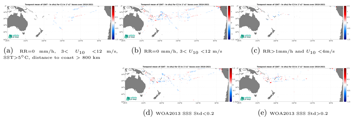
Figure 12: Temporal mean gridded over spatial boxes of size 1^\circ \times 1^\circ of \Delta SSS (CCI SSS L4 Merged-OI v4.4 - 30-day running (ESA) - TSG (GOSUD-Research-vessel)) for 5 different subdatasets corresponding to:RR=0 mm/h, 3 < U_{10} < 12 m/s, SST >5^\circ\text{C} , distance to coast > 800 km (a), RR=0 mm/h, 3 < U_{10} < 12 m/s (b), RR >1 mm/h and U_{10} < 4 m/s (c), WOA2013 SSS Std <0.2 (d), WOA2013 SSS Std >0.2 (e).
