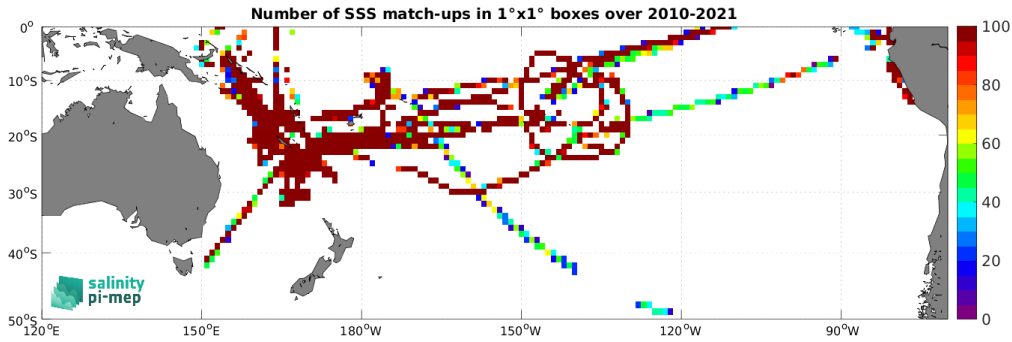
Figure 4: Number of SSS match-ups between TSG (GOSUD-Research-vessel) SSS and the CCI SSS L4 Merged-OI v4.4 - 30-day running (ESA) SSS product for the South Pacific Ocean Pi-MEP region over 1^\circ \times 1^\circ boxes and for the full satellite product period.
