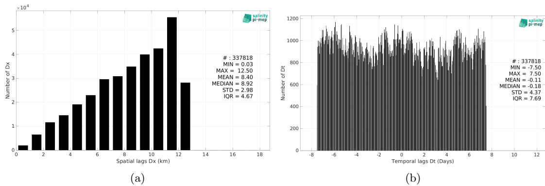
Figure 5: Histograms of the spatial (a) and temporal (b) lags between the location/time of the TSG (GOSUD-Research-vessel) measurement and the date of the corresponding CCI SSS L4 Merged-OI v4.4 - 30-day running (ESA) SSS pixel.
