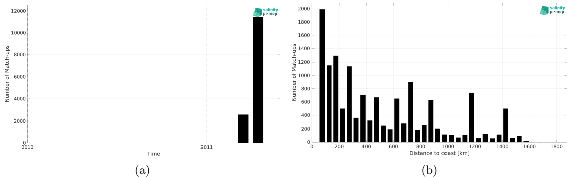
Figure 1: Number of match-ups between TSG (CSIC-UTM) and CCI SSS L4 Merged-OI v4.4 - 30-day running (ESA) SSS as a function of time (a) and as function of the distance to coast (b) over the South Pacific Ocean Pi-MEP region and for the full satellite product period.
