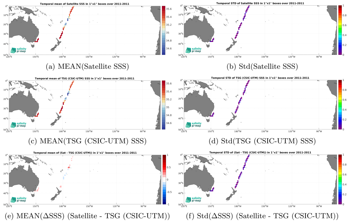
Figure 6: Temporal mean (left) and Std (right) of SSS from CCI SSS L4 Merged-OI v4.4 - 30-day running (ESA) (top), TSG (CSIC-UTM) ( in situ ) dataset (middle), and of \Delta SSS (Satellite - TSG (CSIC-UTM)). Only match-up pairs are used to generate these maps.
