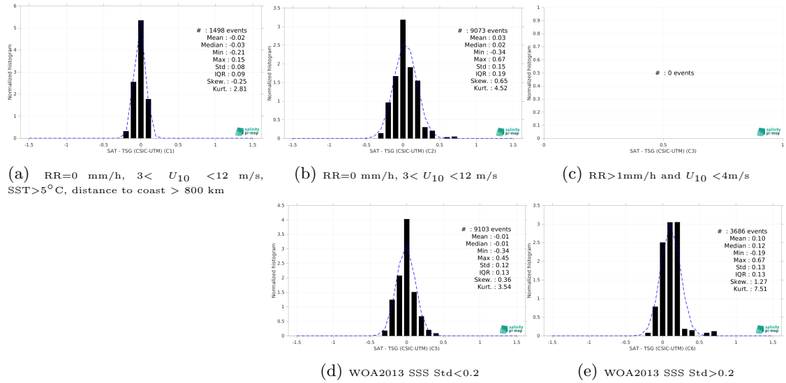
Figure 13: Normalized histogram of \Delta SSS (CCI SSS L4 Merged-OI v4.4 - 30-day running (ESA) - TSG (CSIC-UTM)) for 5 different subdatasets corresponding to: RR=0 mm/h, 3 < U_{10} < 12 m/s, SST > 5°C, distance to coast > 800 km (a), RR=0 mm/h, 3 < U_{10} < 12 m/s (b), RR > 1mm/h and U_{10} < 4 m/s (c), WOA2013 SSS Std < 0.2 (d), WOA2013 SSS Std > 0.2 (e).
