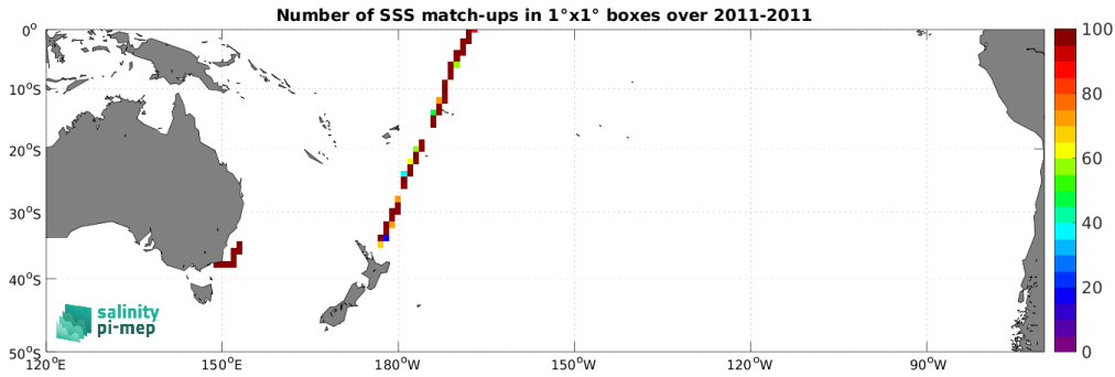
Figure 4: Number of SSS match-ups between TSG (CSIC-UTM) SSS and the CCI SSS L4 Merged-OI v4.4 - 30-day running (ESA) SSS product for the South Pacific Ocean Pi-MEP region over 1^\circ \times 1^\circ boxes and for the full satellite product period.
