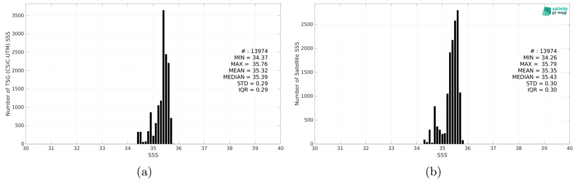
Figure 2: Histograms of SSS from TSG (CSIC-UTM) (a) and CCI SSS L4 Merged-OI v4.4 - 30-day running (ESA) (b) considering all match-up pairs per bins of 0.1 over the South Pacific Ocean Pi-MEP region and for the full satellite product period.
