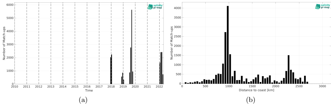
Figure 1: Number of match-ups between Saildrone and CCI SSS L4 Merged-OI v4.4 - 30-day running (ESA) SSS as a function of time (a) and as function of the distance to coast (b) over the South Pacific Ocean Pi-MEP region and for the full satellite product period.
