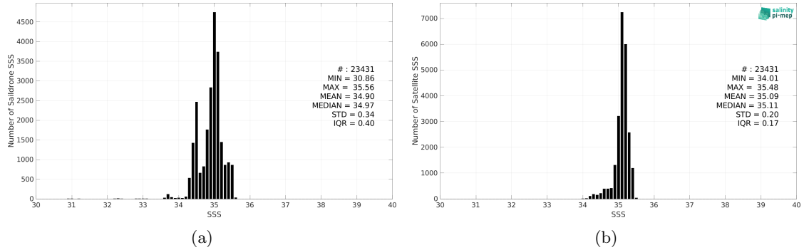
Figure 2: Histograms of SSS from Saildrone (a) and CCI SSS L4 Merged-OI v4.4 - 30-day running (ESA) (b) considering all match-up pairs per bins of 0.1 over the South Pacific Ocean Pi-MEP region and for the full satellite product period.
