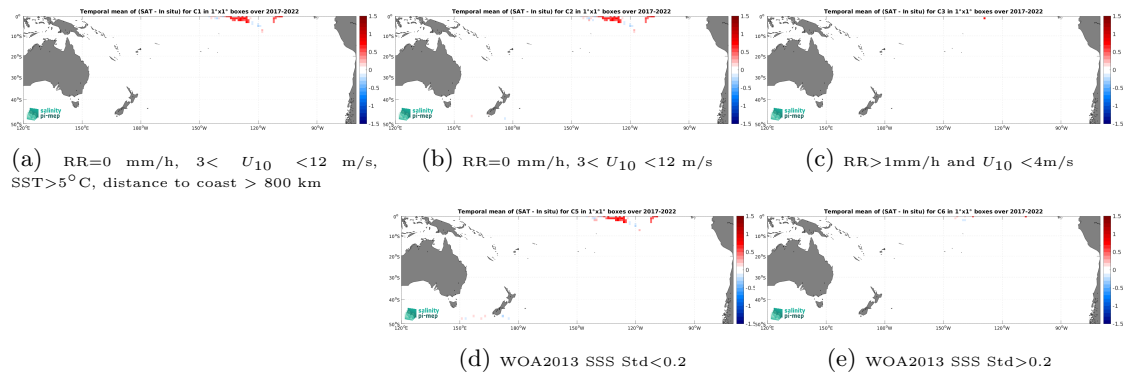
Figure 12: Temporal mean gridded over spatial boxes of size 1^\circ \times 1^\circ of \Delta SSS (CCI SSS L4 Merged-OI v4.4 - 30-day running (ESA) - Saildrone) for 5 different subdatasets corresponding to:RR=0 mm/h, 3 < U_{10} < 12 m/s, SST >5^\circ\text{C} , distance to coast > 800 km (a), RR=0 mm/h, 3 < U_{10} < 12 m/s (b), RR >1 mm/h and U_{10} < 4 m/s (c), WOA2013 SSS Std <0.2 (d), WOA2013 SSS Std >0.2 (e).
