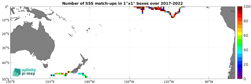
Figure 4: Number of SSS match-ups between Saildrone SSS and the CCI SSS L4 Merged-OI v4.4 - 30-day running (ESA) SSS product for the South Pacific Ocean Pi-MEP region over 1^\circ \times 1^\circ boxes and for the full satellite product period.
