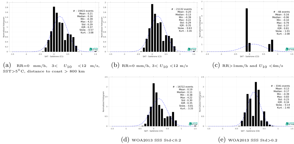
Figure 13: Normalized histogram of \Delta SSS (CCI SSS L4 Merged-OI v4.4 - 30-day running (ESA) - Saldrone) for 5 different subdatasets corresponding to: RR=0 mm/h, 3 < U_{10} < 12 m/s, SST > 5°C, distance to coast > 800 km (a), RR=0 mm/h, 3 < U_{10} < 12 m/s (b), RR > 1mm/h and U_{10} < 4 m/s (c), WOA2013 SSS Std < 0.2 (d), WOA2013 SSS Std > 0.2 (e).
