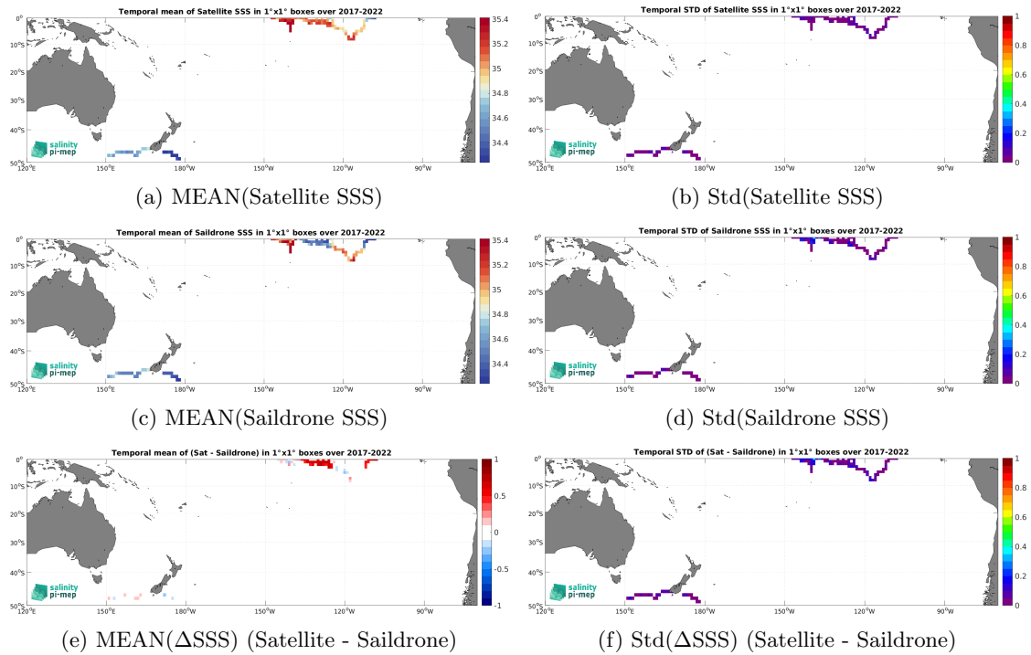
Figure 6: Temporal mean (left) and Std (right) of SSS from CCI SSS L4 Merged-OI v4.4 - 30-day running (ESA) (top), Saildrone (middle), and of \Delta SSS (Satellite - Saildrone). Only match-up pairs are used to generate these maps.
