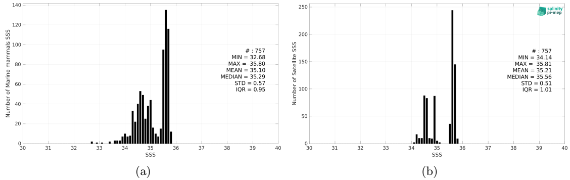
Figure 2: Histograms of SSS from Marine mammals (a) and CCI SSS L4 Merged-OI v4.4 - 30-day running (ESA) (b) considering all match-up pairs per bins of 0.1 over the South Pacific Ocean Pi-MEP region and for the full satellite product period.
