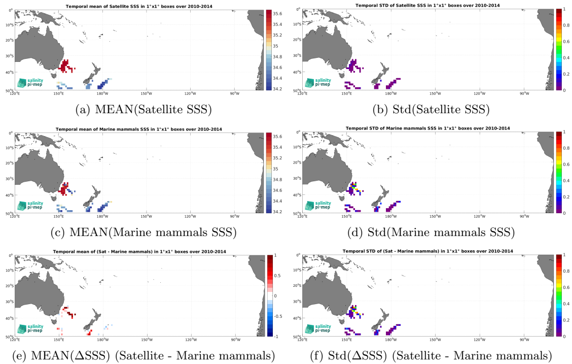
Figure 6: Temporal mean (left) and Std (right) of SSS from CCI SSS L4 Merged-OI v4.4 - 30-day running (ESA) (top), Marine mammals (middle), and of \Delta SSS (Satellite - Marine mammals). Only match-up pairs are used to generate these maps.
