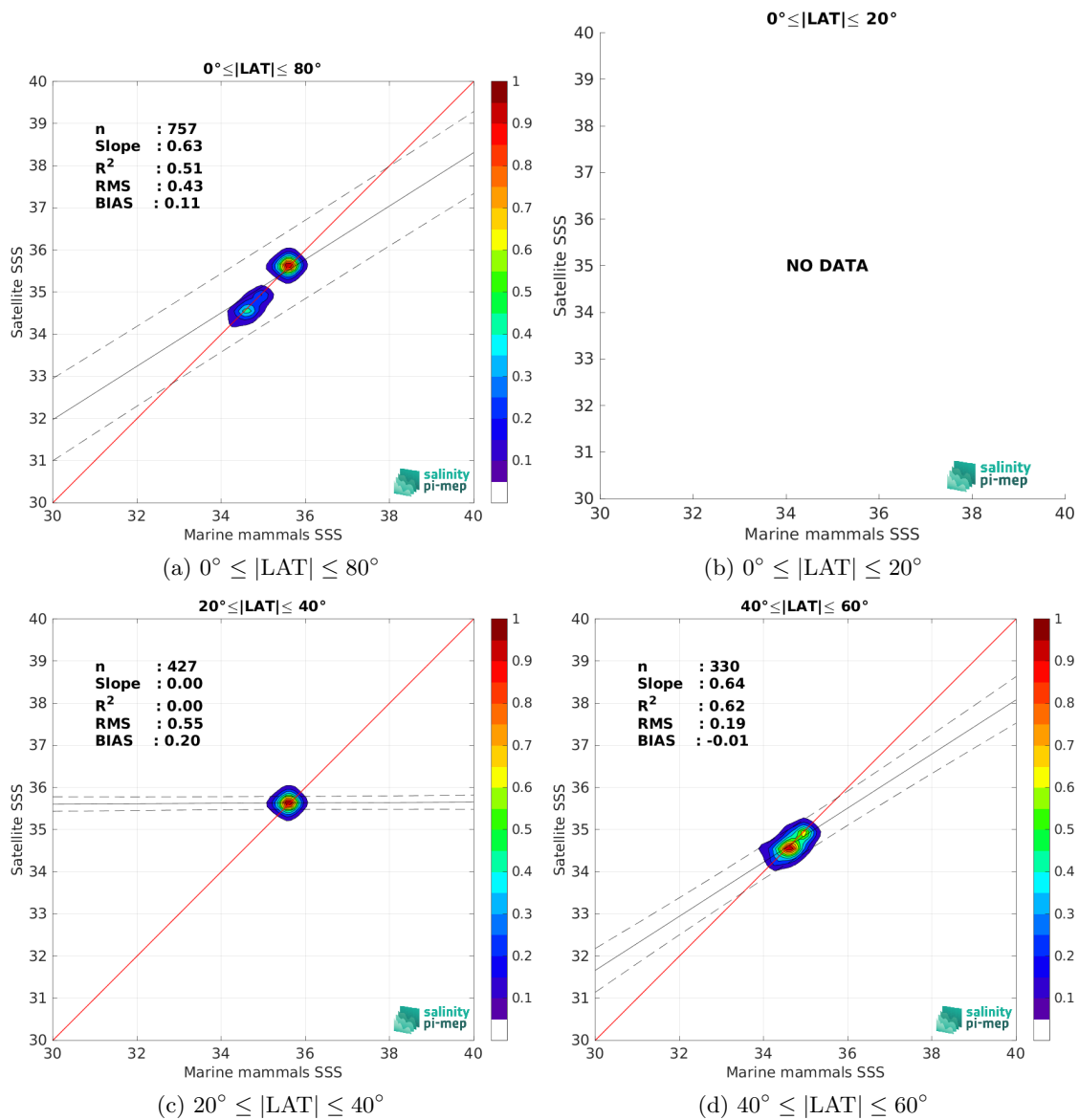
Figure 9: Contour maps of the concentration of CCI SSS L4 Merged-OI v4.4 - 30-day running (ESA) SSS (y-axis) versus Marine mammals SSS (x-axis) at match-up pairs for different latitude bands. For each plot, the red line shows x=y . The black thin and dashed lines indicate a linear fit through the data cloud and the \pm 95\% confidence levels, respectively. The number match-up pairs n , the slope and R^2 coefficient of the linear fit, the root mean square (RMS) and the mean bias between satellite and in situ data are indicated for each latitude band in each plots.
