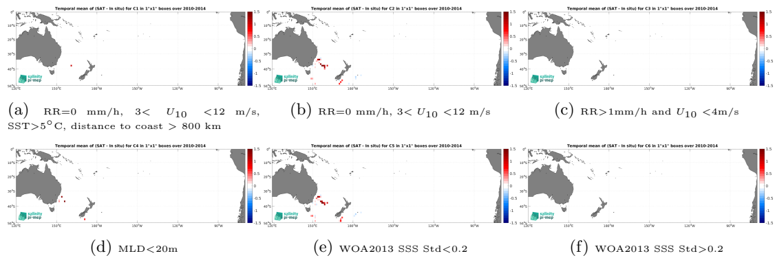
Figure 12: Temporal mean gridded over spatial boxes of size 1^\circ \times 1^\circ of \Delta SSS (CCI SSS L4 Merged-OI v4.4 - 30-day running (ESA) - Marine mammals) for 6 different subdatasets corresponding to:RR=0 mm/h, 3 < U_{10} < 12 m/s, SST >5^\circ C, distance to coast > 800 km (a), RR=0 mm/h, 3 < U_{10} < 12 m/s (b), RR >1 mm/h and U_{10} < 4 m/s (c),MLD <20 m (d),WOA2013 SSS Std <0.2 (e),WOA2013 SSS Std >0.2 (f).
