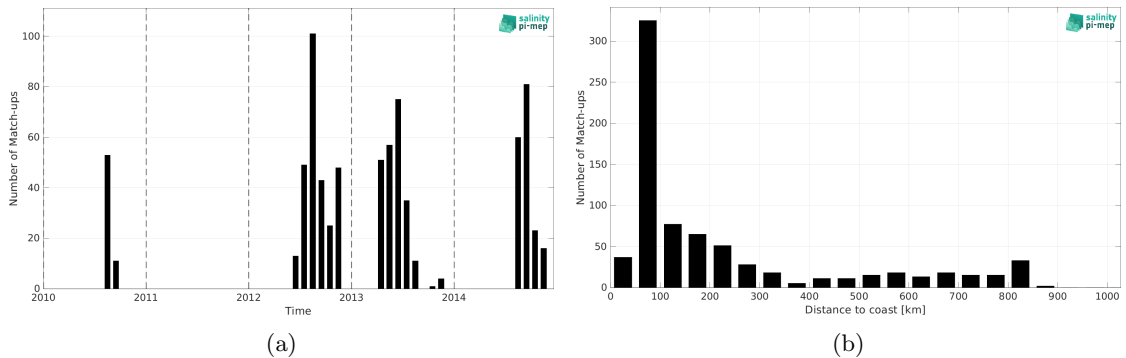
Figure 1: Number of match-ups between Marine mammals and CCI SSS L4 Merged-OI v4.4 - 30-day running (ESA) SSS as a function of time (a) and as function of the distance to coast (b) over the South Pacific Ocean Pi-MEP region and for the full satellite product period.
