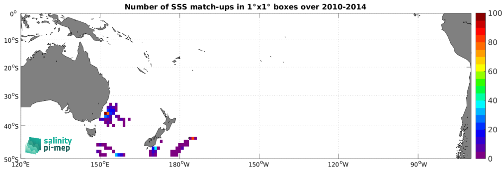
Figure 4: Number of SSS match-ups between Marine mammals SSS and the CCI SSS L4 Merged-OI v4.4 - 30-day running (ESA) SSS product for the South Pacific Ocean Pi-MEP region over 1^\circ \times 1^\circ boxes and for the full satellite product period.
