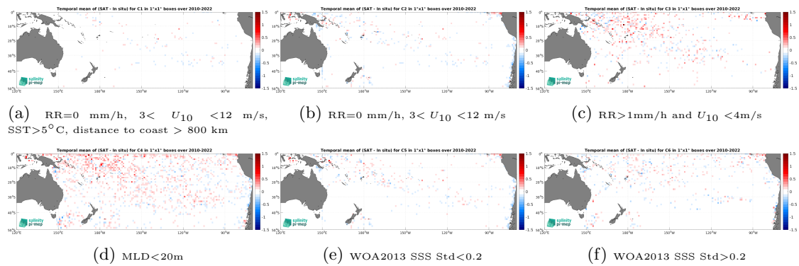
Figure 12: Temporal mean gridded over spatial boxes of size 1^\circ \times 1^\circ of \Delta SSS (CCI SSS L4 Merged-OI v4.4 - 30-day running (ESA) - Argo) for 6 different subdatasets corresponding to:RR=0 mm/h, 3 < U_{10} < 12 m/s, SST >5^\circ C, distance to coast > 800 km (a), RR=0 mm/h, 3 < U_{10} < 12 m/s (b), RR >1 mm/h and U_{10} < 4 m/s (c),MLD <20 m (d),WOA2013 SSS Std <0.2 (e),WOA2013 SSS Std >0.2 (f).
