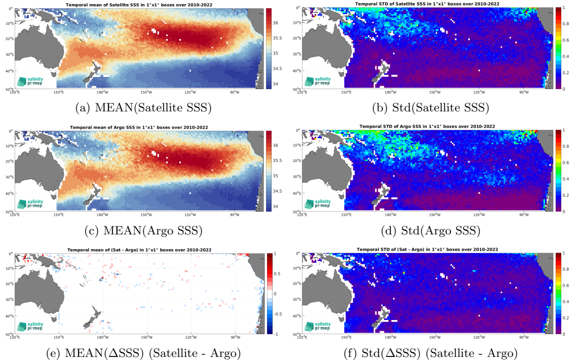
Figure 6: Temporal mean (left) and Std (right) of SSS from CCI SSS L4 Merged-OI v4.4 - 30-day running (ESA) (top), Argo (middle), and of \Delta SSS (Satellite - Argo). Only match-up pairs are used to generate these maps.
