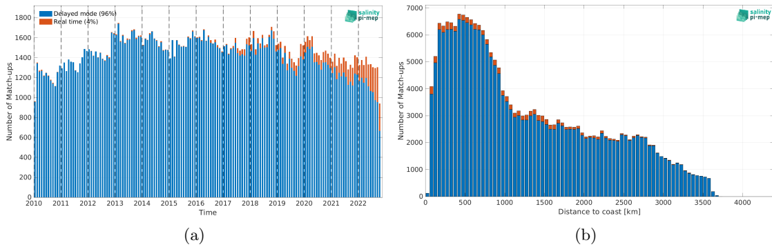
Figure 1: Number of match-ups between Argo and CCI SSS L4 Merged-OI v4.4 - 30-day running (ESA) SSS as a function of time (a) and as function of the distance to coast (b) over the South Pacific Ocean Pi-MEP region and for the full satellite product period.
