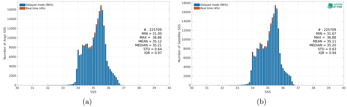
Figure 2: Histograms of SSS from Argo (a) and CCI SSS L4 Merged-OI v4.4 - 30-day running (ESA) (b) considering all match-up pairs per bins of 0.1 over the South Pacific Ocean Pi-MEP region and for the full satellite product period.
