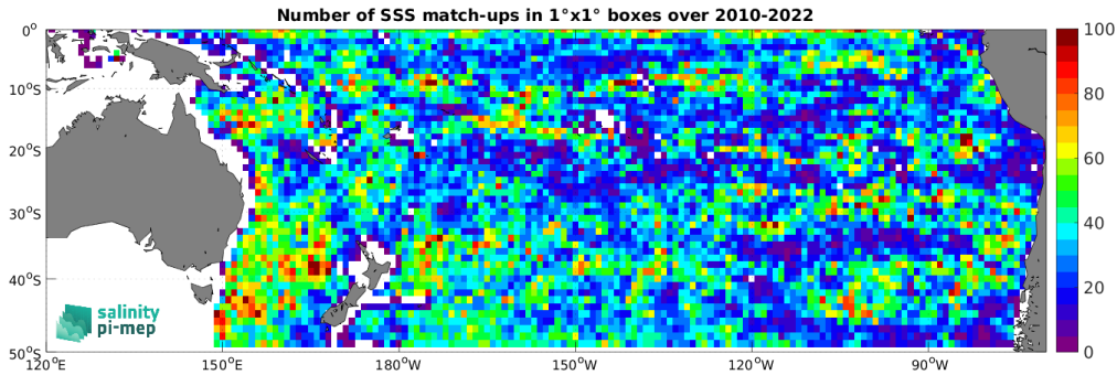
Figure 4: Number of SSS match-ups between Argo SSS and the CCI SSS L4 Merged-OI v4.4 - 30-day running (ESA) SSS product for the South Pacific Ocean Pi-MEP region over 1^\circ \times 1^\circ boxes and for the full satellite product period.
