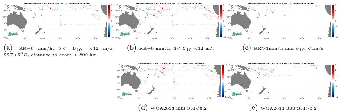
Figure 12: Temporal mean gridded over spatial boxes of size 1^\circ \times 1^\circ of \Delta\text{SSS} (CCI SSS L4 Merged-OI v3.2 - 7-day running (ESA) - TSG (SAMOS)) for 5 different subdatasets corresponding to:RR=0 mm/h, 3 < U_{10} < 12 m/s, SST >5^\circ\text{C} , distance to coast > 800 km (a), RR=0 mm/h, 3 < U_{10} < 12 m/s (b), RR >1 mm/h and U_{10} < 4 m/s (c), WOA2013 SSS Std <0.2 (d), WOA2013 SSS Std >0.2 (e).
