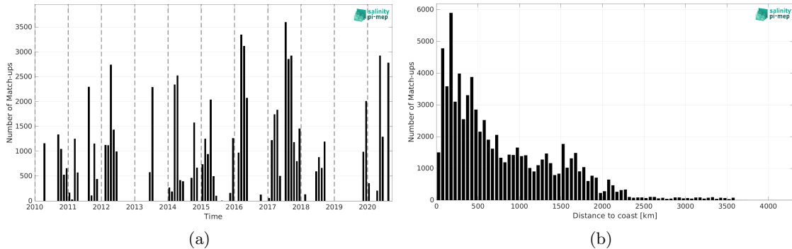
Figure 1: Number of match-ups between TSG (SAMOS) and CCI SSS L4 Merged-OI v3.2 - 7-day running (ESA) SSS as a function of time (a) and as function of the distance to coast (b) over the South Pacific Ocean Pi-MEP region and for the full satellite product period.
