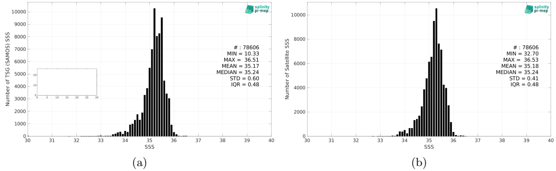
Figure 2: Histograms of SSS from TSG (SAMOS) (a) and CCI SSS L4 Merged-OI v3.2 - 7-day running (ESA) (b) considering all match-up pairs per bins of 0.1 over the South Pacific Ocean Pi-MEP region and for the full satellite product period.
