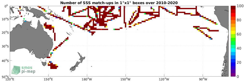
Figure 4: Number of SSS match-ups between TSG (SAMOS) SSS and the CCI SSS L4 Merged-OI v3.2 - 7-day running (ESA) SSS product for the South Pacific Ocean Pi-MEP region over 1^\circ \times 1^\circ boxes and for the full satellite product period.
