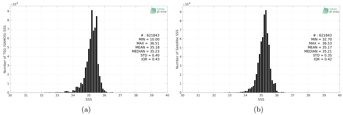
Figure 2: Histograms of SSS from TSG (SAMOS) (a) and CCI SSS L4 Merged-OI v3.2 - 7-day running (ESA) (b) considering all match-up pairs per bins of 0.1 over the South Pacific Ocean Pi-MEP region and for the full satellite product period.
