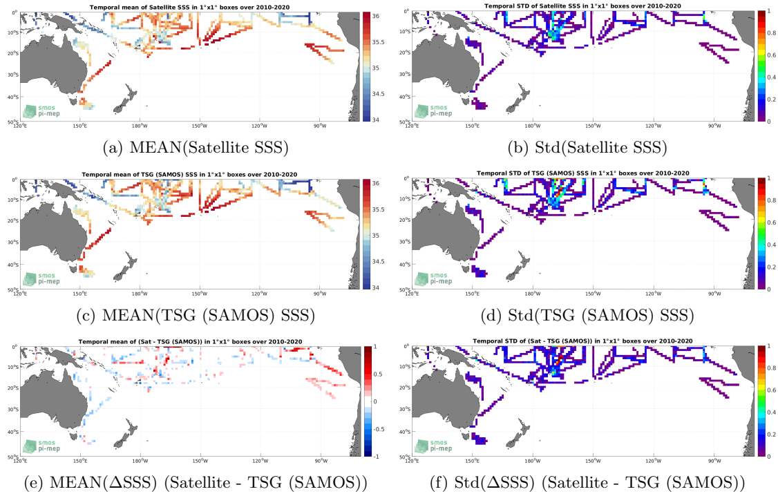
Figure 6: Temporal mean (left) and Std (right) of SSS from CCI SSS L4 Merged-OI v3.2 - 7-day running (ESA) (top), TSG (SAMOS) (middle), and of \Delta SSS (Satellite - TSG (SAMOS)). Only match-up pairs are used to generate these maps.
