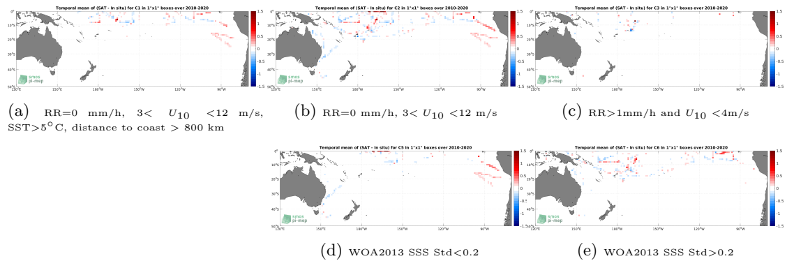
Figure 12: Temporal mean gridded over spatial boxes of size 1^\circ \times 1^\circ of \Delta SSS (CCI SSS L4 Merged-OI v3.2 - 7-day running (ESA) - TSG (SAMOS)) for 5 different subdatasets corresponding to:RR=0 mm/h, 3 < U_{10} < 12 m/s, SST >5^\circ C, distance to coast > 800 km (a), RR=0 mm/h, 3 < U_{10} < 12 m/s (b), RR >1 mm/h and U_{10} < 4 m/s (c), WOA2013 SSS Std <0.2 (d), WOA2013 SSS Std >0.2 (e).
