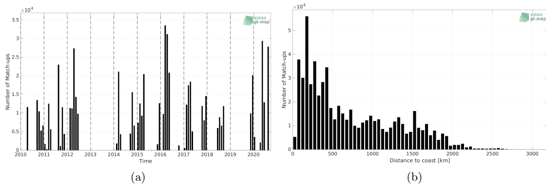
Figure 1: Number of match-ups between TSG (SAMOS) and CCI SSS L4 Merged-OI v3.2 - 7-day running (ESA) SSS as a function of time (a) and as function of the distance to coast (b) over the South Pacific Ocean Pi-MEP region and for the full satellite product period.
