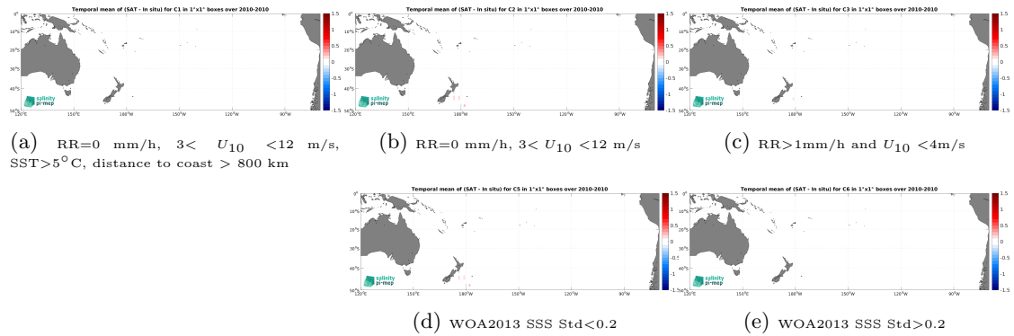
Figure 12: Temporal mean gridded over spatial boxes of size 1^{\circ}\times 1^{\circ} of \Delta\text{SSS} (CCI SSS L4 Merged-OI v3.2 - 7-day running (ESA) - TSG (Polarstern)) for 5 different subdatasets corresponding to:RR=0 mm/h, 3 < U_{10} < 12 m/s, SST > 5^{\circ}\text{C} , distance to coast > 800 km (a), RR=0 mm/h, 3 < U_{10} < 12 m/s (b), RR > 1 mm/h and U_{10} < 4 m/s (c), WOA2013 SSS Std < 0.2 (d), WOA2013 SSS Std > 0.2 (e).
