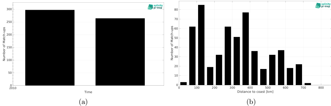
Figure 1: Number of match-ups between TSG (Polarstern) and CCI SSS L4 Merged-OI v3.2 - 7-day running (ESA) SSS as a function of time (a) and as function of the distance to coast (b) over the South Pacific Ocean Pi-MEP region and for the full satellite product period.
