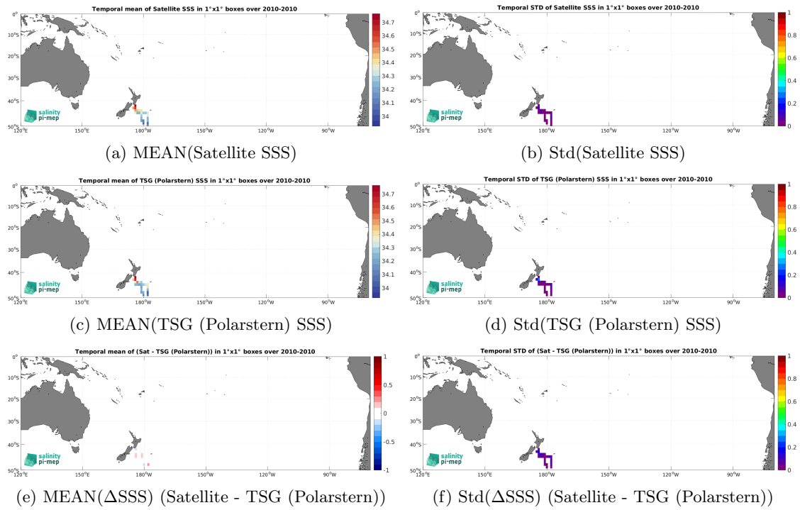
Figure 6: Temporal mean (left) and Std (right) of SSS from CCI SSS L4 Merged-OI v3.2 - 7-day running (ESA) (top), TSG (Polarstern) (middle), and of \Delta SSS (Satellite - TSG (Polarstern)). Only match-up pairs are used to generate these maps.
