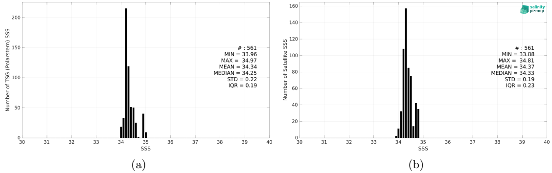
Figure 2: Histograms of SSS from TSG (Polarstern) (a) and CCI SSS L4 Merged-OI v3.2 - 7-day running (ESA) (b) considering all match-up pairs per bins of 0.1 over the South Pacific Ocean Pi-MEP region and for the full satellite product period.
