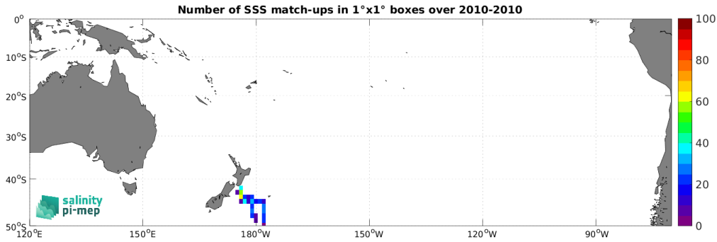
Figure 4: Number of SSS match-ups between TSG (Polarstern) SSS and the CCI SSS L4 Merged-OI v3.2 - 7-day running (ESA) SSS product for the South Pacific Ocean Pi-MEP region over 1^\circ \times 1^\circ boxes and for the full satellite product period.
