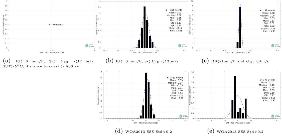
Figure 13: Normalized histogram of \Delta SSS (CCI SSS L4 Merged-OI v3.2 - 7-day running (ESA) - TSG (Polarstern)) for 5 different subdatasets corresponding to: RR=0 mm/h, 3 < U_{10} < 12 m/s, SST > 5°C, distance to coast > 800 km (a), RR=0 mm/h, 3 < U_{10} < 12 m/s (b), RR > 1mm/h and U_{10} < 4 m/s (c), WOA2013 SSS Std < 0.2 (d), WOA2013 SSS Std > 0.2 (e).
