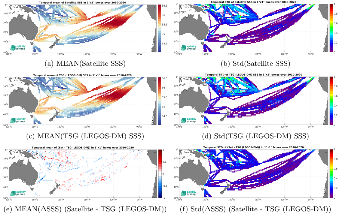
Figure 6: Temporal mean (left) and Std (right) of SSS from CCI SSS L4 Merged-OI v3.2 - 7-day running (ESA) (top), TSG (LEGOS-DM) ( in situ dataset) (middle), and of \Delta\text{SSS} (Satellite - TSG (LEGOS-DM)). Only match-up pairs are used to generate these maps.
