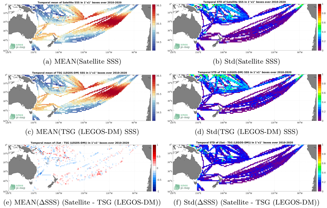
Figure 6: Temporal mean (left) and Std (right) of SSS from CCI SSS L4 Merged-OI v3.2 - 7-day running (ESA) (top), TSG (LEGOS-DM) (middle), and of \Delta\text{SSS} (Satellite - TSG (LEGOS-DM)). Only match-up pairs are used to generate these maps.
