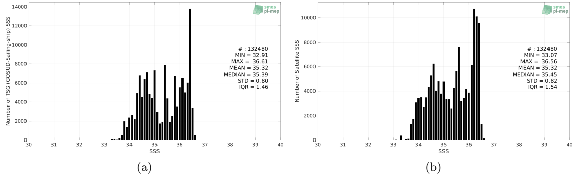
Figure 2: Histograms of SSS from TSG (GOSUD-Sailing-ship) (a) and CCI SSS L4 Merged-OI v3.2 - 7-day running (ESA) (b) considering all match-up pairs per bins of 0.1 over the South Pacific Ocean Pi-MEP region and for the full satellite product period.
