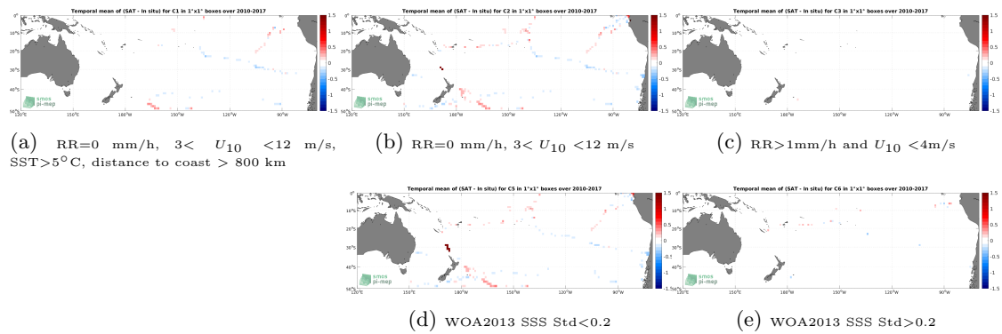
Figure 12: Temporal mean gridded over spatial boxes of size 1^\circ \times 1^\circ of \Delta SSS (CCI SSS L4 Merged-OI v3.2 - 7-day running (ESA) - TSG (GOSUD-Sailing-ship)) for 5 different subdatasets corresponding to:RR=0 mm/h, 3 < U_{10} < 12 m/s, SST >5^\circ\text{C} , distance to coast > 800 km (a), RR=0 mm/h, 3 < U_{10} < 12 m/s (b), RR >1 mm/h and U_{10} < 4 m/s (c), WOA2013 SSS Std <0.2 (d), WOA2013 SSS Std >0.2 (e).
