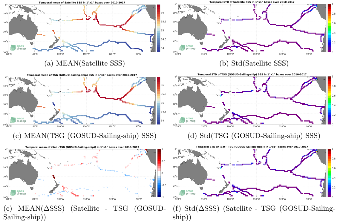
Figure 6: Temporal mean (left) and Std (right) of SSS from CCI SSS L4 Merged-OI v3.2 - 7-day running (ESA) (top), TSG (GOSUD-Sailing-ship) (middle), and of \Delta SSS (Satellite - TSG (GOSUD-Sailing-ship)). Only match-up pairs are used to generate these maps.
