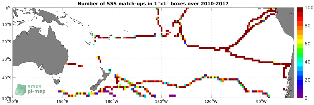
Figure 4: Number of SSS match-ups between TSG (GOSUD-Sailing-ship) SSS and the CCI SSS L4 Merged-OI v3.2 - 7-day running (ESA) SSS product for the South Pacific Ocean Pi-MEP region over 1^\circ \times 1^\circ boxes and for the full satellite product period.
