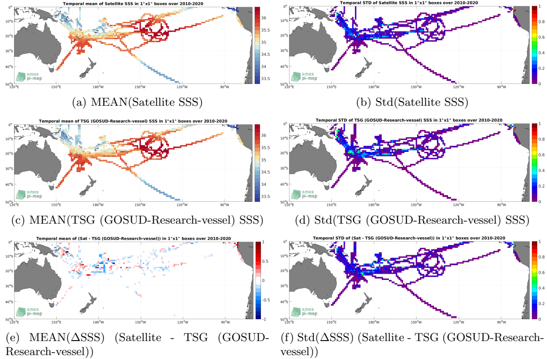
Figure 6: Temporal mean (left) and Std (right) of SSS from CCI SSS L4 Merged-OI v3.2 - 7-day running (ESA) (top), TSG (GOSUD-Research-vessel) (middle), and of \Delta SSS (Satellite - TSG (GOSUD-Research-vessel)). Only match-up pairs are used to generate these maps.
