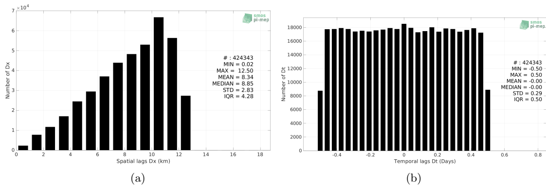
Figure 5: Histograms of the spatial (a) and temporal (b) lags between the location/time of the TSG (GOSUD-Research-vessel) measurement and the date of the corresponding CCI SSS L4 Merged-OI v3.2 - 7-day running (ESA) SSS pixel.
