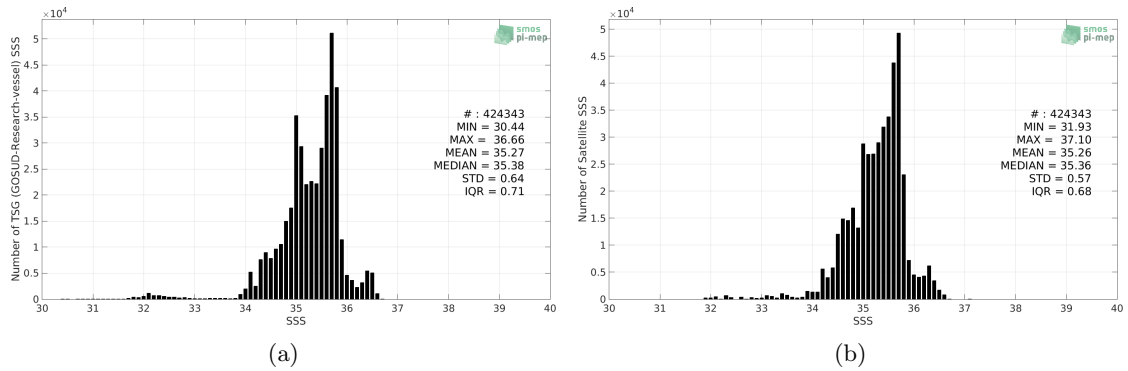
Figure 2: Histograms of SSS from TSG (GOSUD-Research-vessel) (a) and CCI SSS L4 Merged-OI v3.2 - 7-day running (ESA) (b) considering all match-up pairs per bins of 0.1 over the South Pacific Ocean Pi-MEP region and for the full satellite product period.
