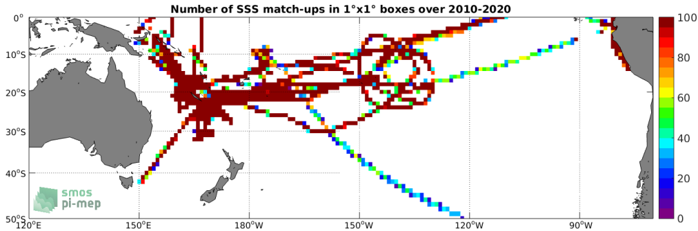
Figure 4: Number of SSS match-ups between TSG (GOSUD-Research-vessel) SSS and the CCI SSS L4 Merged-OI v3.2 - 7-day running (ESA) SSS product for the South Pacific Ocean Pi-MEP region over 1^\circ \times 1^\circ boxes and for the full satellite product period.
