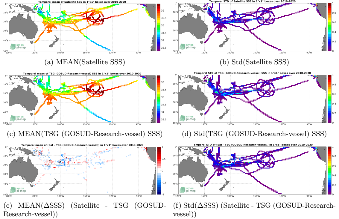
Figure 6: Temporal mean (left) and Std (right) of SSS from CCI SSS L4 Merged-OI v3.2 - 7-day running (ESA) (top), TSG (GOSUD-Research-vessel) (middle), and of \Delta SSS (Satellite - TSG (GOSUD-Research-vessel)). Only match-up pairs are used to generate these maps.
