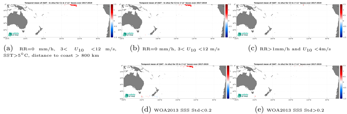
Figure 12: Temporal mean gridded over spatial boxes of size 1^\circ \times 1^\circ of \Delta SSS (CCI SSS L4 Merged-OI v3.2 - 7-day running (ESA) - Sairdrone) for 5 different subdatasets corresponding to:RR=0 mm/h, 3 < U_{10} < 12 m/s, SST >5^\circ C, distance to coast > 800 km (a), RR=0 mm/h, 3 < U_{10} < 12 m/s (b), RR >1 mm/h and U_{10} < 4 m/s (c), WOA2013 SSS Std <0.2 (d), WOA2013 SSS Std >0.2 (e).
