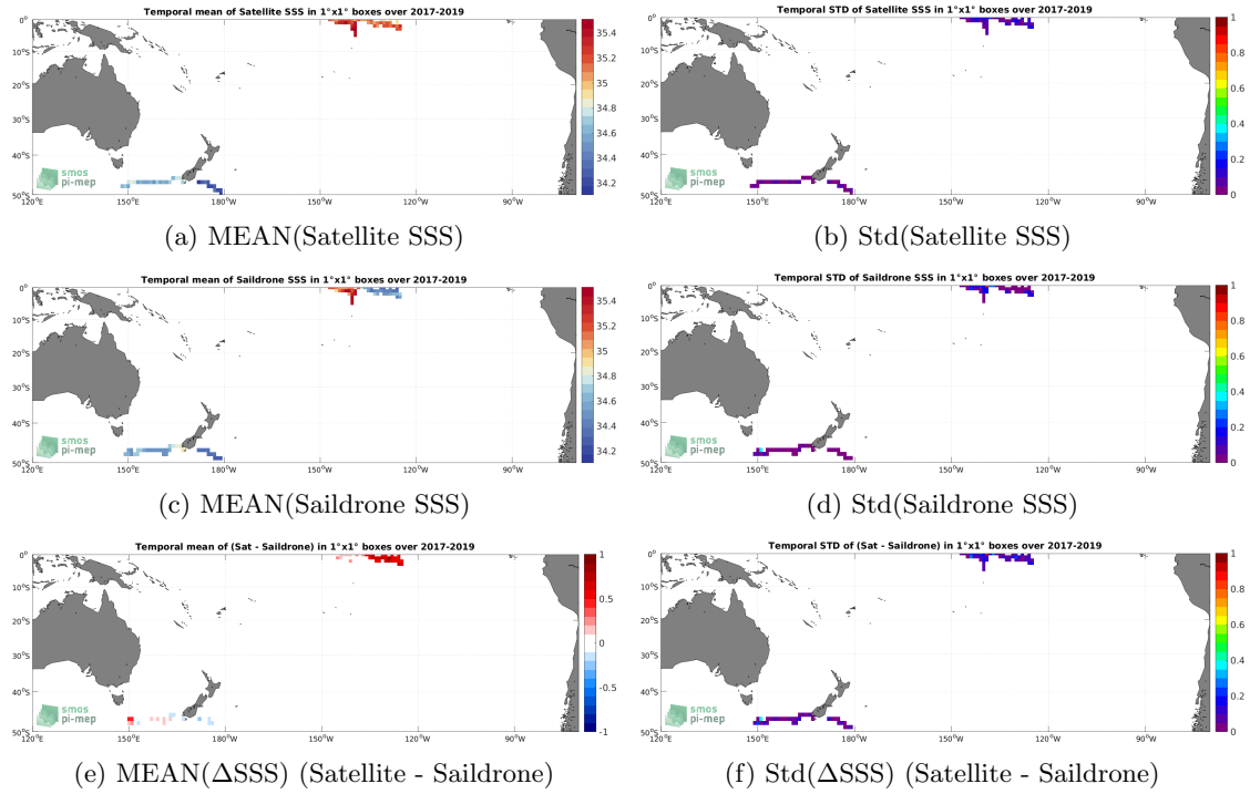
Figure 6: Temporal mean (left) and Std (right) of SSS from CCI SSS L4 Merged-OI v3.2 - 7-day running (ESA) (top), Saildrone (middle), and of \Delta SSS (Satellite - Saildrone). Only match-up pairs are used to generate these maps.
