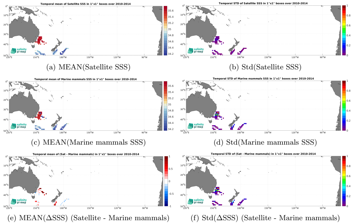
Figure 6: Temporal mean (left) and Std (right) of SSS from CCI SSS L4 Merged-OI v3.2 - 7-day running (ESA) (top), Marine mammals (middle), and of \Delta SSS (Satellite - Marine mammals). Only match-up pairs are used to generate these maps.
