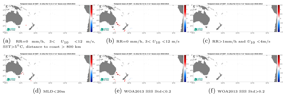
Figure 12: Temporal mean gridded over spatial boxes of size 1^\circ \times 1^\circ of \Delta SSS (CCI SSS L4 Merged-OI v3.2 - 7-day running (ESA) - Marine mammals) for 6 different subdatasets corresponding to:RR=0 mm/h, 3 < U_{10} < 12 m/s, SST >5^\circ C, distance to coast > 800 km (a), RR=0 mm/h, 3 < U_{10} < 12 m/s (b), RR >1 mm/h and U_{10} < 4 m/s (c),MLD <20 m (d),WOA2013 SSS Std <0.2 (e),WOA2013 SSS Std >0.2 (f).
