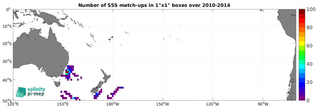
Figure 4: Number of SSS match-ups between Marine mammals SSS and the CCI SSS L4 Merged-OI v3.2 - 7-day running (ESA) SSS product for the South Pacific Ocean Pi-MEP region over 1^\circ \times 1^\circ boxes and for the full satellite product period.
