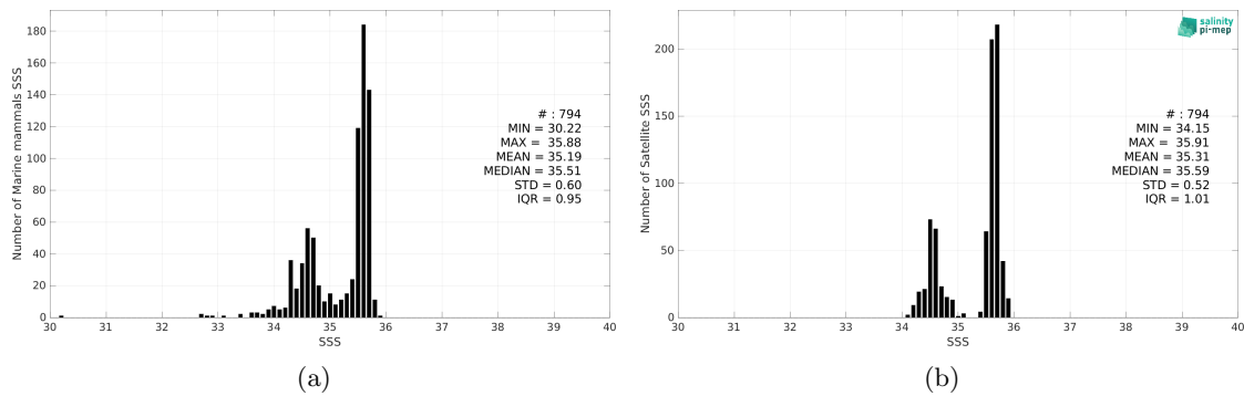
Figure 2: Histograms of SSS from Marine mammals (a) and CCI SSS L4 Merged-OI v3.2 - 7-day running (ESA) (b) considering all match-up pairs per bins of 0.1 over the South Pacific Ocean Pi-MEP region and for the full satellite product period.
