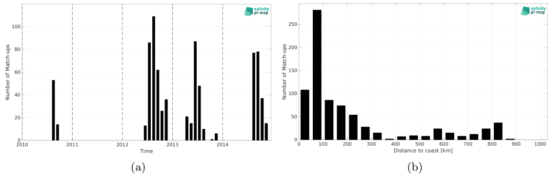
Figure 1: Number of match-ups between Marine mammals and CCI SSS L4 Merged-OI v3.2 - 7-day running (ESA) SSS as a function of time (a) and as function of the distance to coast (b) over the South Pacific Ocean Pi-MEP region and for the full satellite product period.
