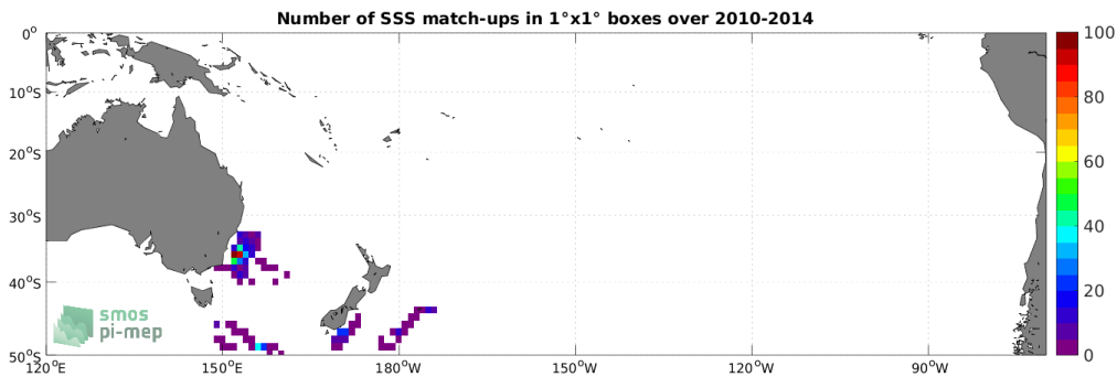
Figure 4: Number of SSS match-ups between Marine mammals SSS and the CCI SSS L4 Merged-OI v3.2 - 7-day running (ESA) SSS product for the South Pacific Ocean Pi-MEP region over 1°×1° boxes and for the full satellite product period.
