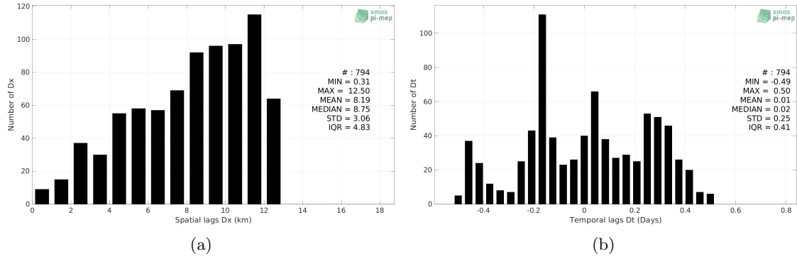
Figure 5: Histograms of the spatial (a) and temporal (b) lags between the location/time of the Marine mammals measurement and the date of the corresponding CCI SSS L4 Merged-OI v3.2 - 7-day running (ESA) SSS pixel.
