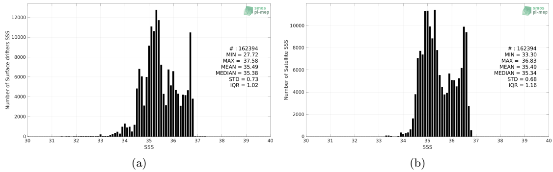
Figure 2: Histograms of SSS from Surface drifters (a) and CCI SSS L4 Merged-OI v3.2 - 7-day running (ESA) (b) considering all match-up pairs per bins of 0.1 over the South Pacific Ocean Pi-MEP region and for the full satellite product period.
