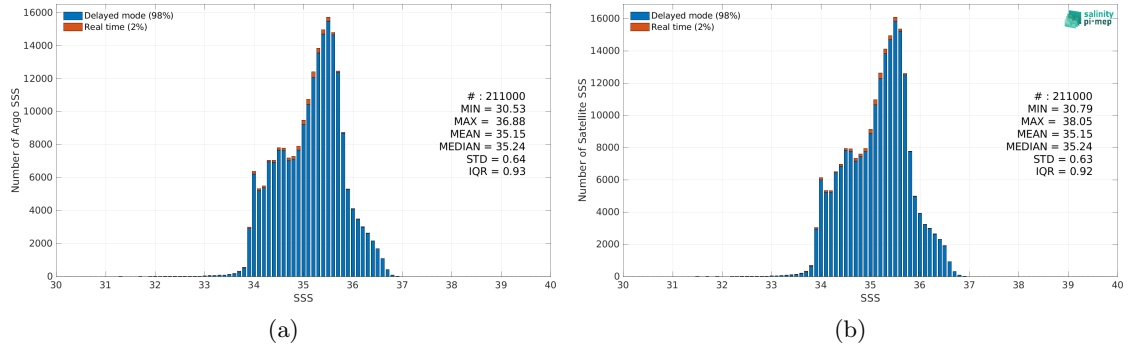
Figure 2: Histograms of SSS from Argo (a) and CCI SSS L4 Merged-OI v3.2 - 7-day running (ESA) (b) considering all match-up pairs per bins of 0.1 over the South Pacific Ocean Pi-MEP region and for the full satellite product period.
