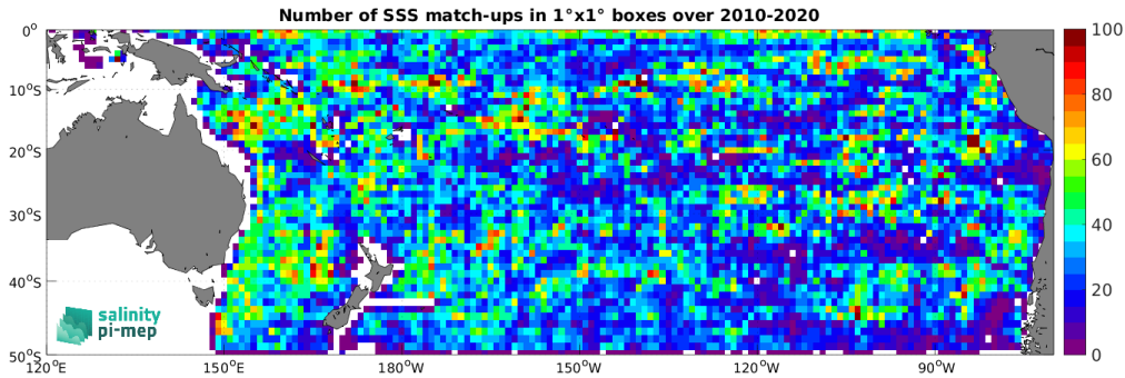
Figure 4: Number of SSS match-ups between Argo SSS and the CCI SSS L4 Merged-OI v3.2 - 7-day running (ESA) SSS product for the South Pacific Ocean Pi-MEP region over 1^\circ \times 1^\circ boxes and for the full satellite product period.
