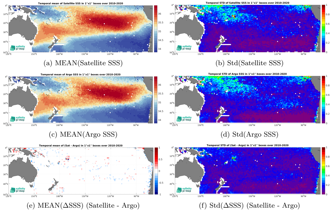
Figure 6: Temporal mean (left) and Std (right) of SSS from CCI SSS L4 Merged-OI v3.2 - 7-day running (ESA) (top), Argo (middle), and of \Delta SSS (Satellite - Argo). Only match-up pairs are used to generate these maps.
