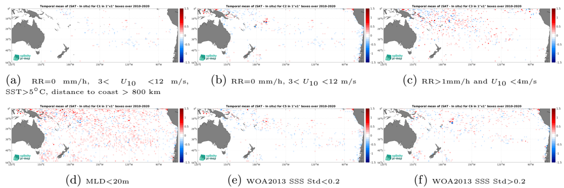
Figure 12: Temporal mean gridded over spatial boxes of size 1^\circ \times 1^\circ of \Delta SSS (CCI SSS L4 Merged-OI v3.2 - 7-day running (ESA) - Argo) for 6 different subdatasets corresponding to:RR=0 mm/h, 3 < U_{10} < 12 m/s, SST >5^\circ\text{C} , distance to coast > 800 km (a), RR=0 mm/h, 3 < U_{10} < 12 m/s (b), RR >1 mm/h and U_{10} < 4 m/s (c),MLD <20 m (d),WOA2013 SSS Std <0.2 (e),WOA2013 SSS Std >0.2 (f).
