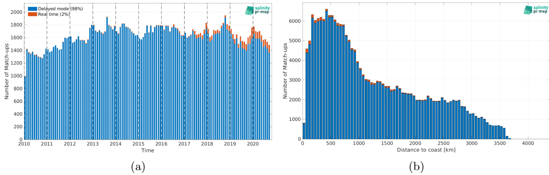
Figure 1: Number of match-ups between Argo and CCI SSS L4 Merged-OI v3.2 - 7-day running (ESA) SSS as a function of time (a) and as function of the distance to coast (b) over the South Pacific Ocean Pi-MEP region and for the full satellite product period.
