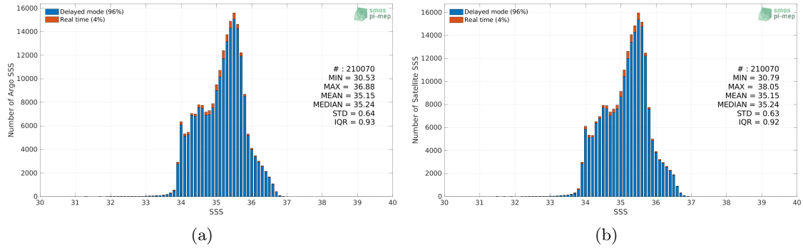
Figure 2: Histograms of SSS from Argo (a) and CCI SSS L4 Merged-OI v3.2 - 7-day running (ESA) (b) considering all match-up pairs per bins of 0.1 over the South Pacific Ocean Pi-MEP region and for the full satellite product period.
