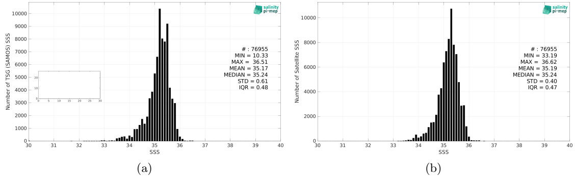
Figure 2: Histograms of SSS from TSG (SAMOS) (a) and CCI SSS L4 Merged-OI v3.2 - 30-day running (ESA) (b) considering all match-up pairs per bins of 0.1 over the South Pacific Ocean Pi-MEP region and for the full satellite product period.
