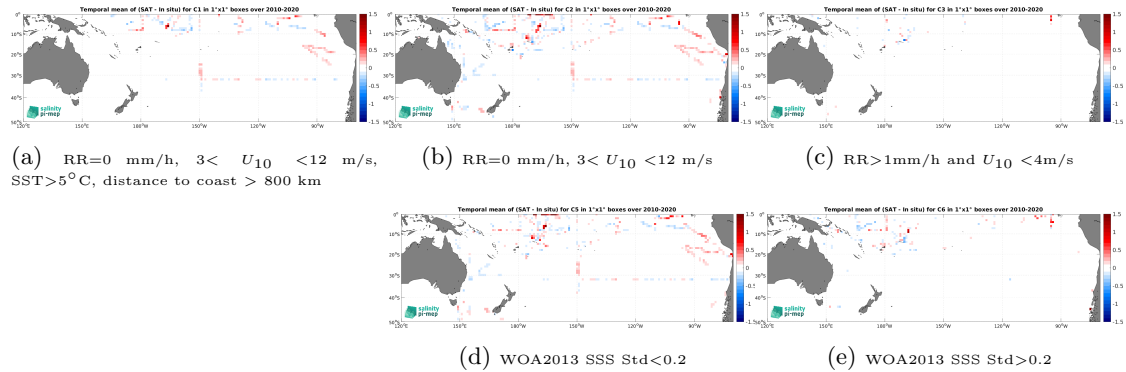
Figure 12: Temporal mean gridded over spatial boxes of size 1^\circ \times 1^\circ of \Delta\text{SSS} (CCI SSS L4 Merged-OI v3.2 - 30-day running (ESA) - TSG (SAMOS)) for 5 different subdatasets corresponding to:RR=0 mm/h, 3 < U_{10} < 12 m/s, SST >5^\circ\text{C} , distance to coast > 800 km (a), RR=0 mm/h, 3 < U_{10} < 12 m/s (b), RR >1 mm/h and U_{10} < 4 m/s (c), WOA2013 SSS Std <0.2 (d), WOA2013 SSS Std >0.2 (e).
