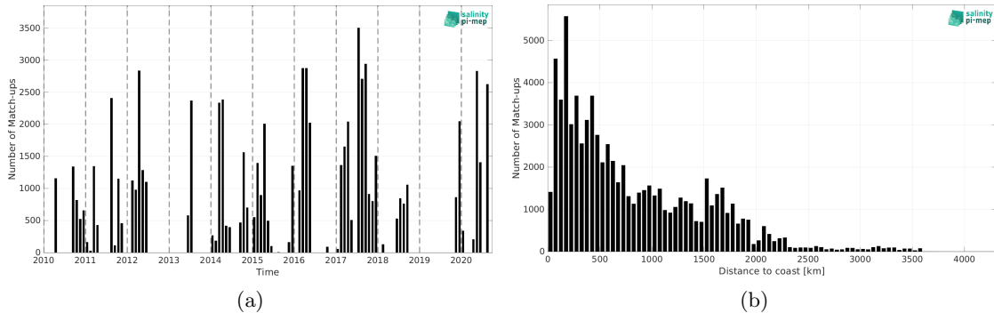
Figure 1: Number of match-ups between TSG (SAMOS) and CCI SSS L4 Merged-OI v3.2 - 30-day running (ESA) SSS as a function of time (a) and as function of the distance to coast (b) over the South Pacific Ocean Pi-MEP region and for the full satellite product period.
