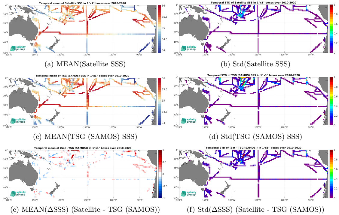
Figure 6: Temporal mean (left) and Std (right) of SSS from CCI SSS L4 Merged-OI v3.2 - 30-day running (ESA) (top), TSG (SAMOS) (middle), and of \Delta SSS (Satellite - TSG (SAMOS)). Only match-up pairs are used to generate these maps.
