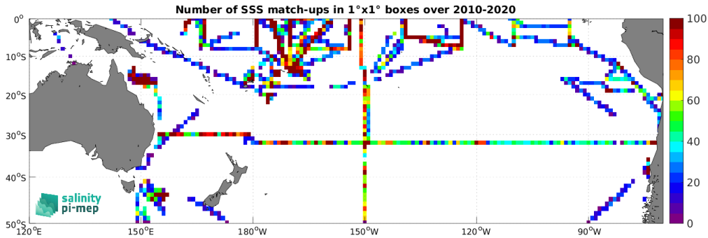
Figure 4: Number of SSS match-ups between TSG (SAMOS) SSS and the CCI SSS L4 Merged-OI v3.2 - 30-day running (ESA) SSS product for the South Pacific Ocean Pi-MEP region over 1^\circ \times 1^\circ boxes and for the full satellite product period.
