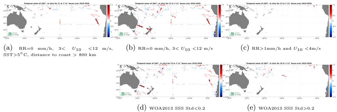
Figure 12: Temporal mean gridded over spatial boxes of size 1^\circ \times 1^\circ of \Delta SSS (CCI SSS L4 Merged-OI v3.2 - 30-day running (ESA) - TSG (SAMOS)) for 5 different subdatasets corresponding to:RR=0 mm/h, 3 < U_{10} < 12 m/s, SST >5^\circ C, distance to coast > 800 km (a), RR=0 mm/h, 3 < U_{10} < 12 m/s (b), RR >1 mm/h and U_{10} < 4 m/s (c), WOA2013 SSS Std <0.2 (d), WOA2013 SSS Std >0.2 (e).
