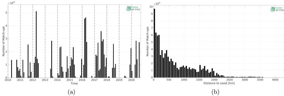
Figure 1: Number of match-ups between TSG (SAMOS) and CCI SSS L4 Merged-OI v3.2 - 30-day running (ESA) SSS as a function of time (a) and as function of the distance to coast (b) over the South Pacific Ocean Pi-MEP region and for the full satellite product period.
