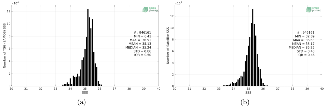
Figure 2: Histograms of SSS from TSG (SAMOS) (a) and CCI SSS L4 Merged-OI v3.2 - 30-day running (ESA) (b) considering all match-up pairs per bins of 0.1 over the South Pacific Ocean Pi-MEP region and for the full satellite product period.
