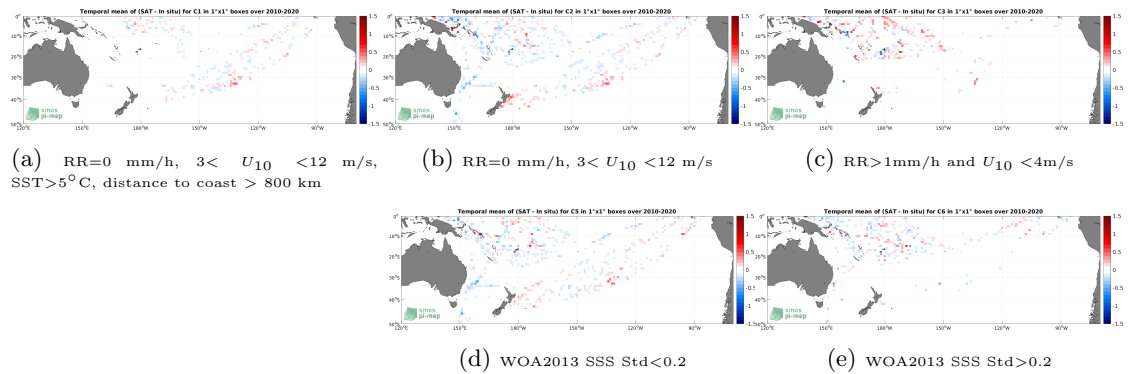
Figure 12: Temporal mean gridded over spatial boxes of size 1^\circ \times 1^\circ of \Delta SSS (CCI SSS L4 Merged-OI v3.2 - 30-day running (ESA) - TSG (LEGOS-DM)) for 5 different subdatasets corresponding to:RR=0 mm/h, 3 < U_{10} < 12 m/s, SST >5^\circ C, distance to coast > 800 km (a), RR=0 mm/h, 3 < U_{10} < 12 m/s (b), RR >1 mm/h and U_{10} < 4 m/s (c), WOA2013 SSS Std <0.2 (d), WOA2013 SSS Std >0.2 (e).
