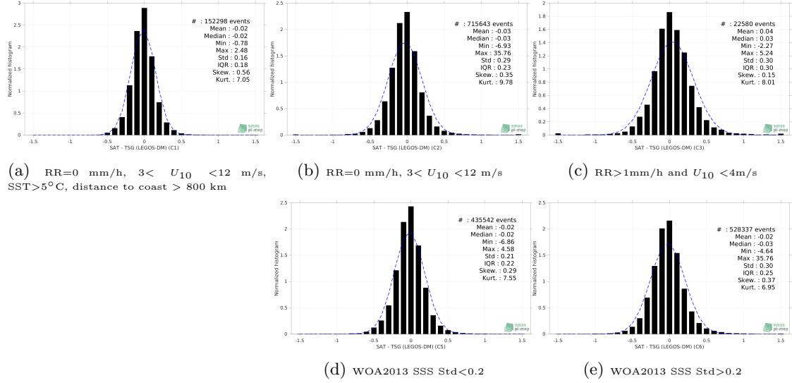
Figure 13: Normalized histogram of \Delta\text{SSS} (CCI SSS L4 Merged-OI v3.2 - 30-day running (ESA) - TSG (LEGOS-DM)) for 5 different subdatasets corresponding to: RR=0 mm/h, 3 < U_{10} < 12 m/s, SST >5^\circ\text{C} , distance to coast > 800 km (a), RR=0 mm/h, 3 < U_{10} < 12 m/s (b), RR >1 mm/h and U_{10} < 4 m/s (c), WOA2013 SSS Std <0.2 (d), WOA2013 SSS Std >0.2 (e).
