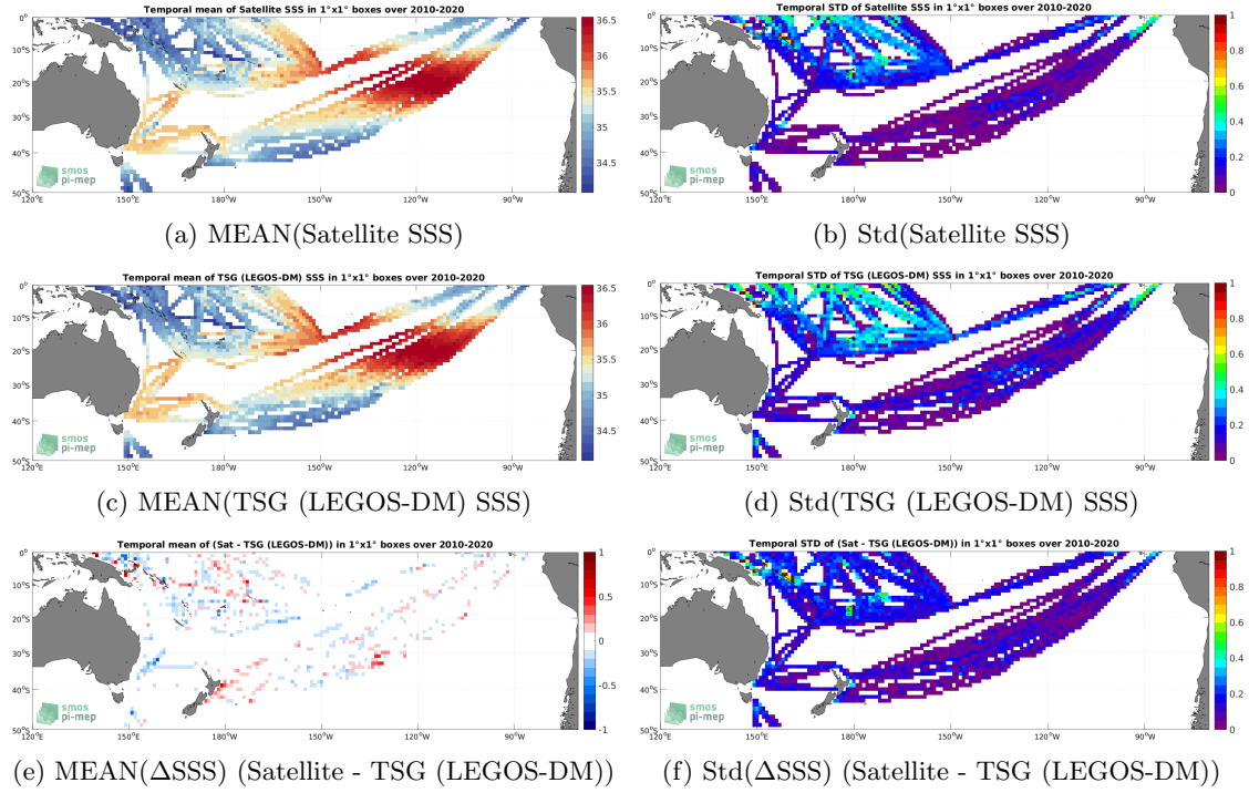
Figure 6: Temporal mean (left) and Std (right) of SSS from CCI SSS L4 Merged-OI v3.2 - 30-day running (ESA) (top), TSG (LEGOS-DM) ( in situ ) dataset (middle), and of \Delta\text{SSS} (Satellite - TSG (LEGOS-DM)). Only match-up pairs are used to generate these maps.
