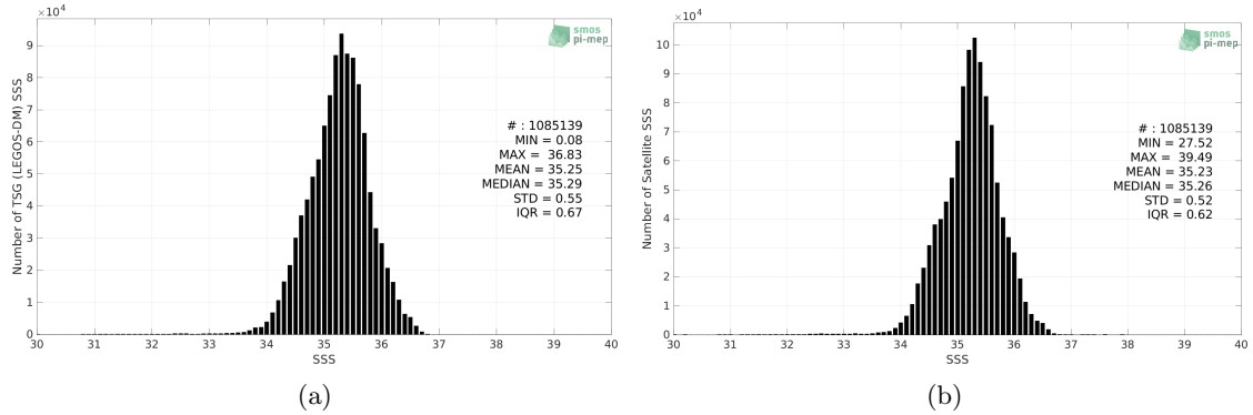
Figure 2: Histograms of SSS from TSG (LEGOS-DM) (a) and CCI SSS L4 Merged-OI v3.2 - 30-day running (ESA) (b) considering all match-up pairs per bins of 0.1 over the South Pacific Ocean Pi-MEP region and for the full satellite product period.
