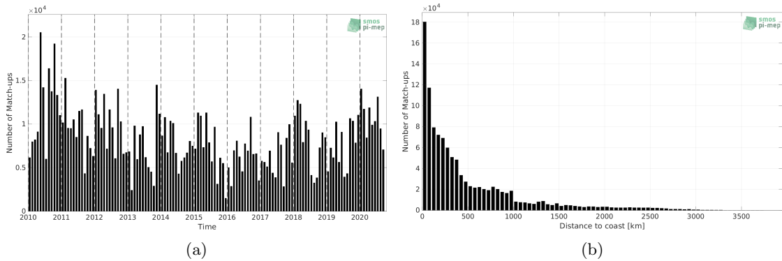
Figure 1: Number of match-ups between TSG (LEGOS-DM) and CCI SSS L4 Merged-OI v3.2 - 30-day running (ESA) SSS as a function of time (a) and as function of the distance to coast (b) over the South Pacific Ocean Pi-MEP region and for the full satellite product period.
