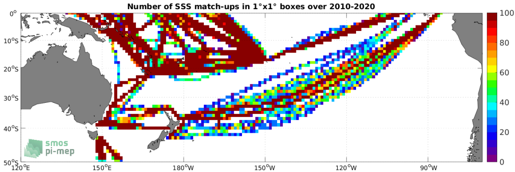
Figure 4: Number of SSS match-ups between TSG (LEGOS-DM) SSS and the CCI SSS L4 Merged-OI v3.2 - 30-day running (ESA) SSS product for the South Pacific Ocean Pi-MEP region over 1^\circ \times 1^\circ boxes and for the full satellite product period.
