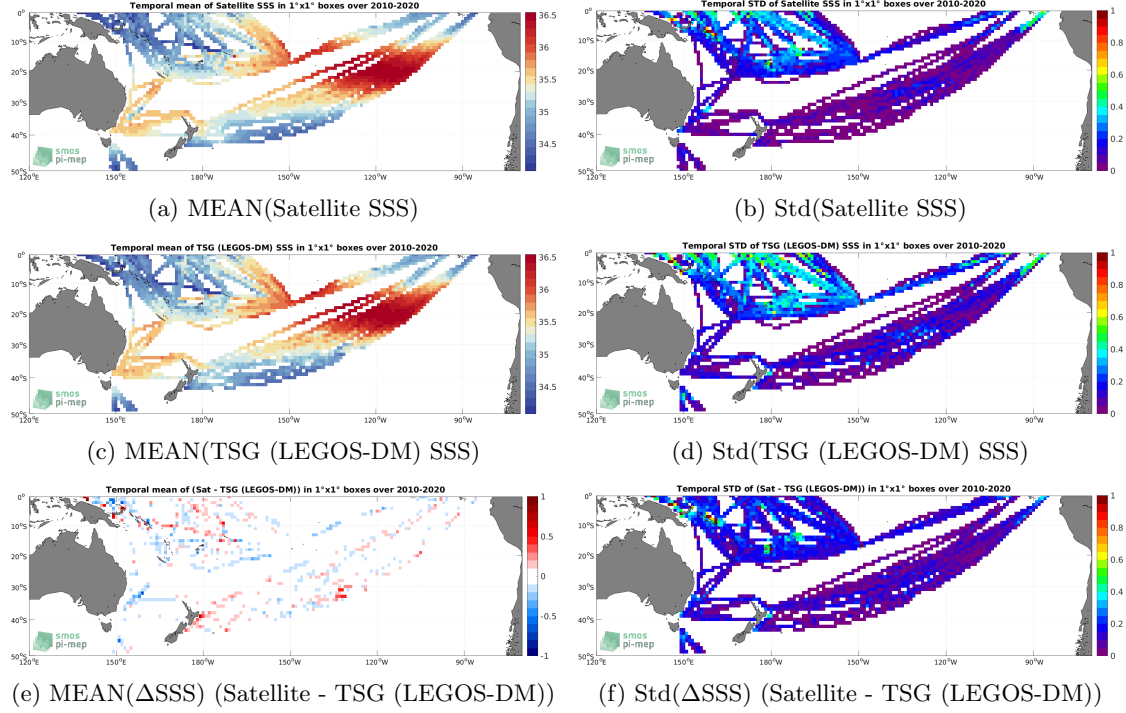
Figure 6: Temporal mean (left) and Std (right) of SSS from CCI SSS L4 Merged-OI v3.2 - 30-day running (ESA) (top), TSG (LEGOS-DM) (middle), and of \Delta SSS (Satellite - TSG (LEGOS-DM)). Only match-up pairs are used to generate these maps.
