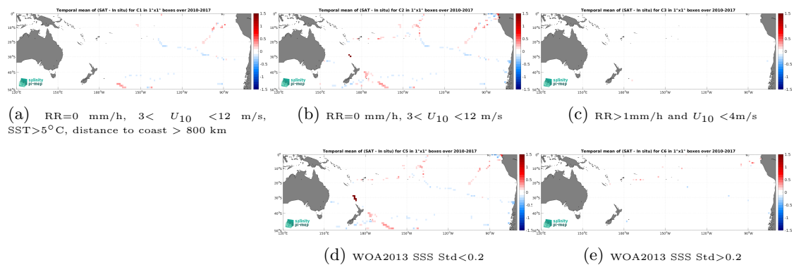
Figure 12: Temporal mean gridded over spatial boxes of size 1^\circ \times 1^\circ of \Delta\text{SSS} (CCI SSS L4 Merged-OI v3.2 - 30-day running (ESA) - TSG (GOSUD-Sailing-ship)) for 5 different subdatasets corresponding to:RR=0 mm/h, 3 < U_{10} < 12 m/s, SST >5^\circ\text{C} , distance to coast > 800 km (a), RR=0 mm/h, 3 < U_{10} < 12 m/s (b), RR >1 mm/h and U_{10} < 4 m/s (c), WOA2013 SSS Std <0.2 (d), WOA2013 SSS Std >0.2 (e).
