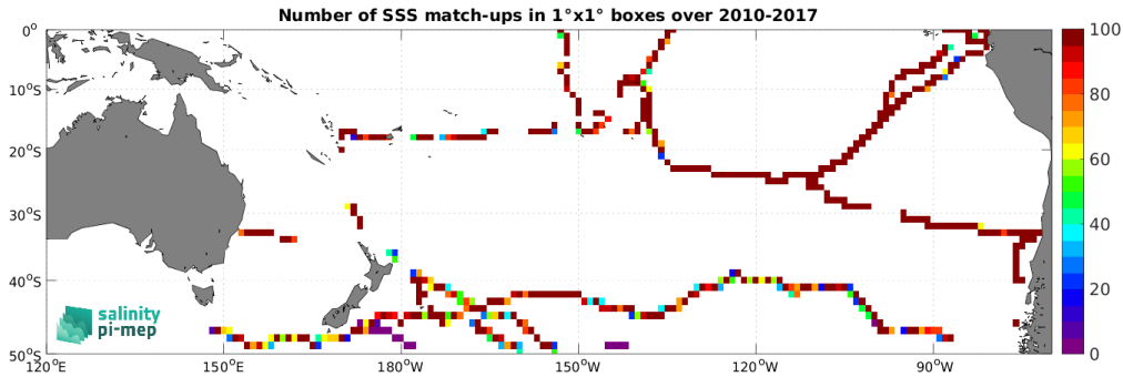
Figure 4: Number of SSS match-ups between TSG (GOSUD-Sailing-ship) SSS and the CCI SSS L4 Merged-OI v3.2 - 30-day running (ESA) SSS product for the South Pacific Ocean Pi-MEP region over 1^\circ \times 1^\circ boxes and for the full satellite product period.
