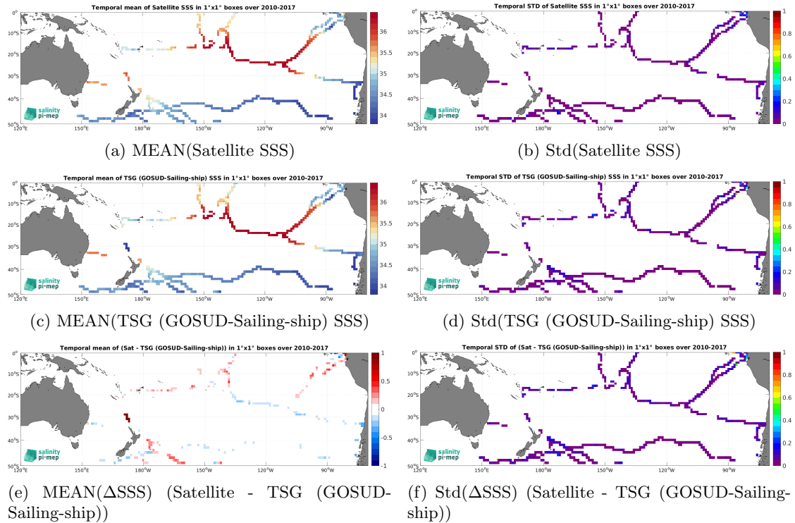
Figure 6: Temporal mean (left) and Std (right) of SSS from CCI SSS L4 Merged-OI v3.2 - 30-day running (ESA) (top), TSG (GOSUD-Sailing-ship) (middle), and of \Delta SSS (Satellite - TSG (GOSUD-Sailing-ship)). Only match-up pairs are used to generate these maps.
