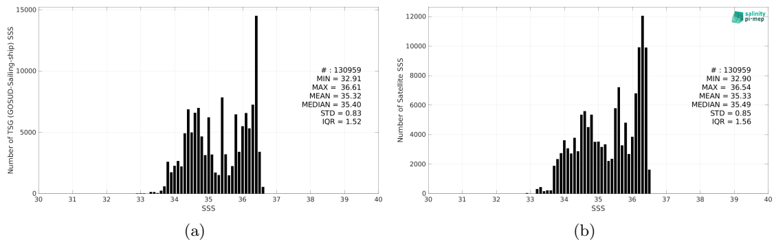
Figure 2: Histograms of SSS from TSG (GOSUD-Sailing-ship) (a) and CCI SSS L4 Merged-OI v3.2 - 30-day running (ESA) (b) considering all match-up pairs per bins of 0.1 over the South Pacific Ocean Pi-MEP region and for the full satellite product period.
